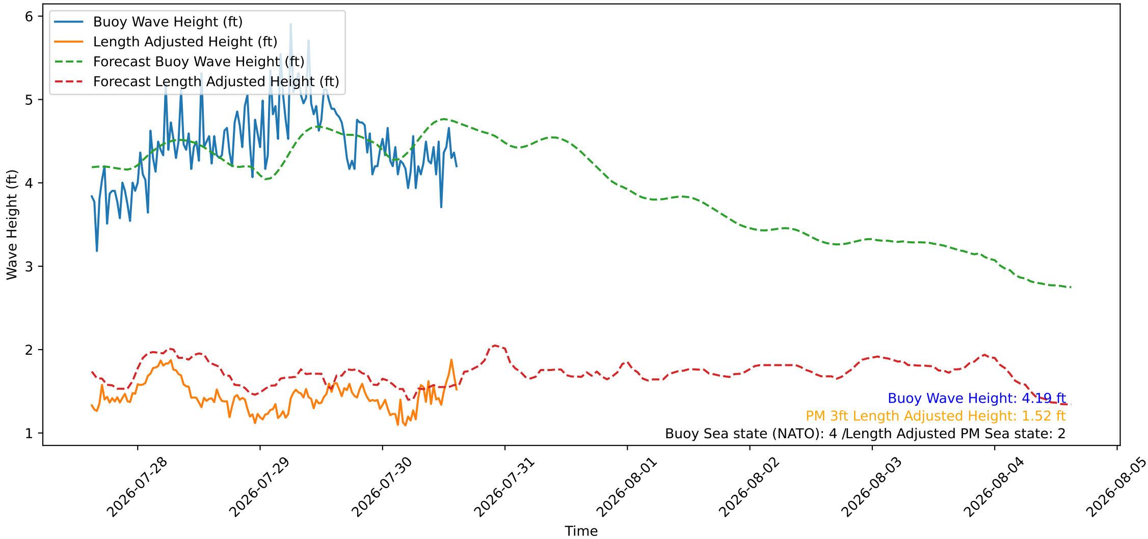
Wave Heights over Time for Oceanside Harbor at 2026-07-30 15:10:27
