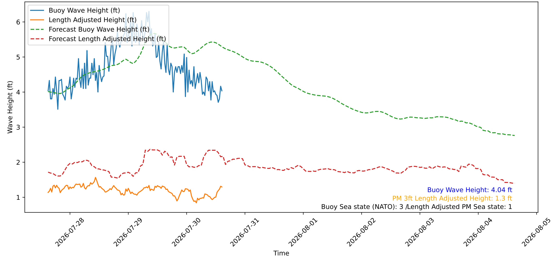
Wave Heights over Time for Green Beach at 2026-07-30 15:11:10
