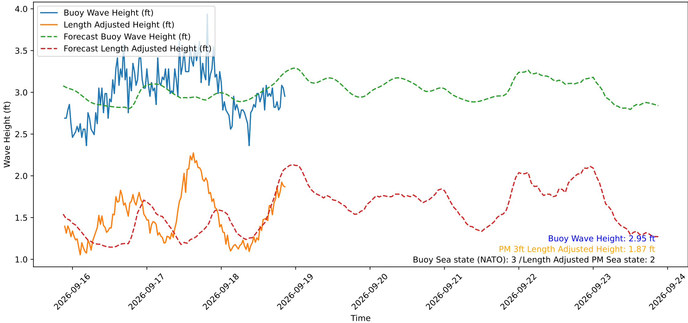
Wave Heights over Time for Oceanside Harbor at 2026-09-18 21:20:30
