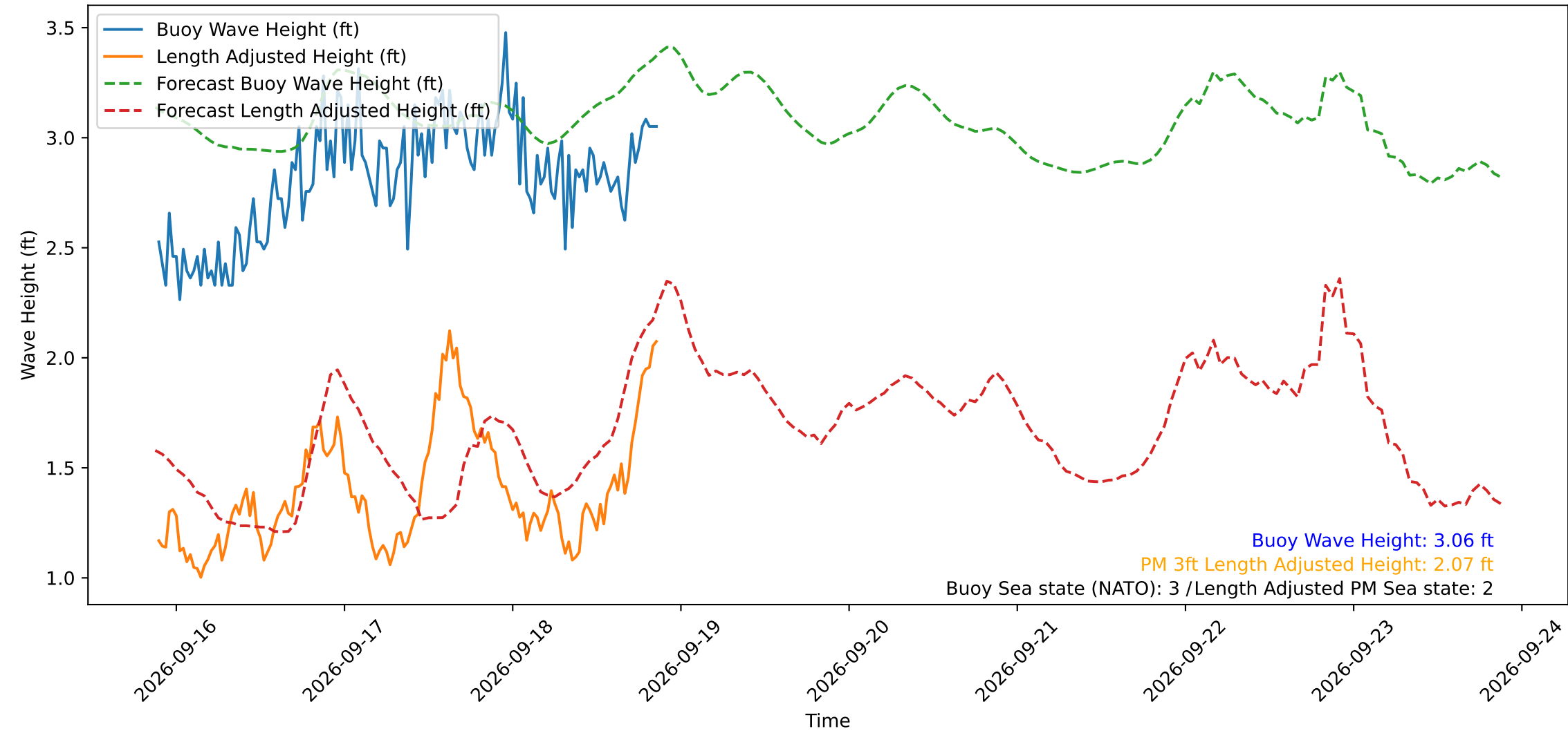
Wave Heights over Time for Green Beach at 2026-09-18 21:21:14
