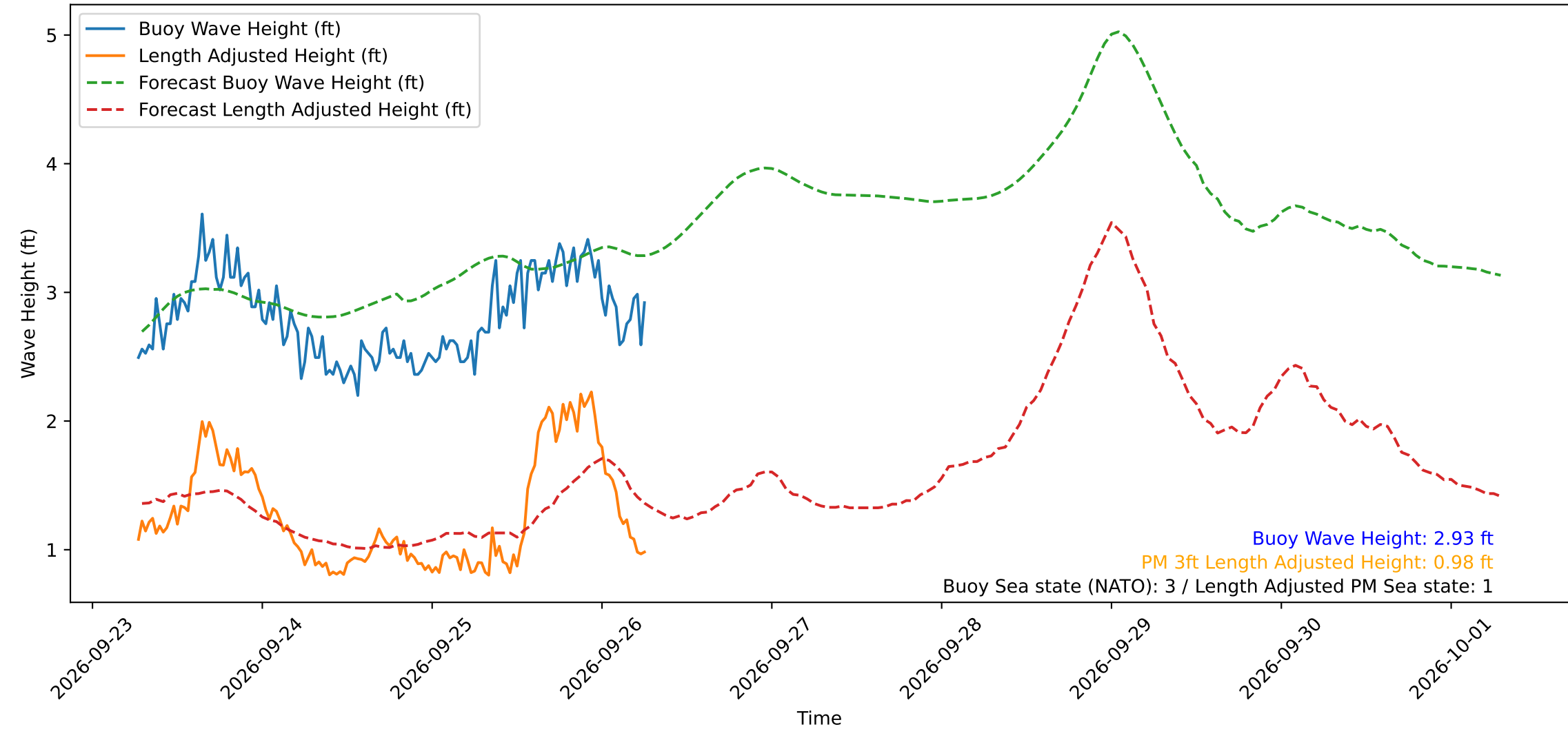
Wave Heights over Time for Oceanside Harbor at 2026-09-26 06:30:29
