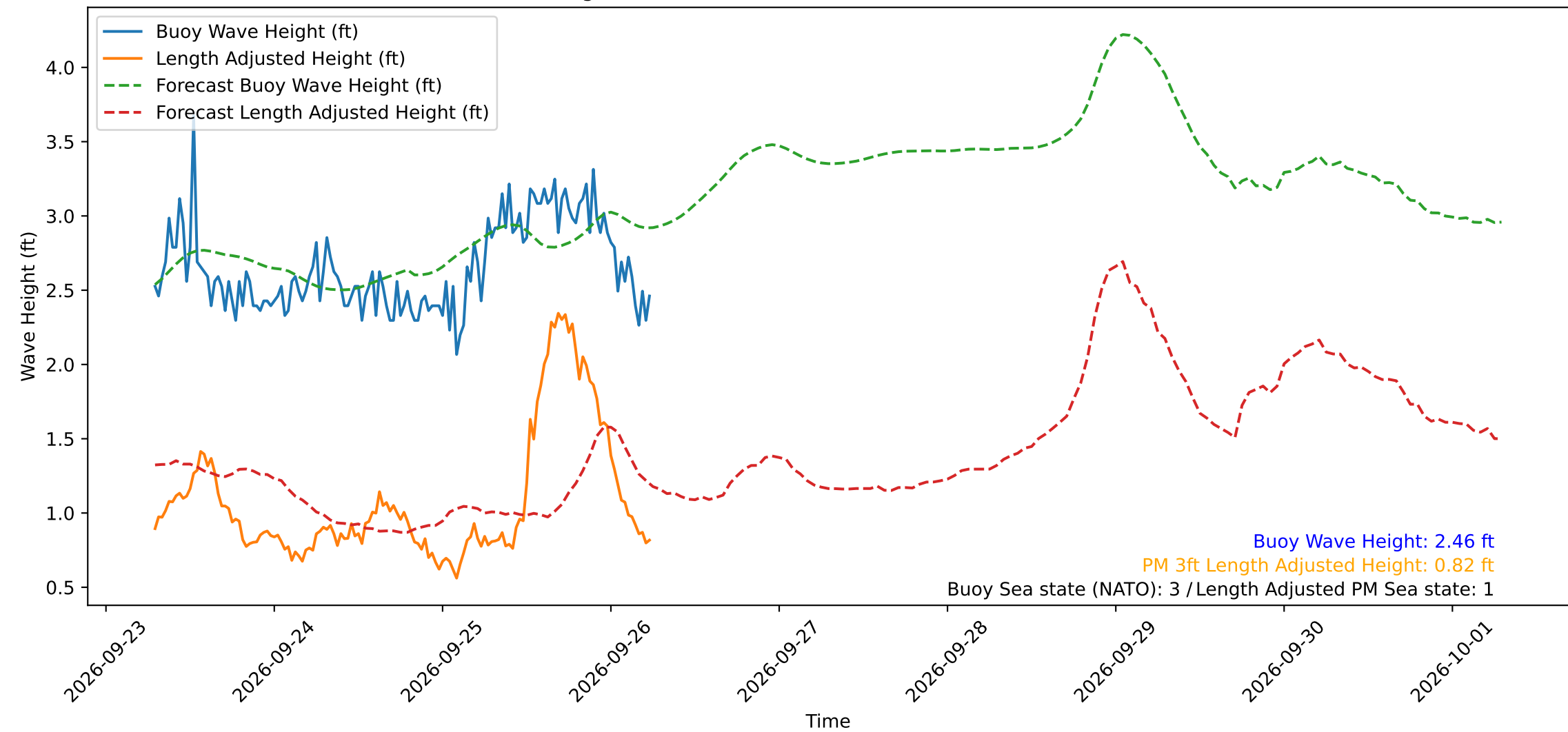
Wave Heights over Time for Red Beach at 2026-09-26 06:30:49
