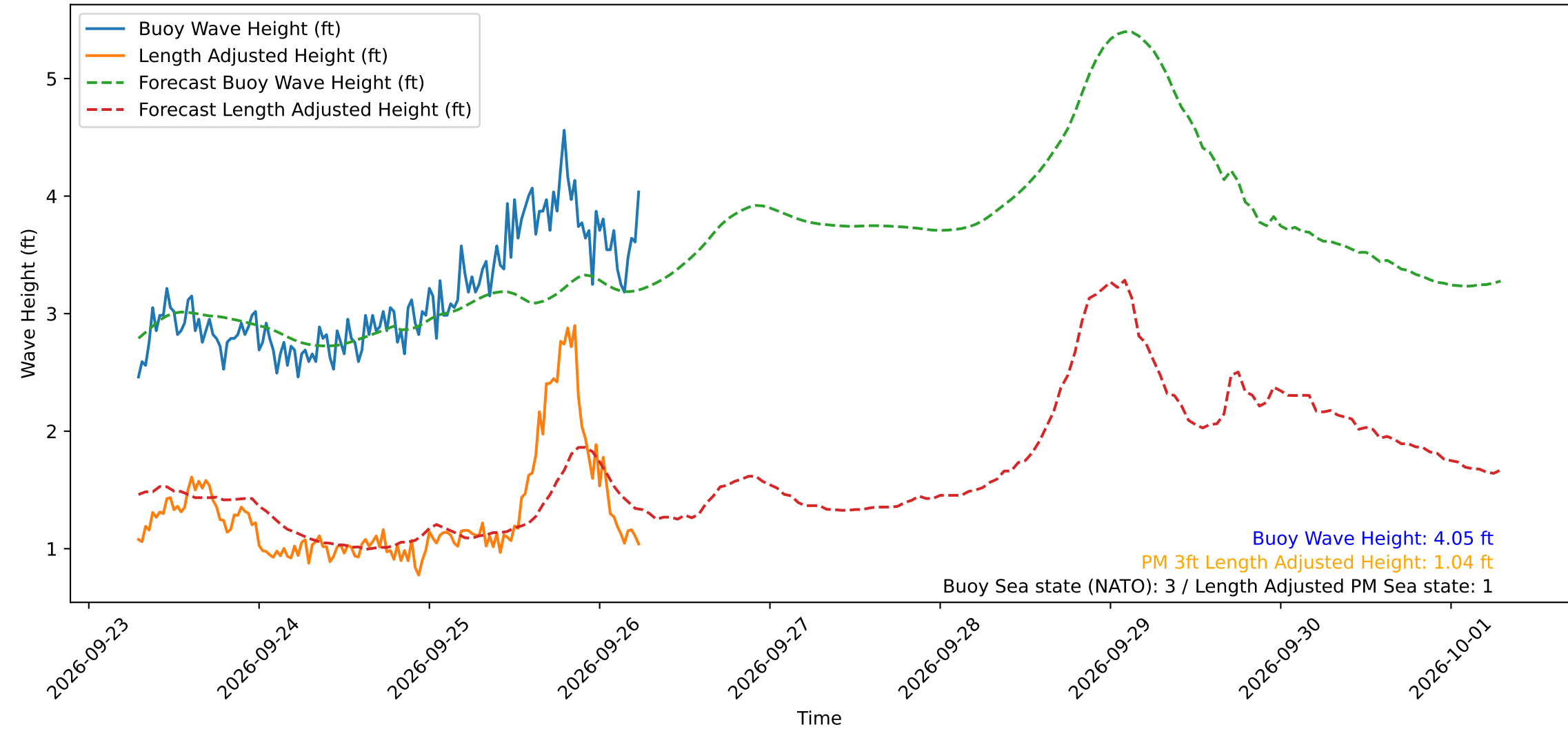
Wave Heights over Time for Green Beach at 2026-09-26 06:31:12
