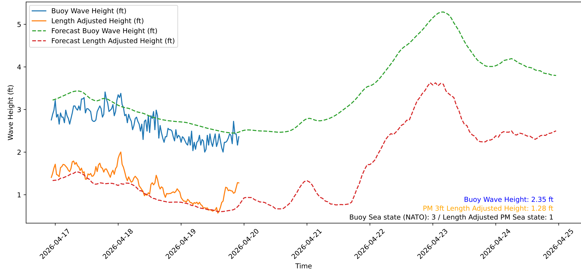
Wave Heights over Time for Oceanside Harbor at 2026-04-19 22:40:32
