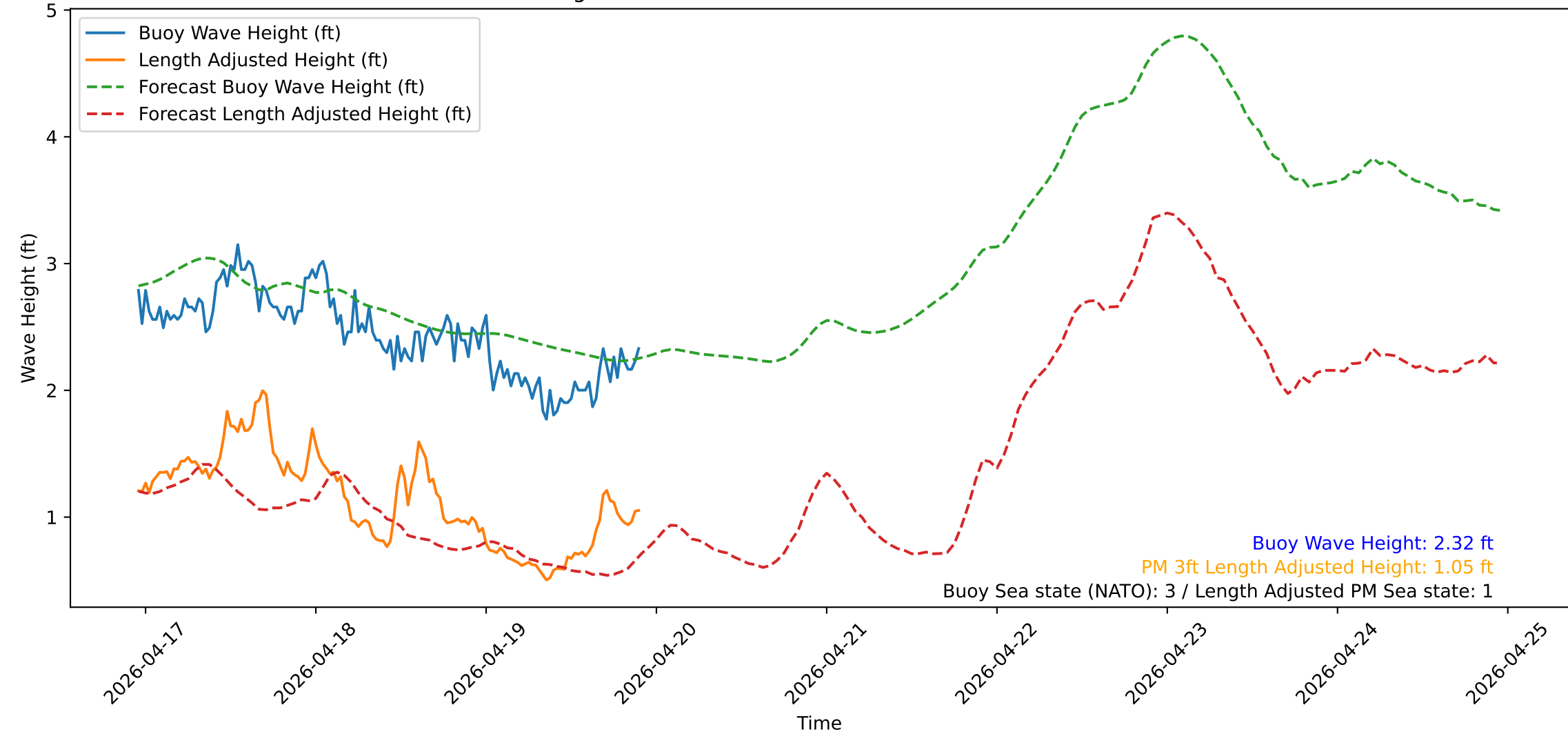
Wave Heights over Time for Red Beach at 2026-04-19 22:40:52
