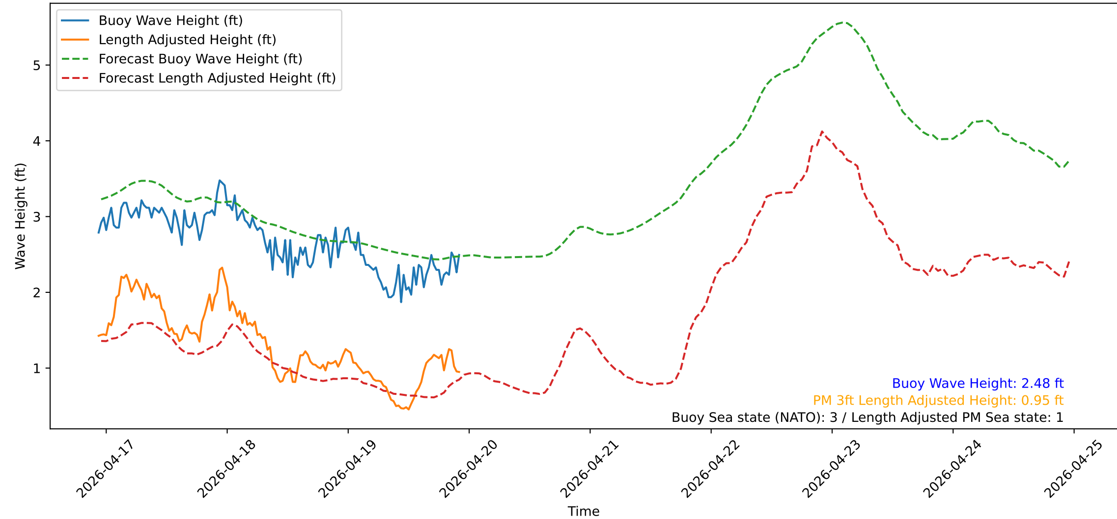
Wave Heights over Time for Green Beach at 2026-04-19 22:41:14
