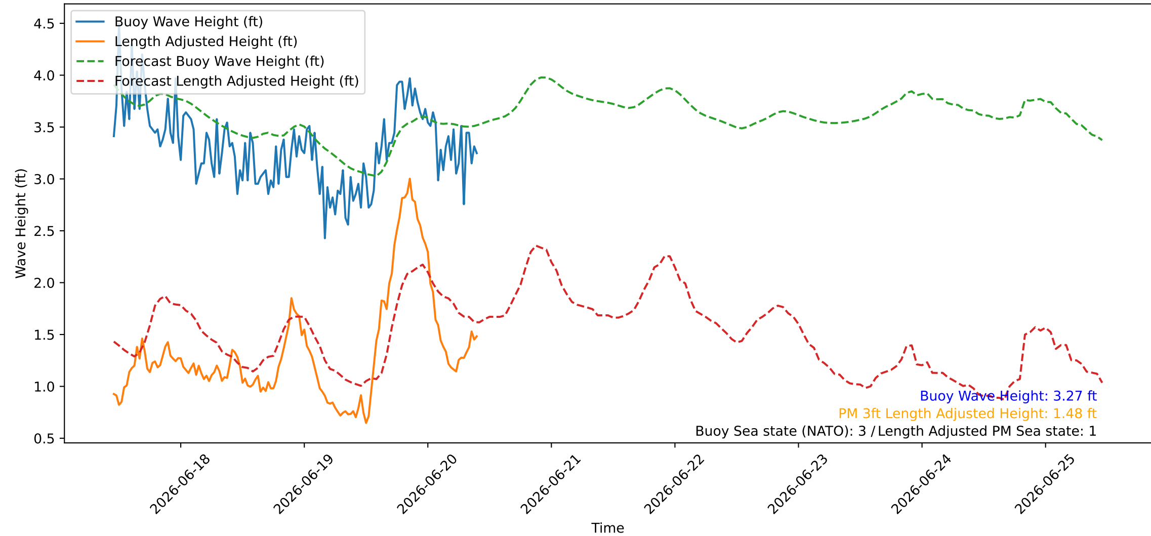
Wave Heights over Time for Green Beach at 2026-06-20 11:01:07
