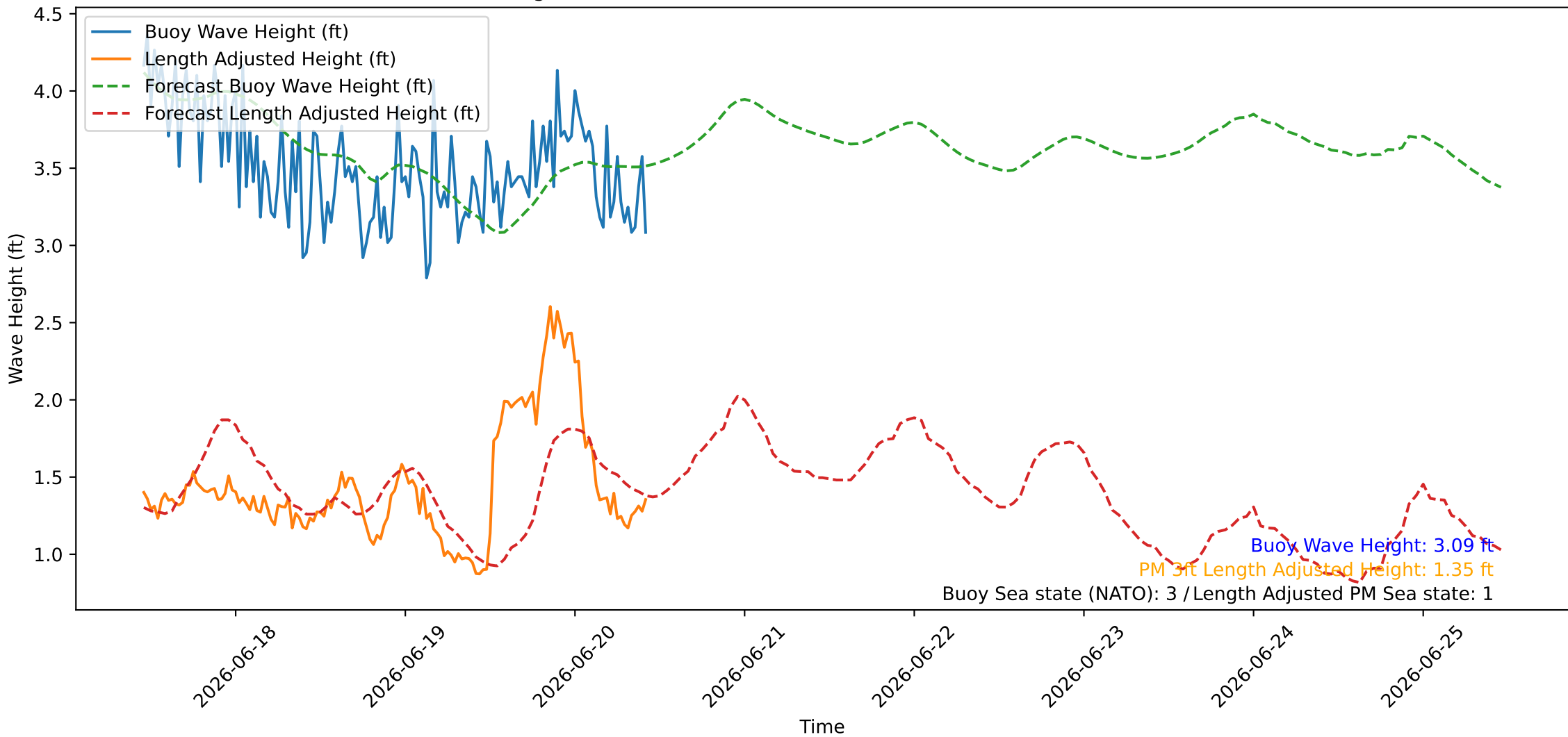
Wave Heights over Time for Oceanside Harbor at 2026-06-20 11:00:26
