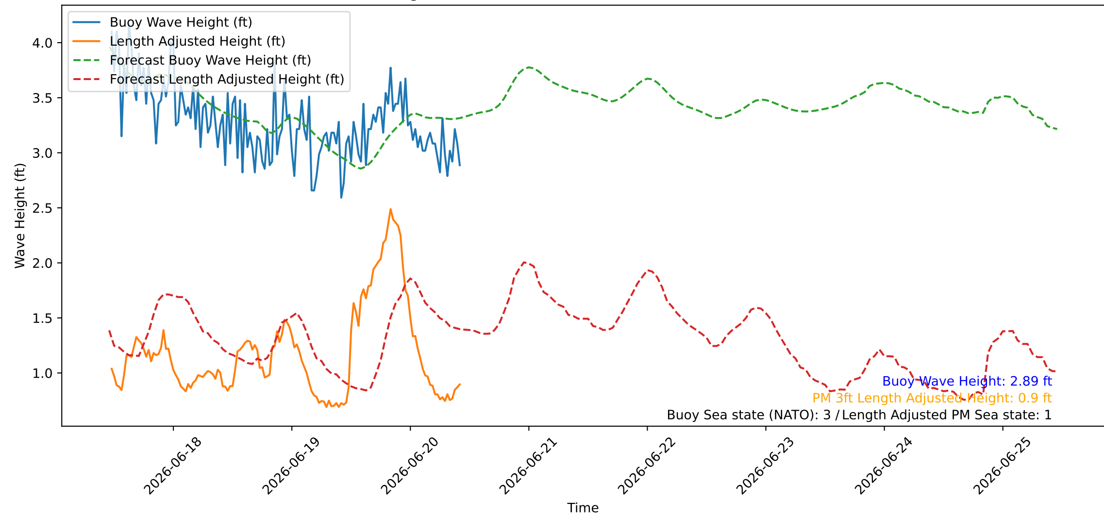
Wave Heights over Time for Red Beach at 2026-06-20 11:00:45
