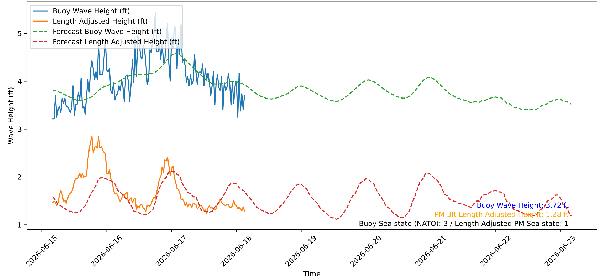
Wave Heights over Time for Oceanside Harbor at 2026-06-18 03:50:26
