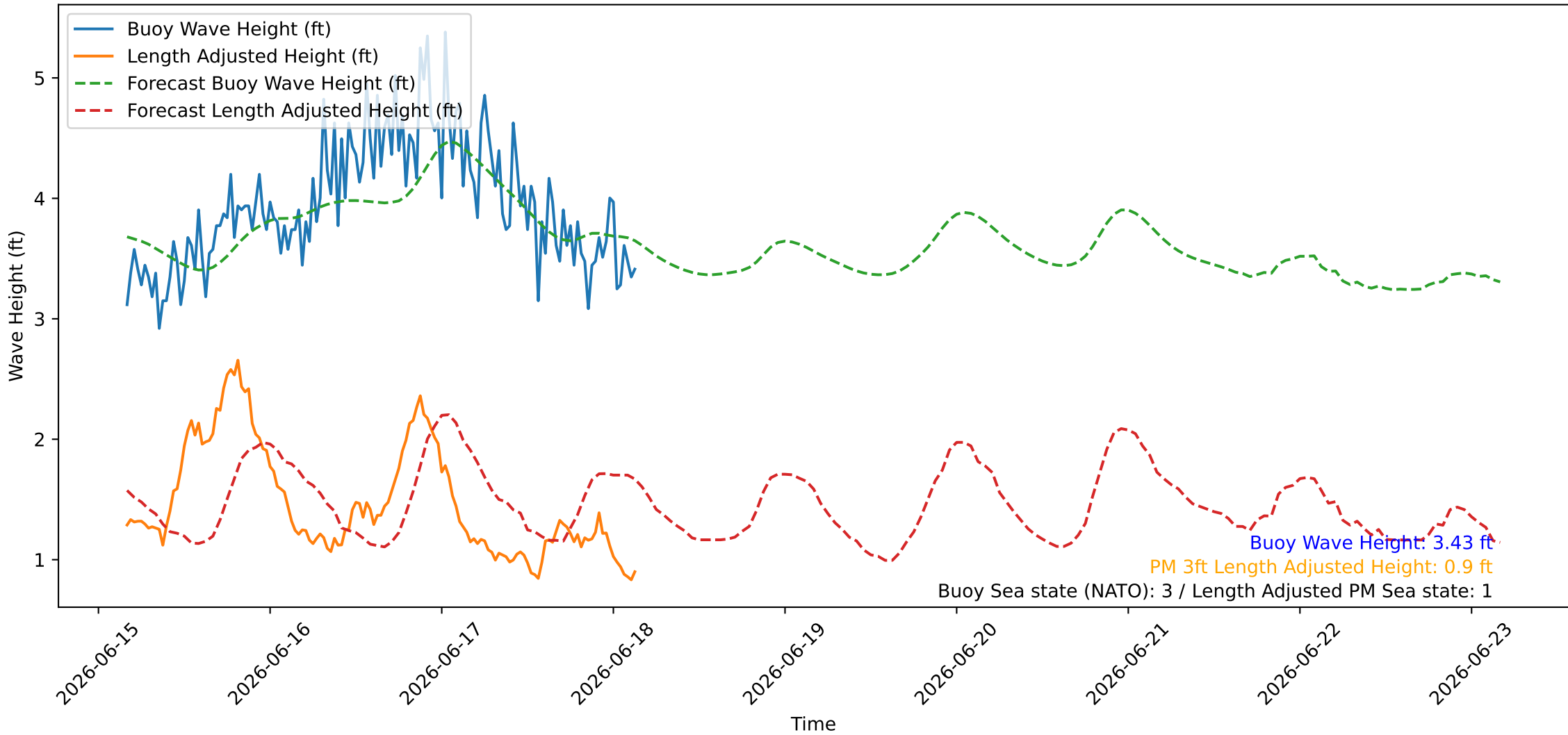
Wave Heights over Time for Red Beach at 2026-06-18 03:50:47
