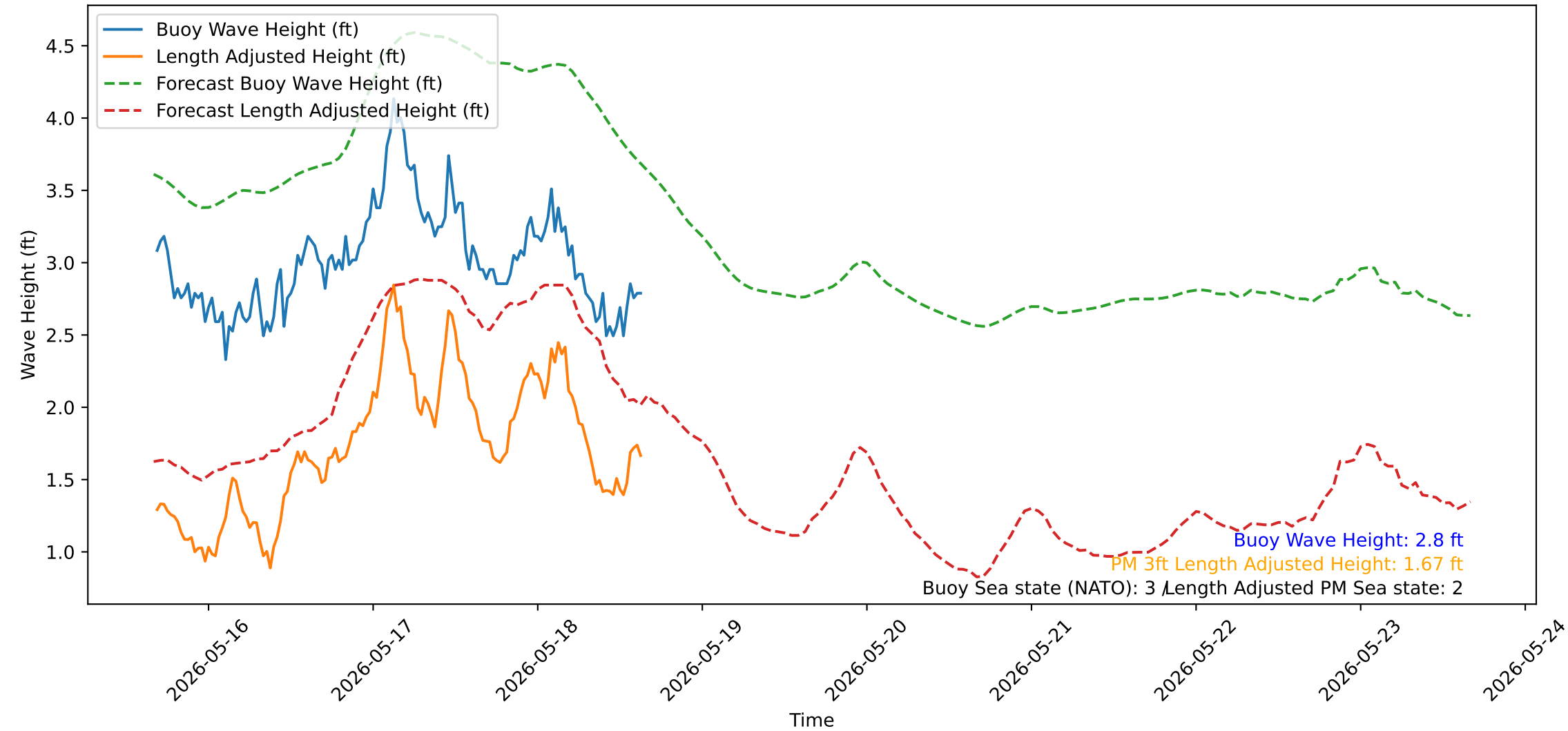
Wave Heights over Time for Red Beach at 2026-05-18 16:00:51
