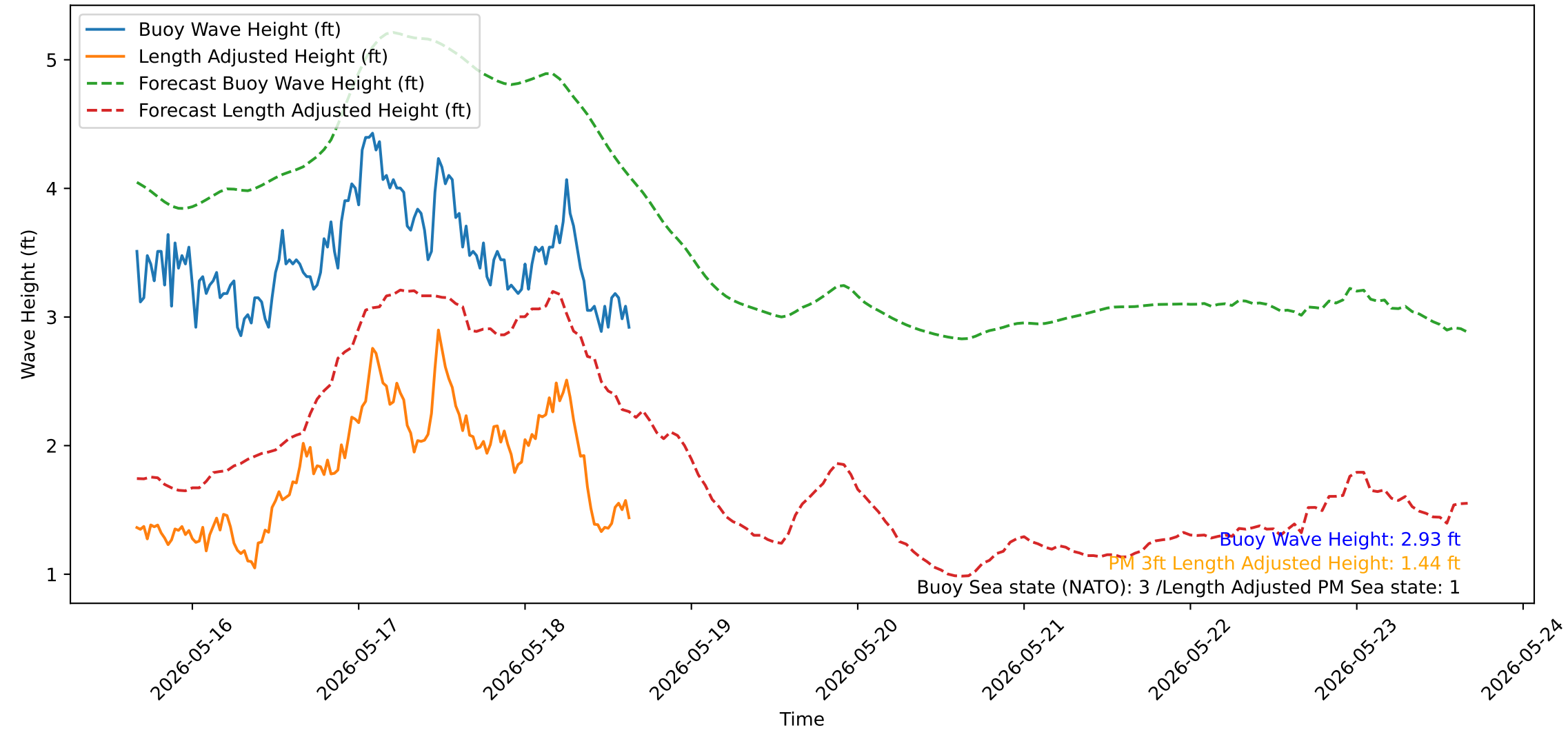
Wave Heights over Time for Green Beach at 2026-05-18 16:01:13
