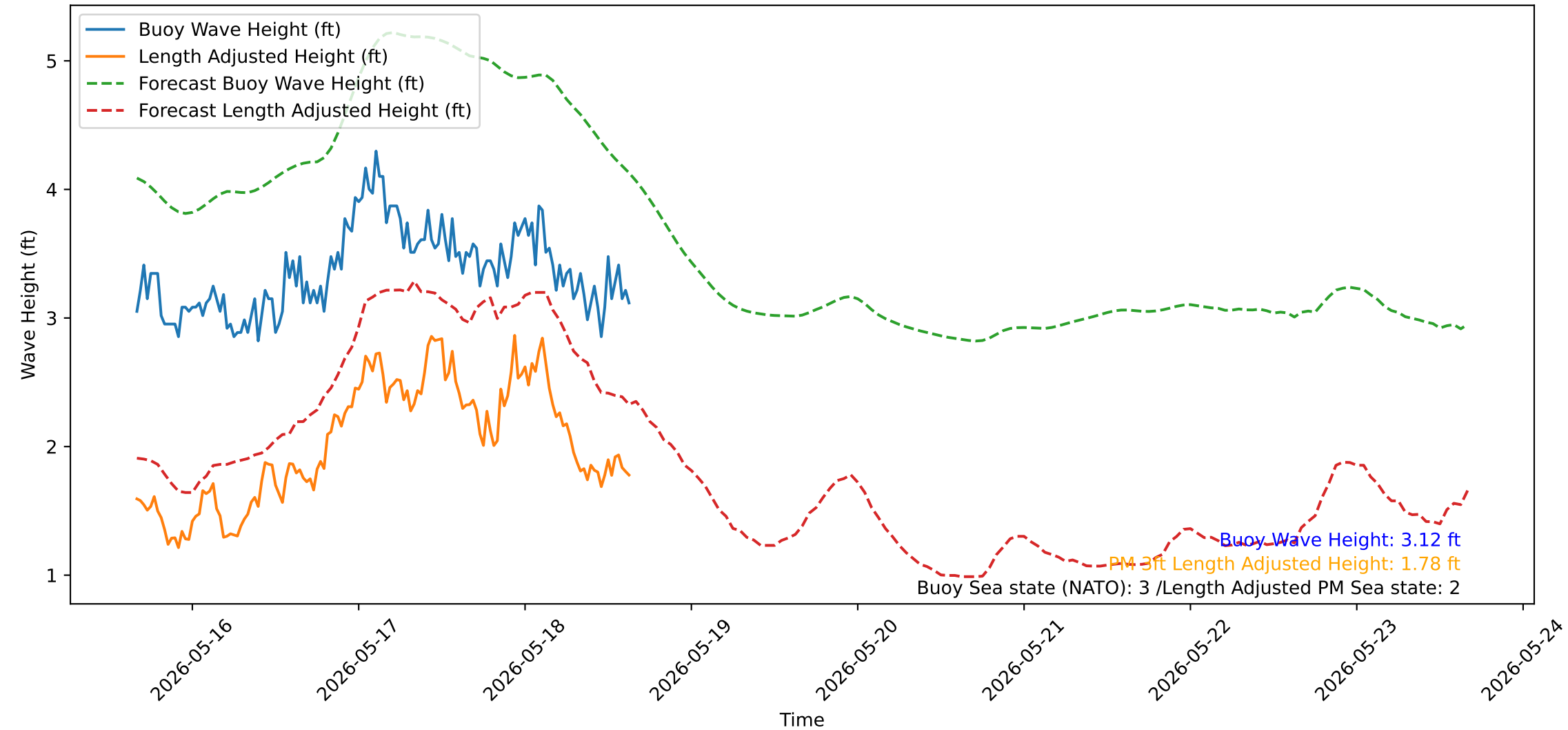
Wave Heights over Time for Oceanside Harbor at 2026-05-18 16:00:31
