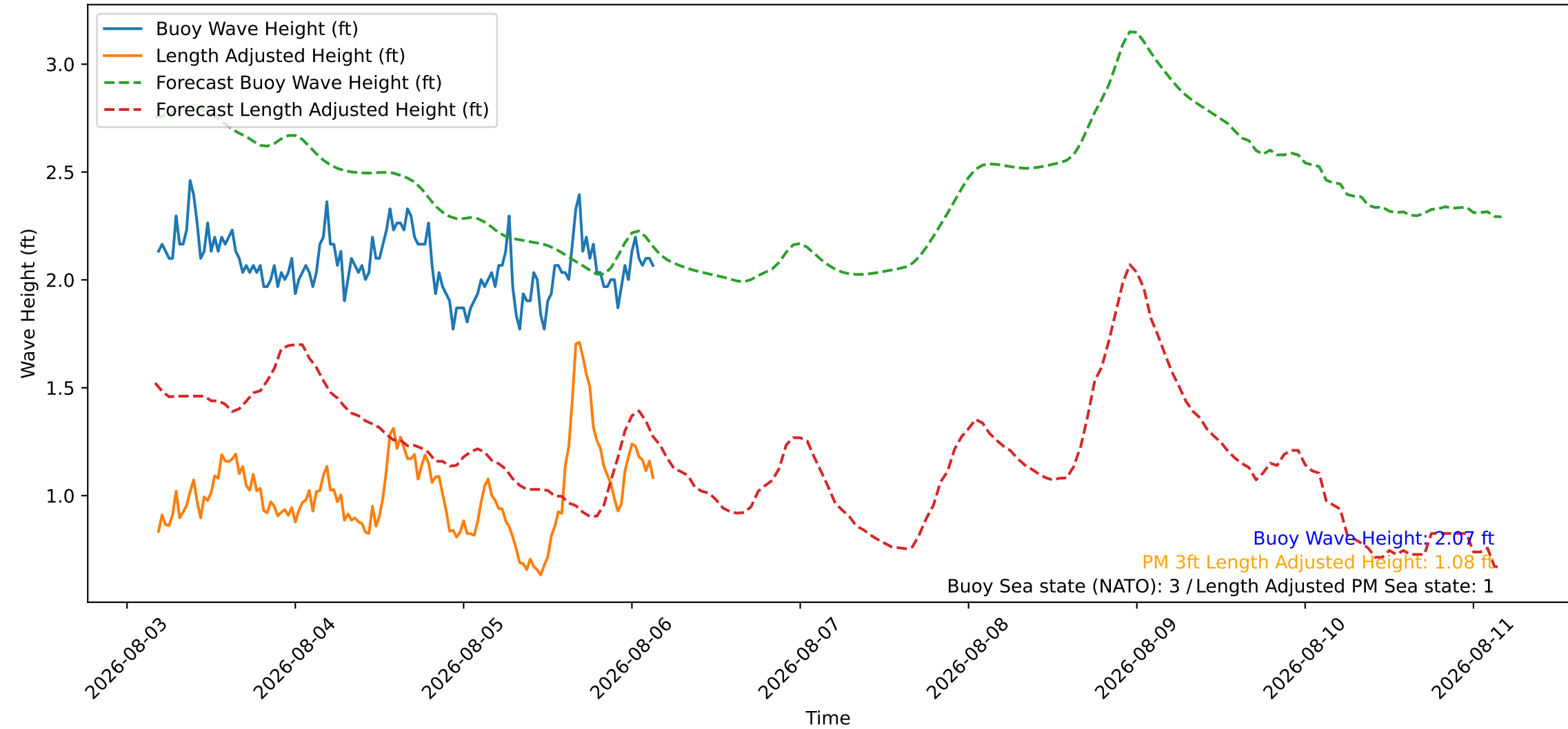
Wave Heights over Time for Red Beach at 2026-08-06 04:11:10
