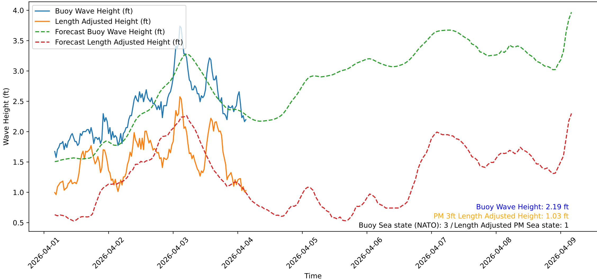
Wave Heights over Time for Red Beach at 2026-04-04 03:40:47
