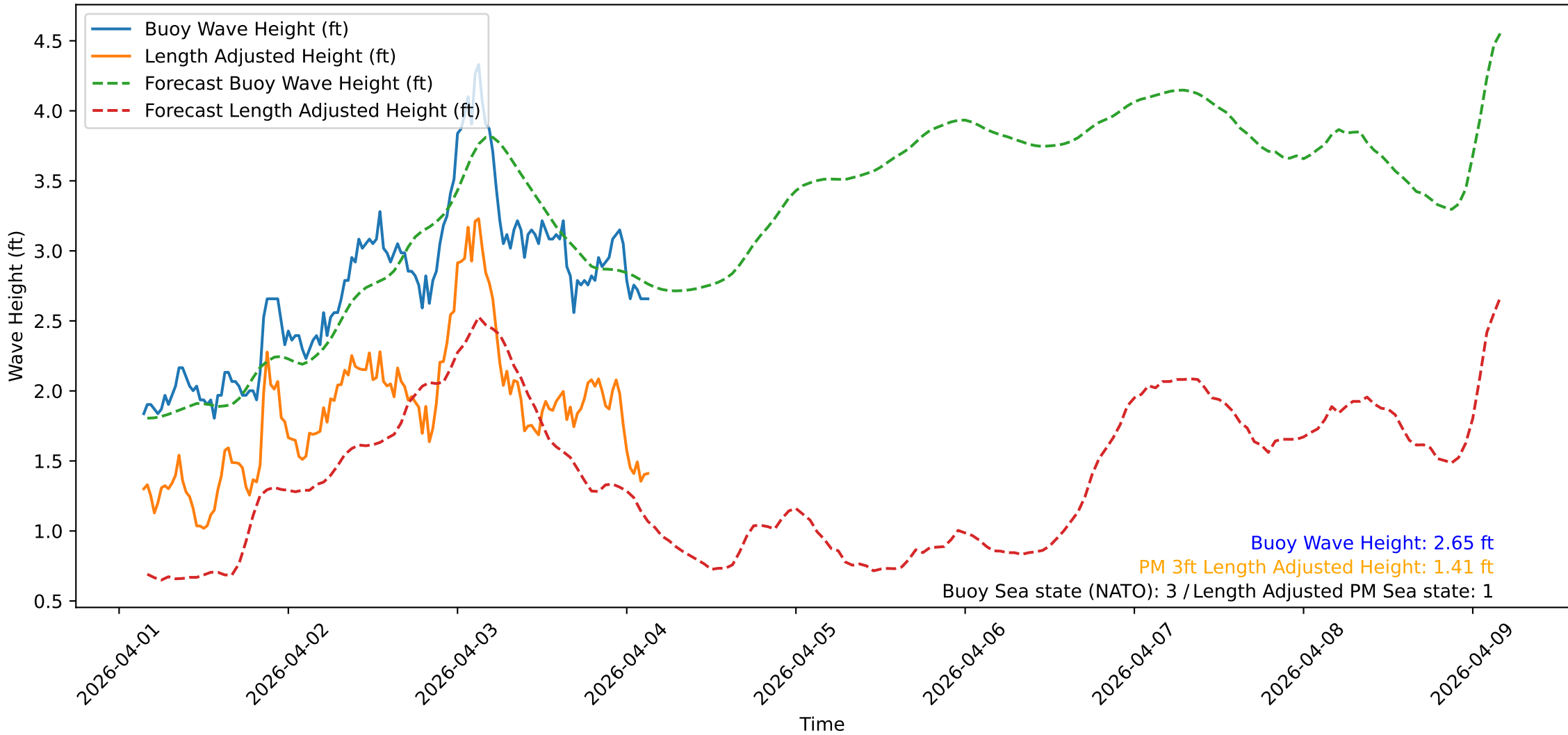
Wave Heights over Time for Green Beach at 2026-04-04 03:41:10
