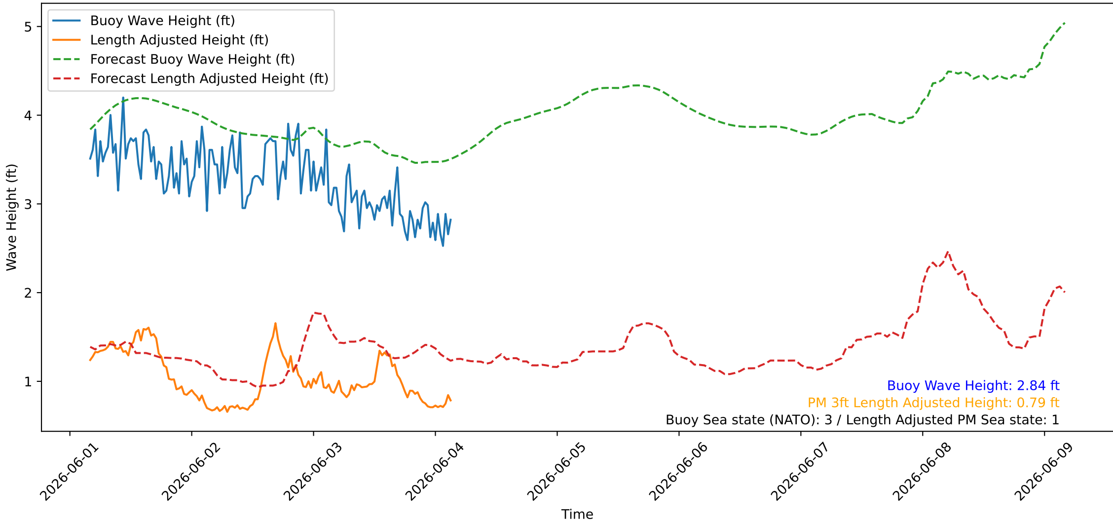
Wave Heights over Time for Red Beach at 2026-06-04 03:50:46
