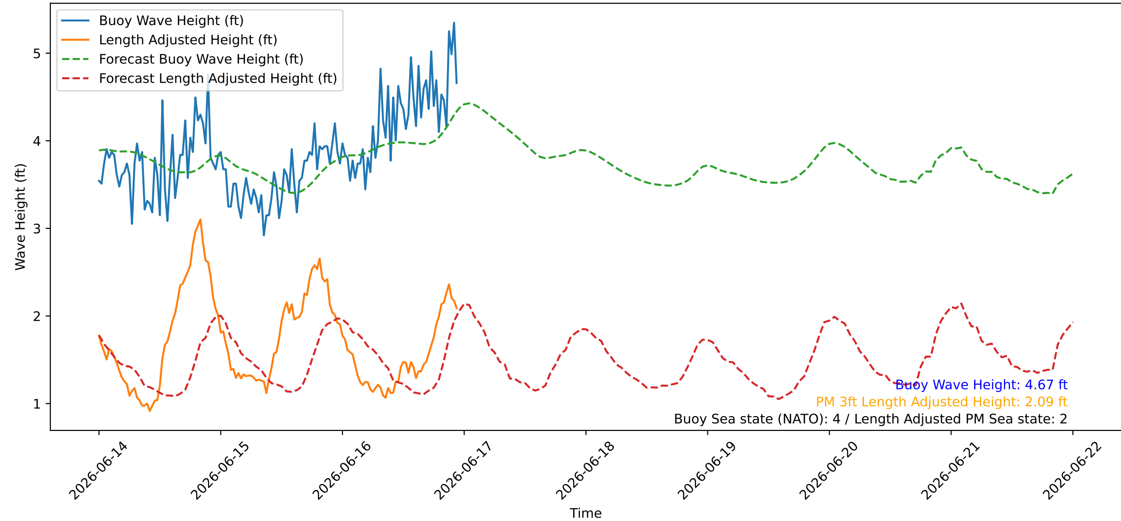
Wave Heights over Time for Red Beach at 2026-06-16 23:30:46
