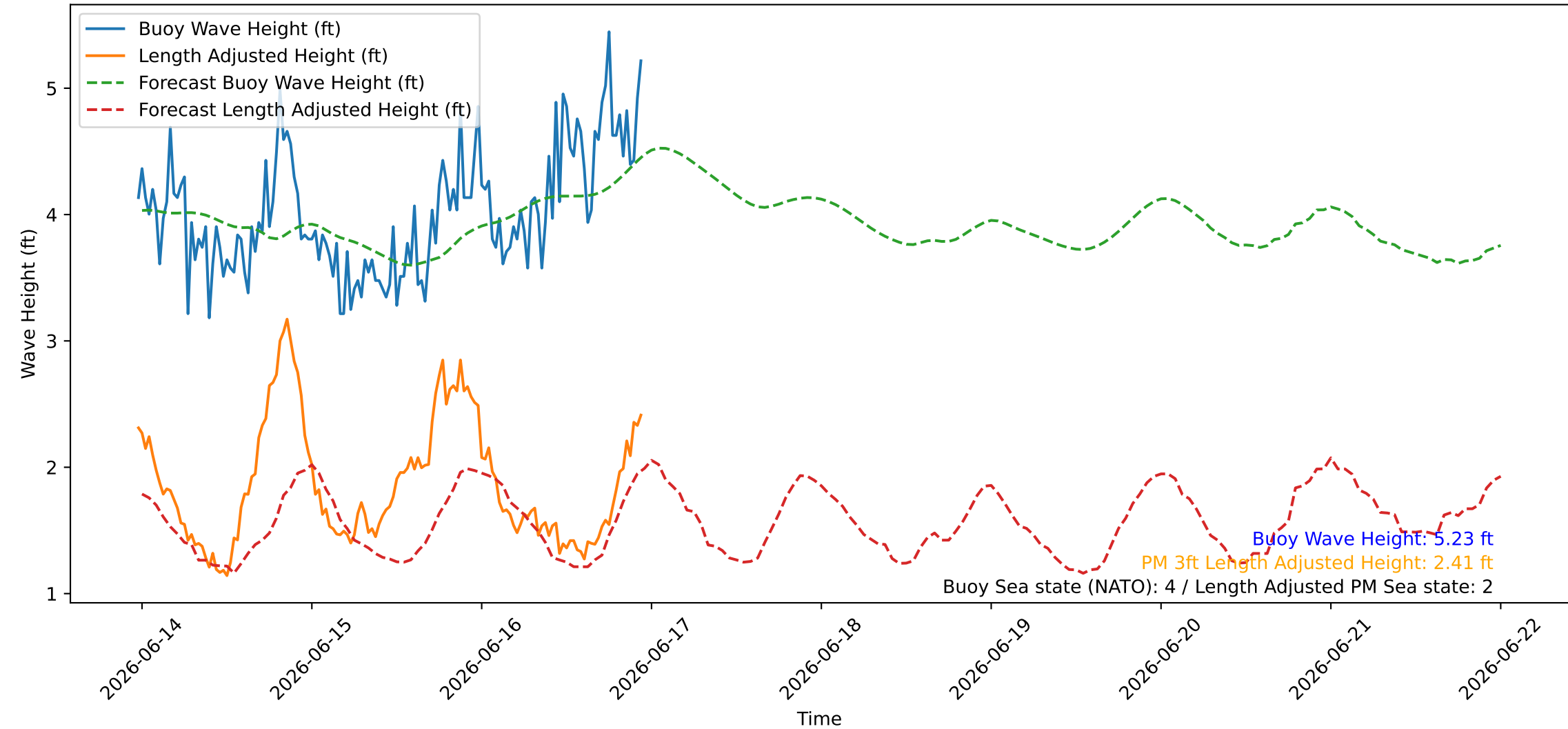
Wave Heights over Time for Oceanside Harbor at 2026-06-16 23:30:26
