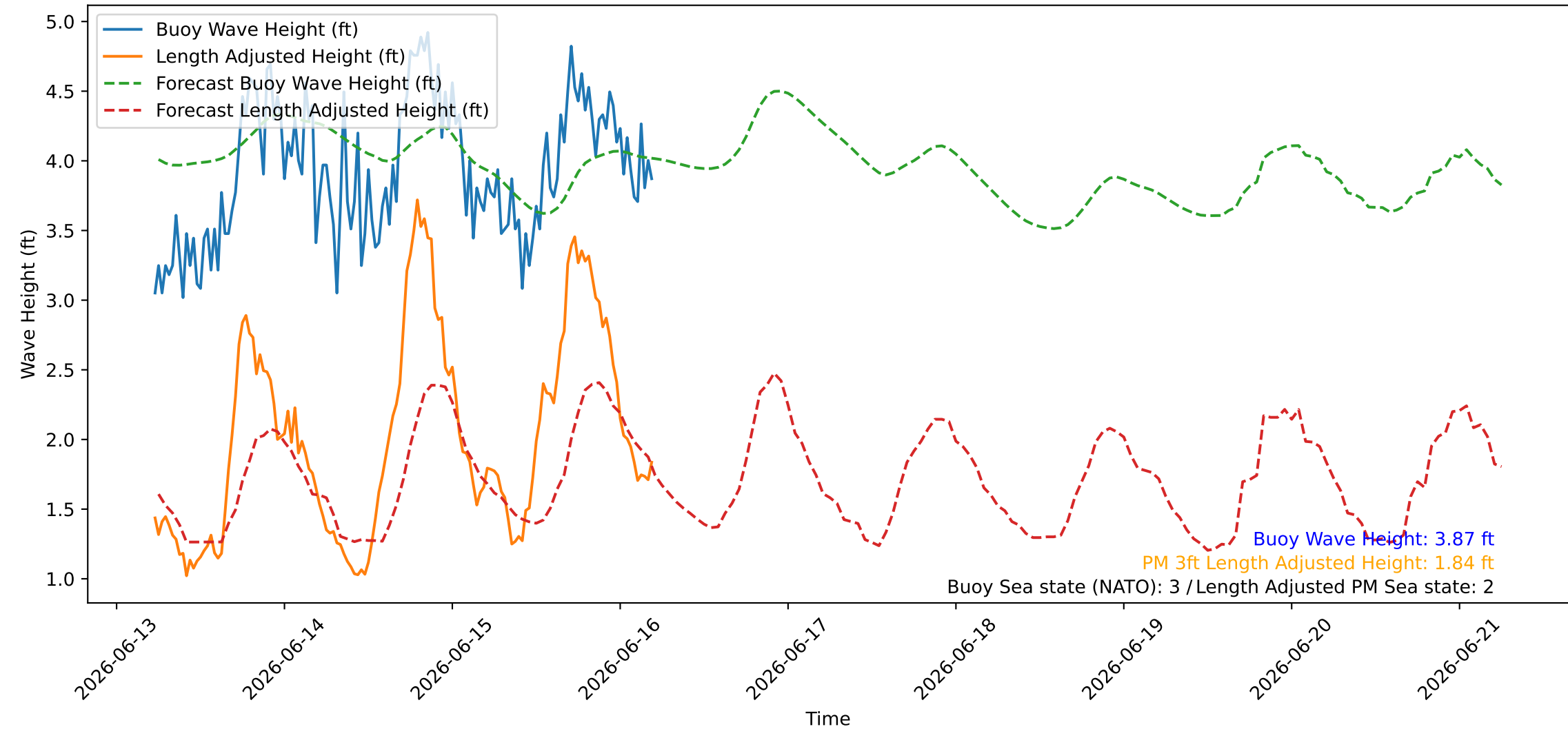
Wave Heights over Time for Green Beach at 2026-06-16 05:31:07
