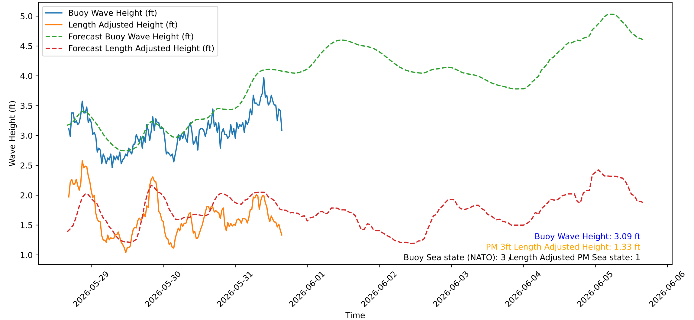
Wave Heights over Time for Green Beach at 2026-05-31 16:21:08
