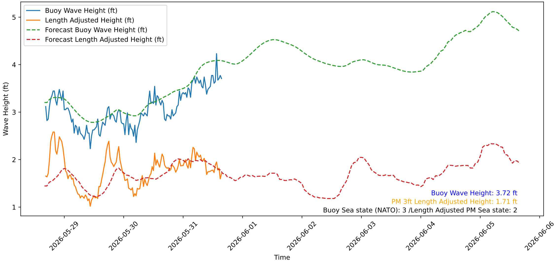
Wave Heights over Time for Oceanside Harbor at 2026-05-31 16:20:26
