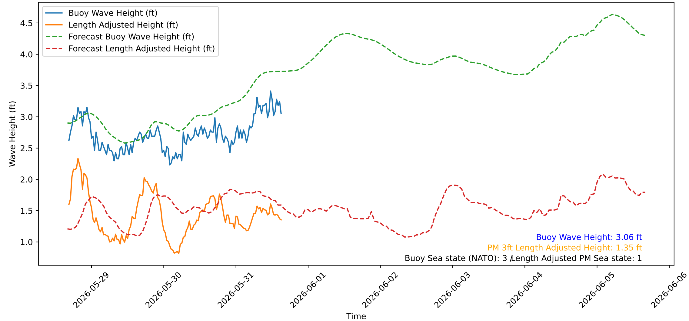
Wave Heights over Time for Red Beach at 2026-05-31 16:20:46
