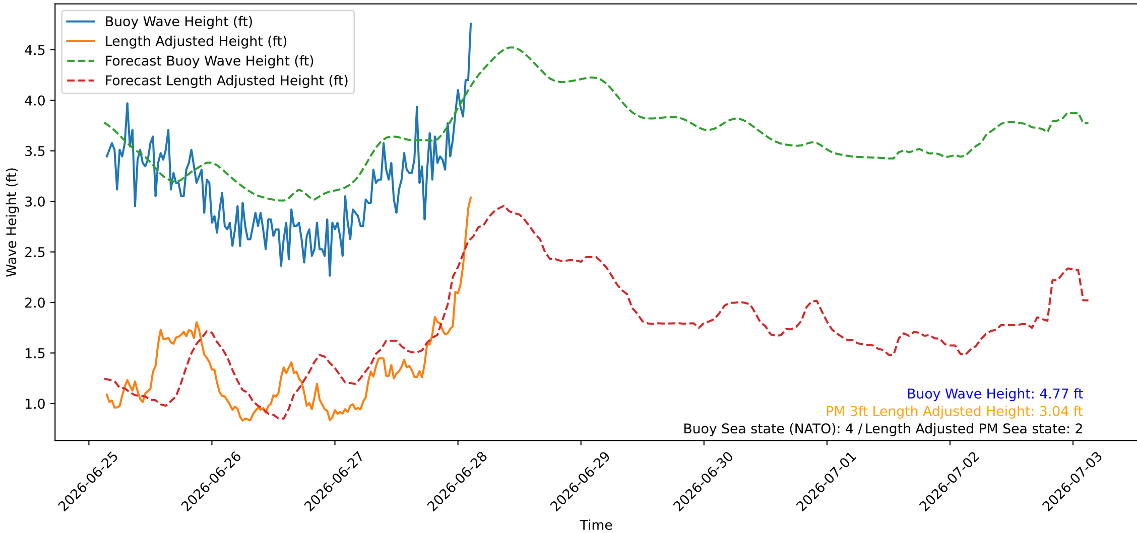
Wave Heights over Time for Green Beach at 2026-06-28 03:21:09
