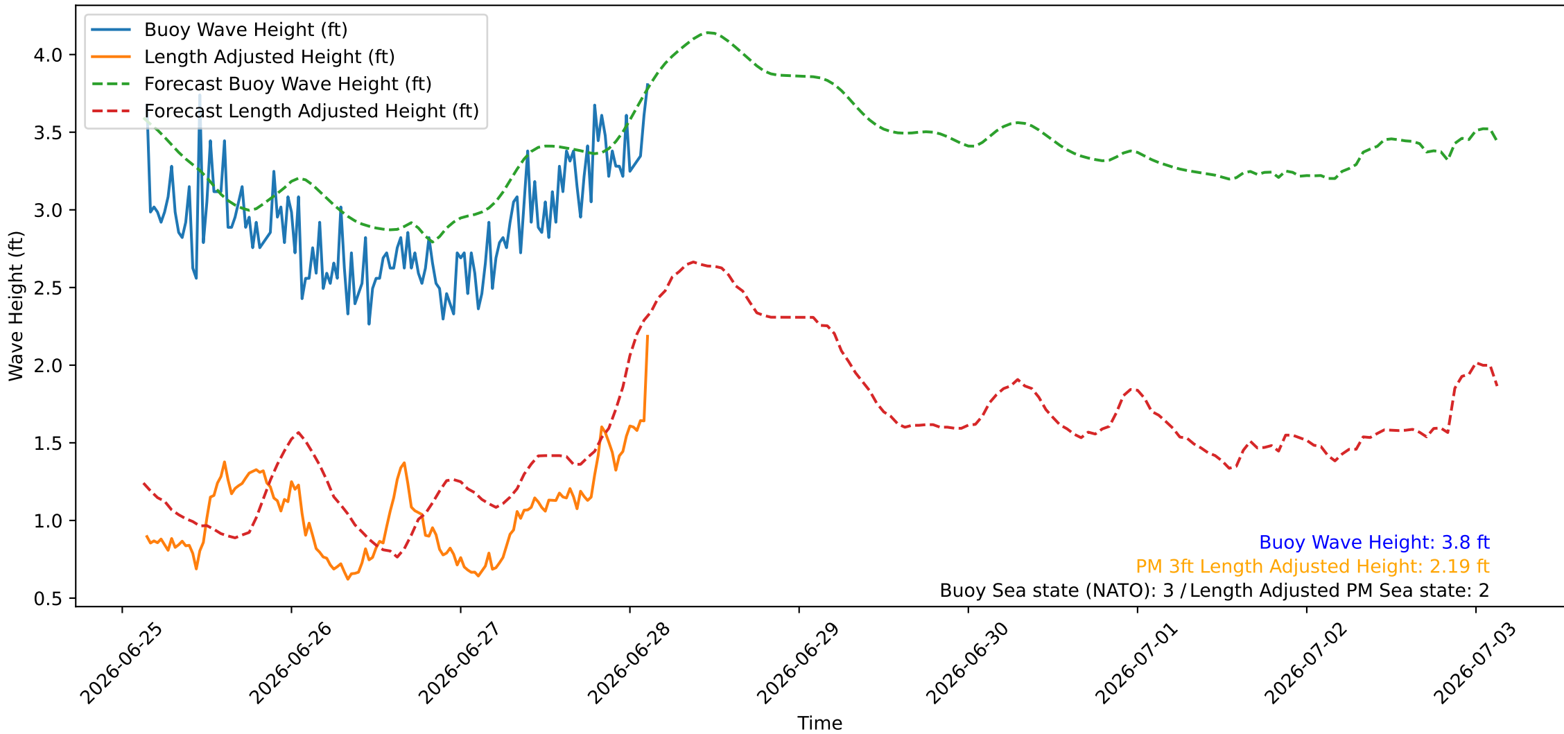
Wave Heights over Time for Red Beach at 2026-06-28 03:20:47
