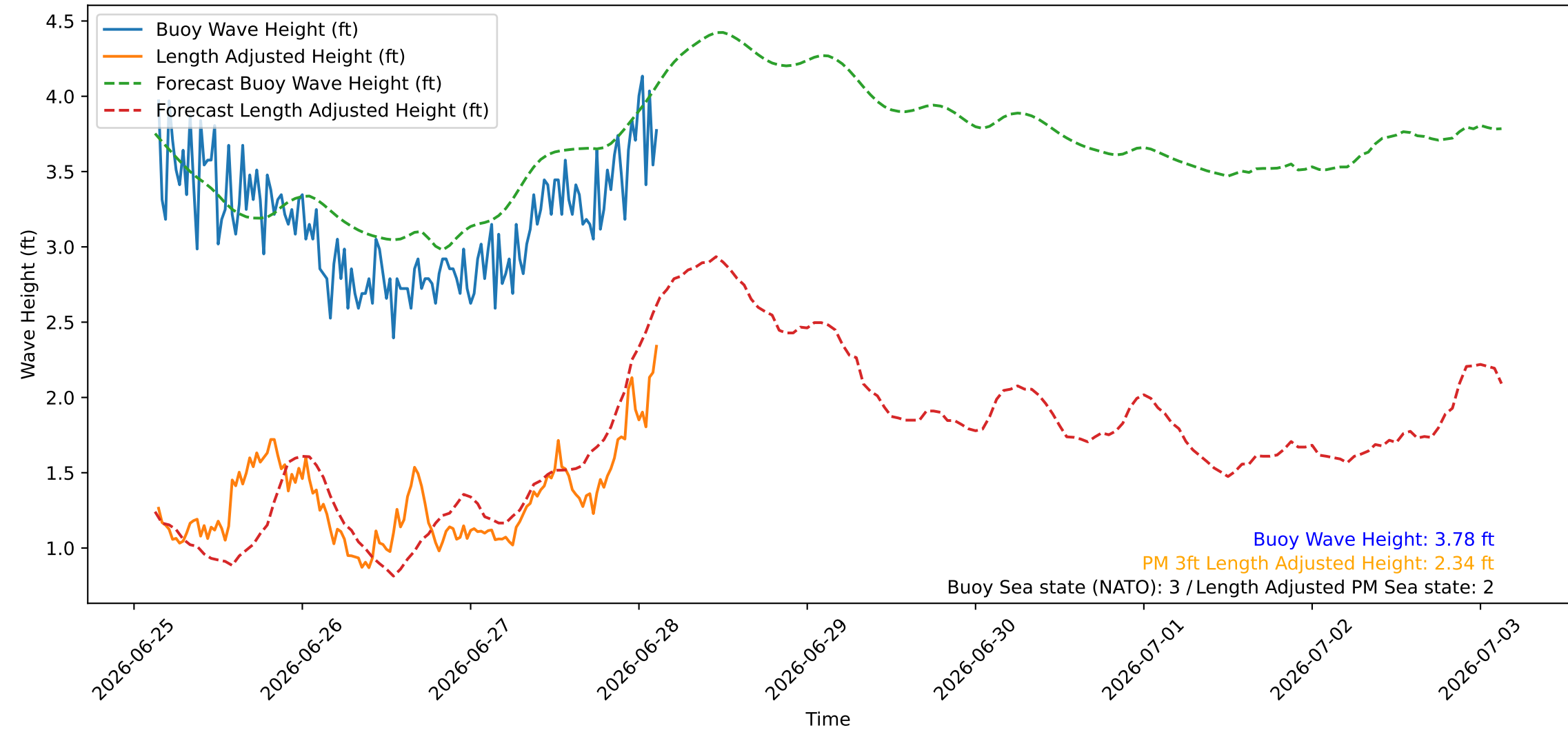
Wave Heights over Time for Oceanside Harbor at 2026-06-28 03:20:26
