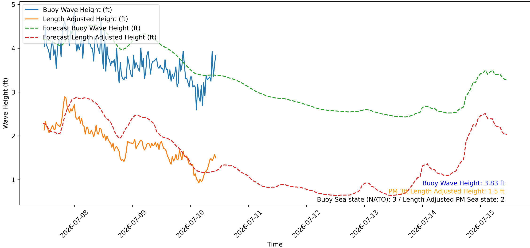
Wave Heights over Time for Red Beach at 2026-07-10 11:10:46
