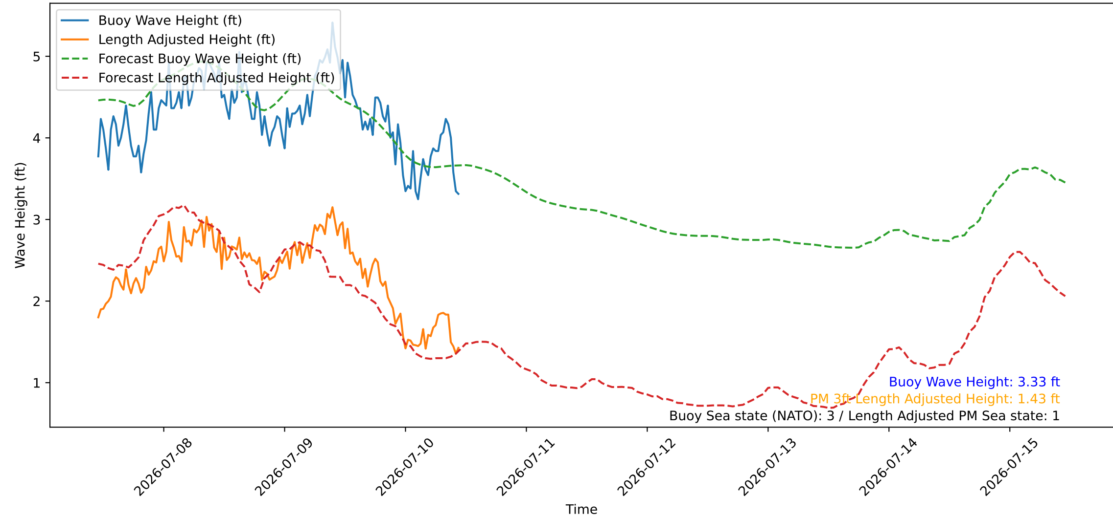
Wave Heights over Time for Oceanside Harbor at 2026-07-10 11:10:26
