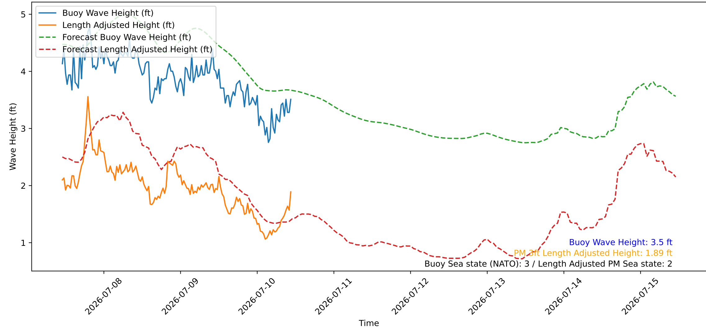
Wave Heights over Time for Green Beach at 2026-07-10 11:11:08
