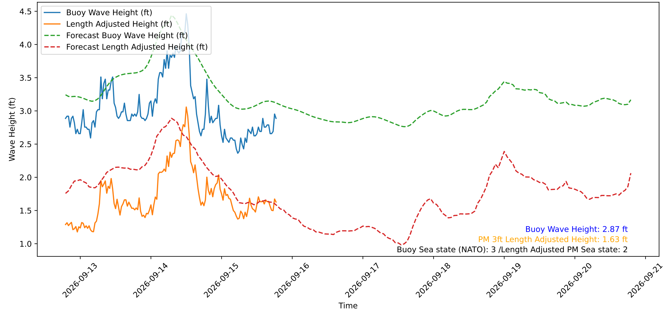
Wave Heights over Time for Oceanside Harbor at 2026-09-15 19:10:29
