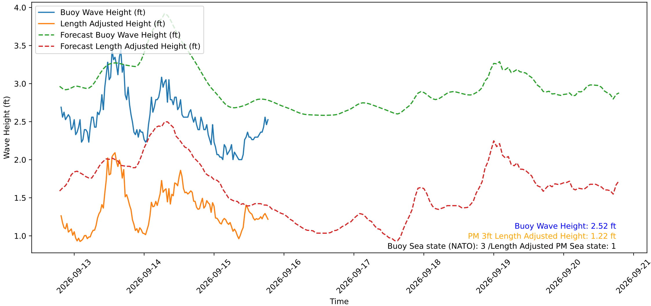
Wave Heights over Time for Red Beach at 2026-09-15 19:10:49
