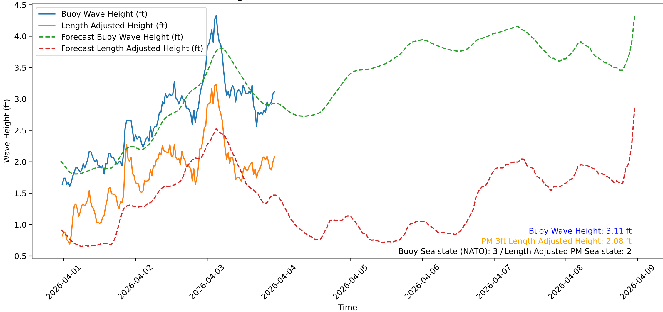
Wave Heights over Time for Green Beach at 2026-04-03 23:21:18
