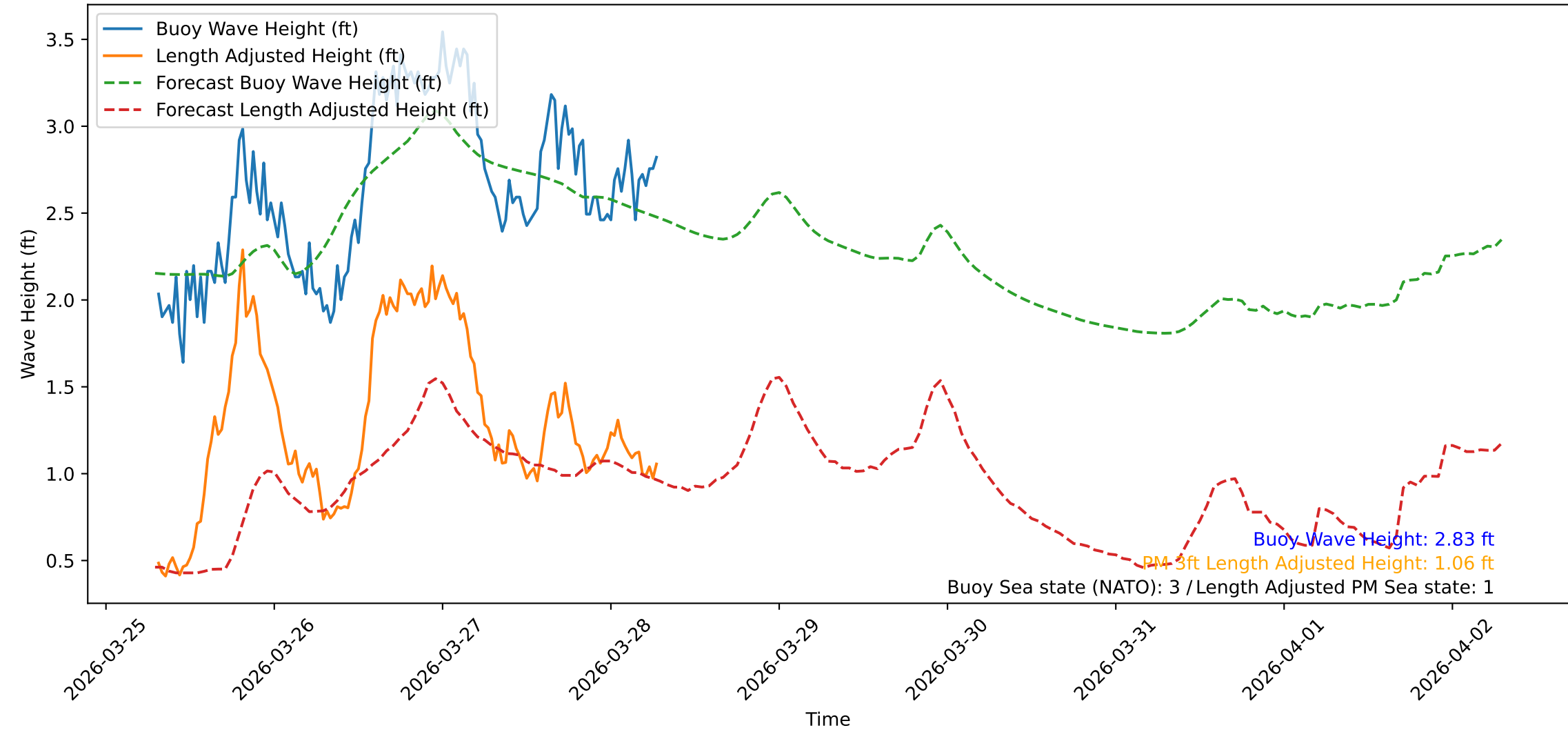
Wave Heights over Time for Green Beach at 2026-03-28 07:21:09
