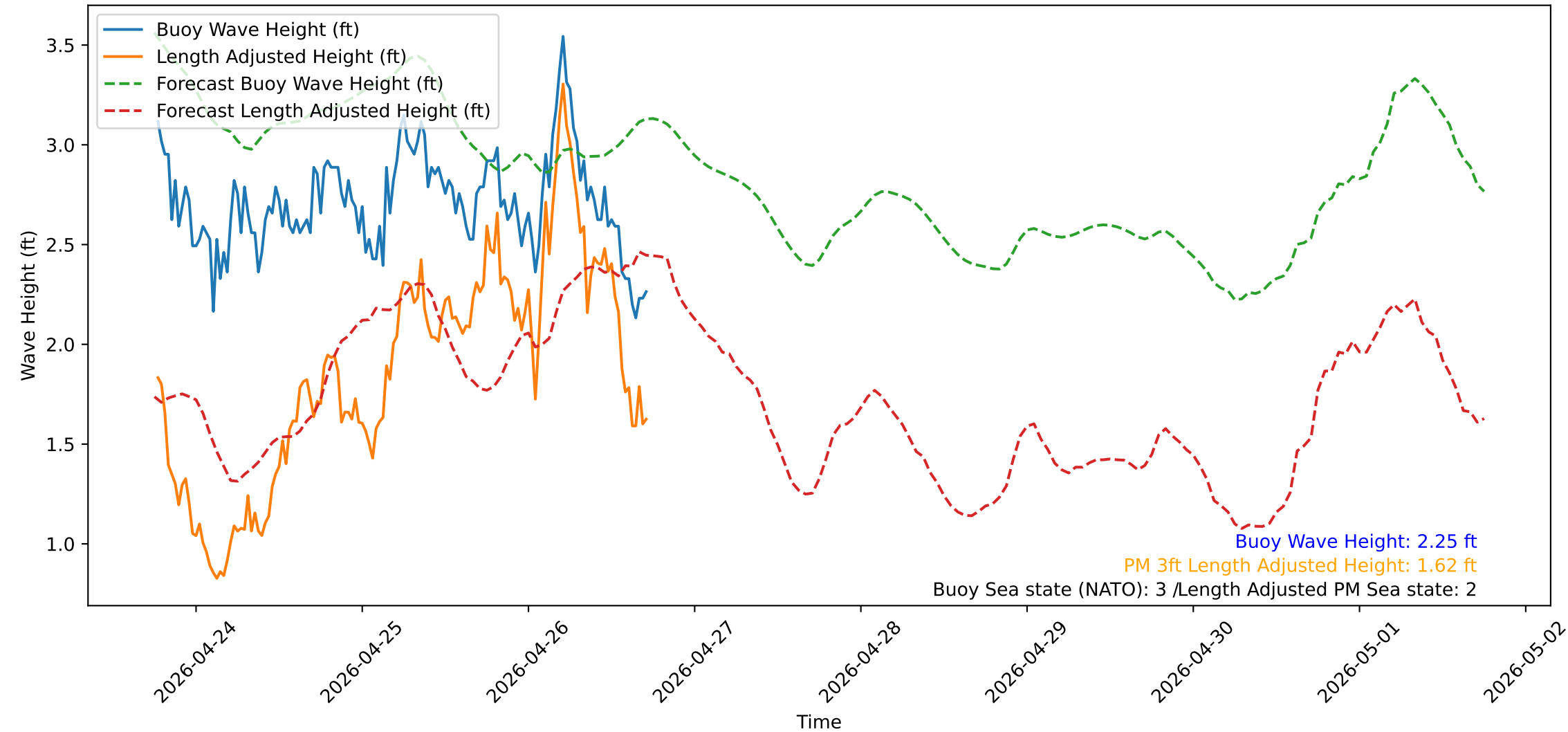
Wave Heights over Time for Red Beach at 2026-04-26 18:00:50
