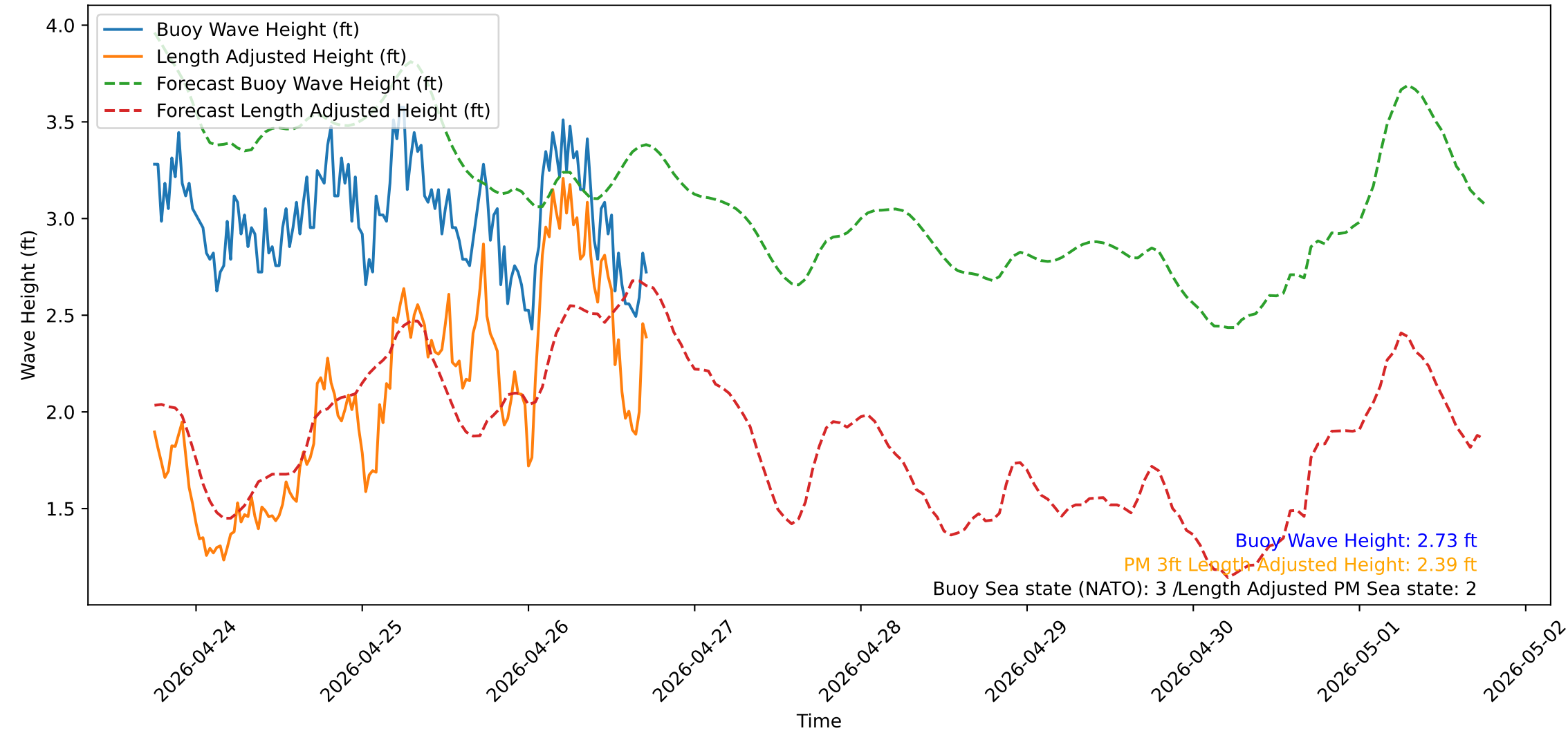
Wave Heights over Time for Green Beach at 2026-04-26 18:01:12
