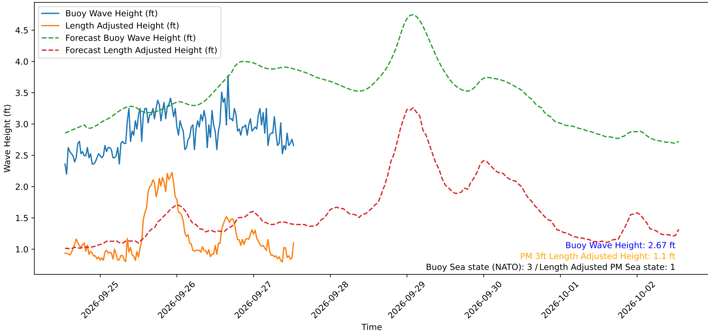
Wave Heights over Time for Oceanside Harbor at 2026-09-27 13:00:30
