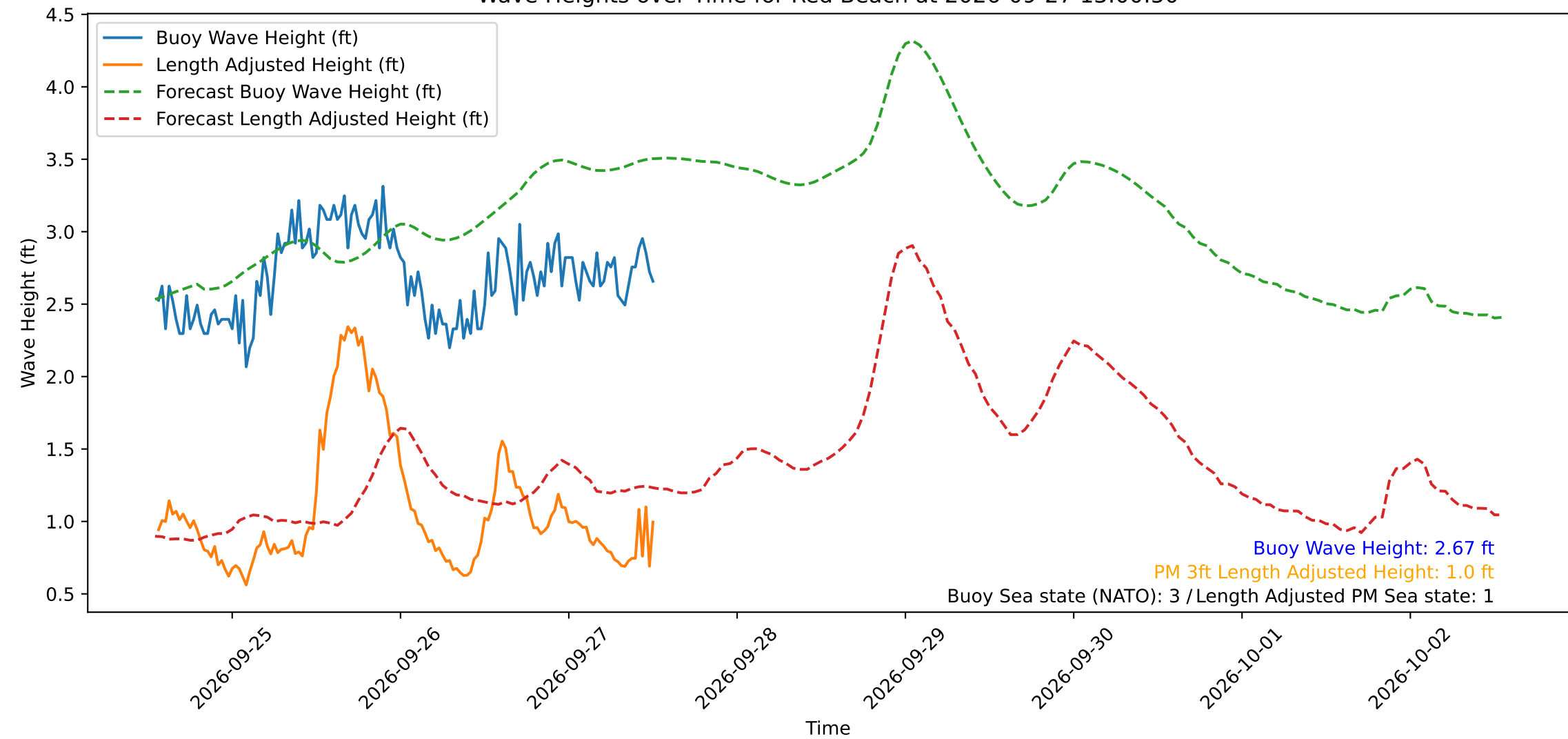
Wave Heights over Time for Red Beach at 2026-09-27 13:00:50
