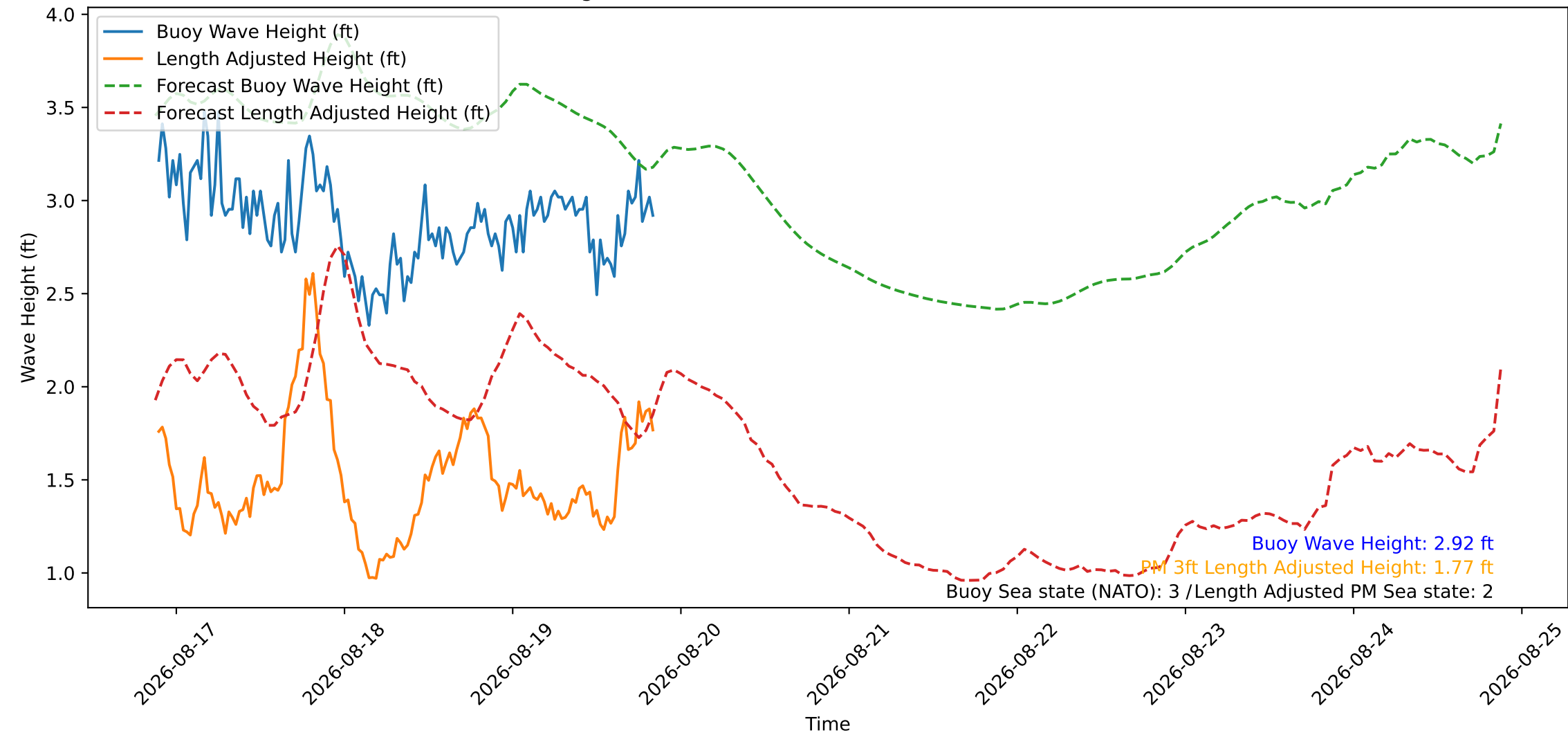
Wave Heights over Time for Red Beach at 2026-08-19 21:00:46
