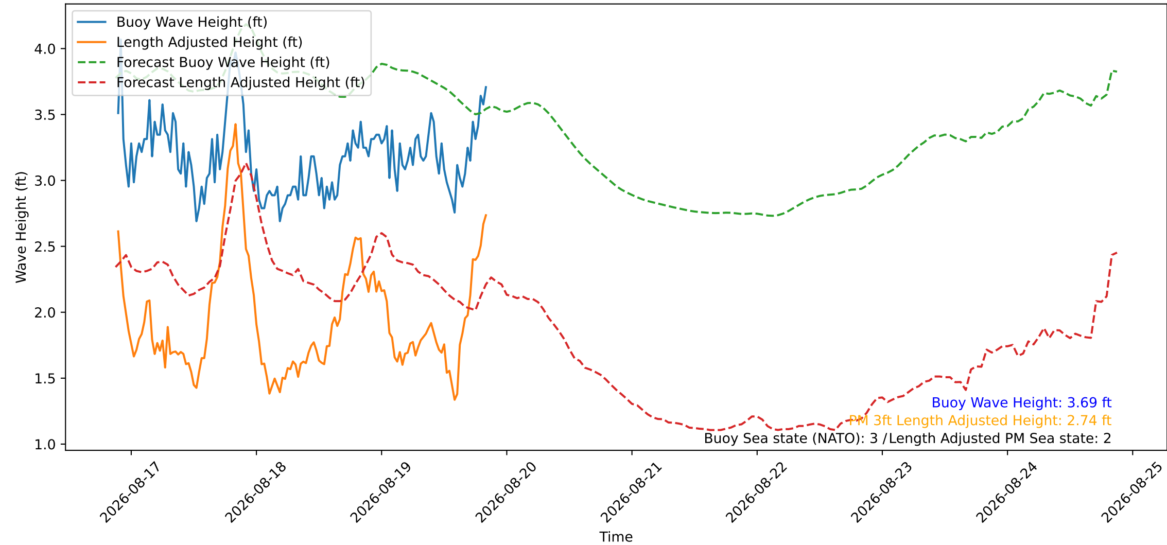
Wave Heights over Time for Green Beach at 2026-08-19 21:01:08
