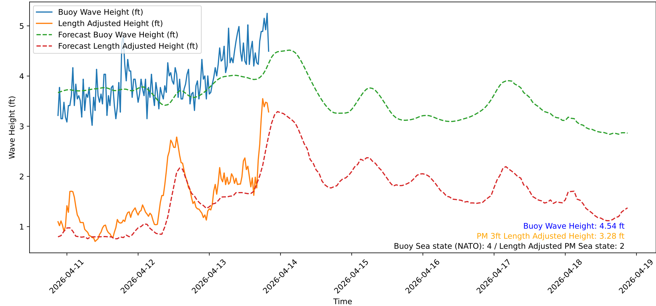
Wave Heights over Time for Oceanside Harbor at 2026-04-13 21:10:31
