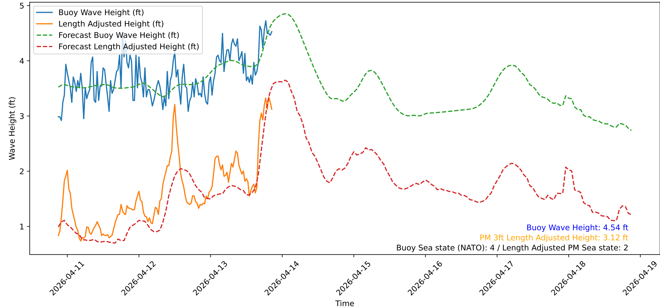
Wave Heights over Time for Green Beach at 2026-04-13 21:11:12
