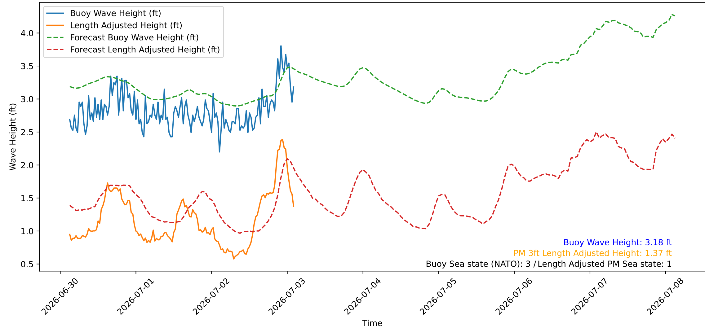
Wave Heights over Time for Red Beach at 2026-07-03 02:40:45
