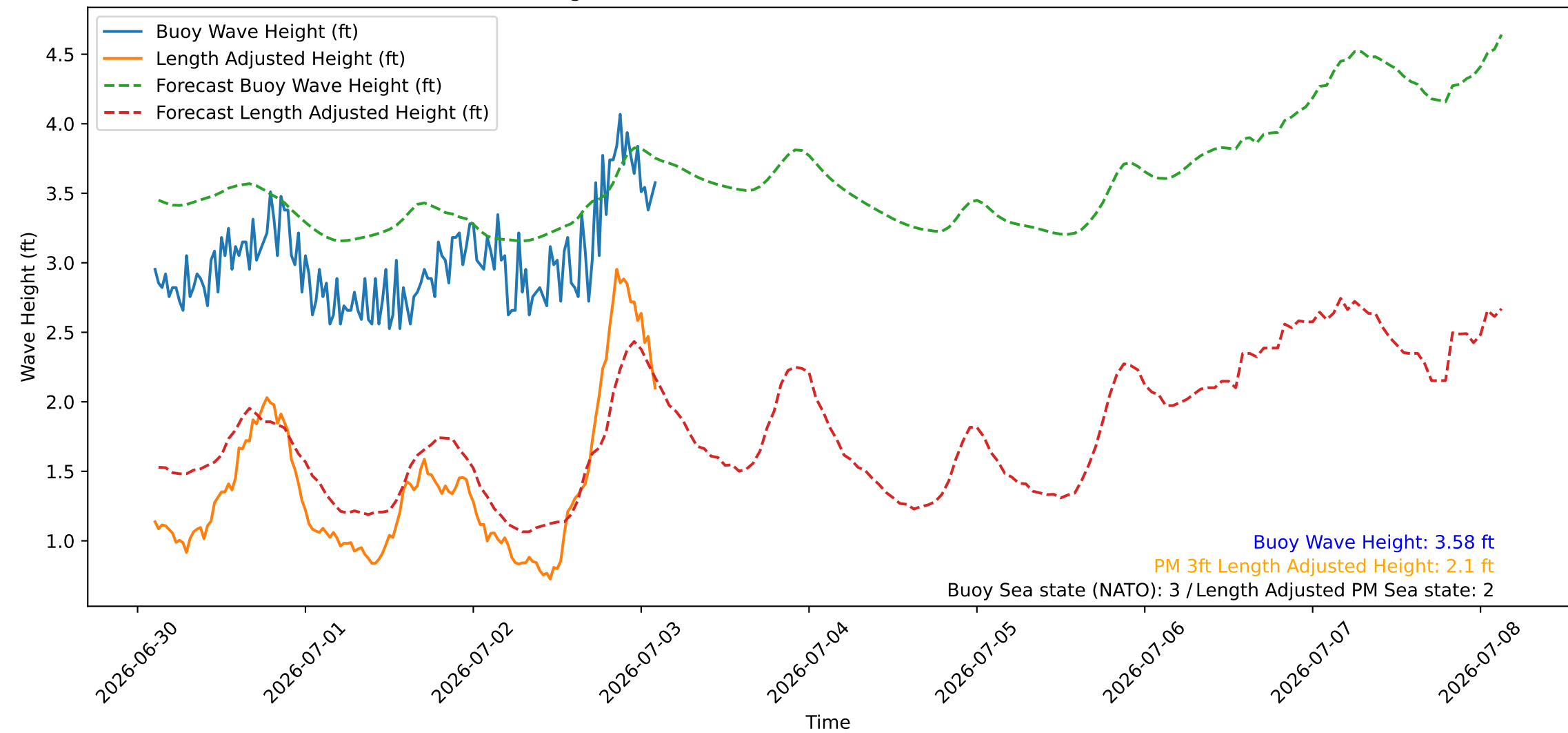
Wave Heights over Time for Green Beach at 2026-07-03 02:41:07
