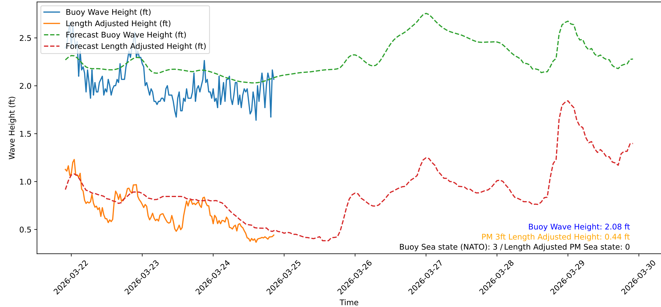
Wave Heights over Time for Red Beach at 2026-03-24 21:30:47
