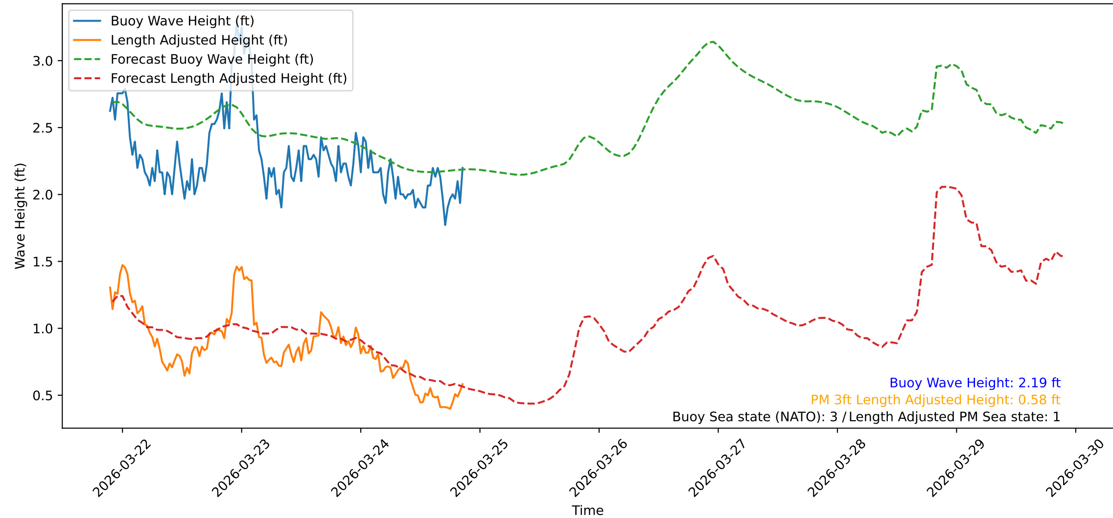
Wave Heights over Time for Green Beach at 2026-03-24 21:31:08
