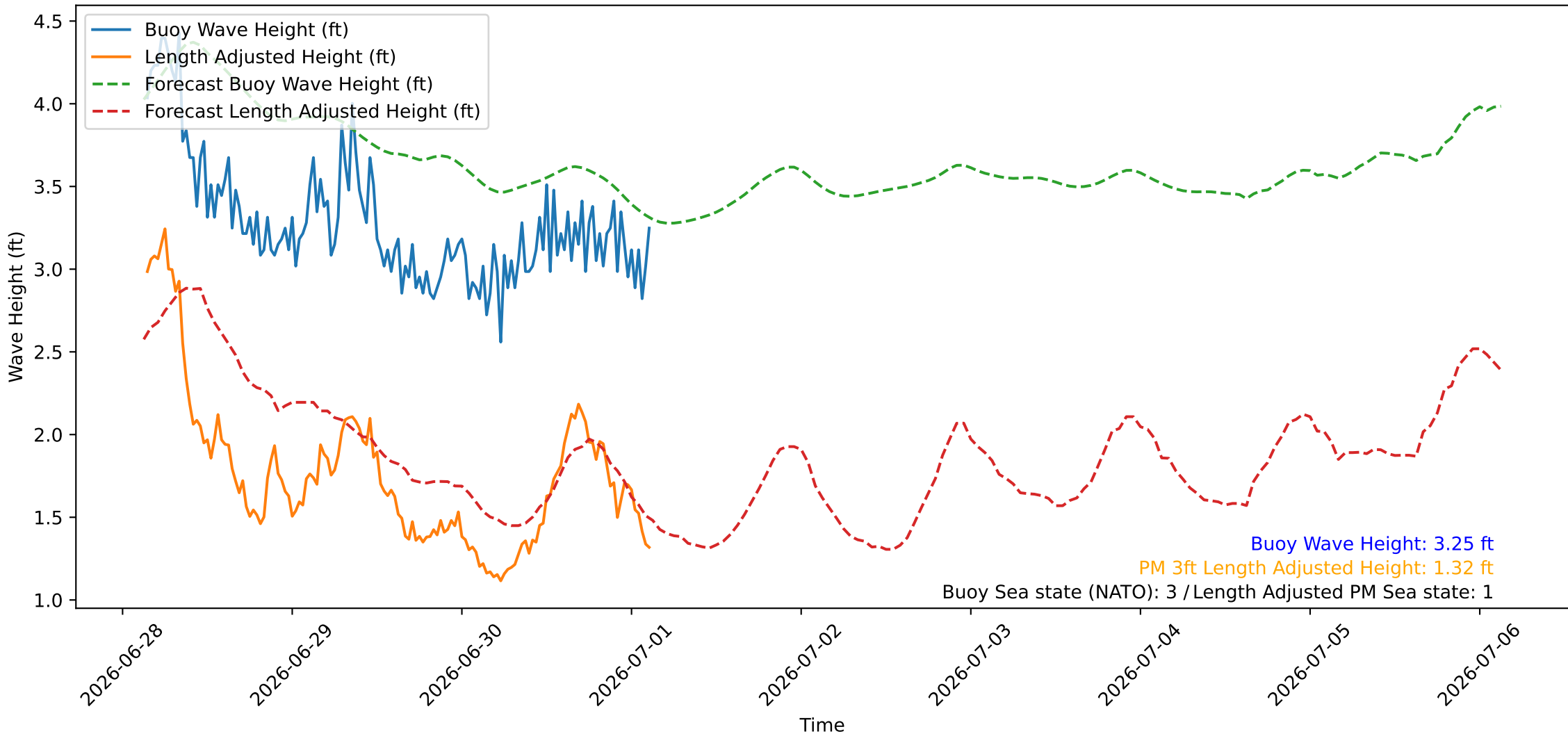
Wave Heights over Time for Oceanside Harbor at 2026-07-01 03:20:26
