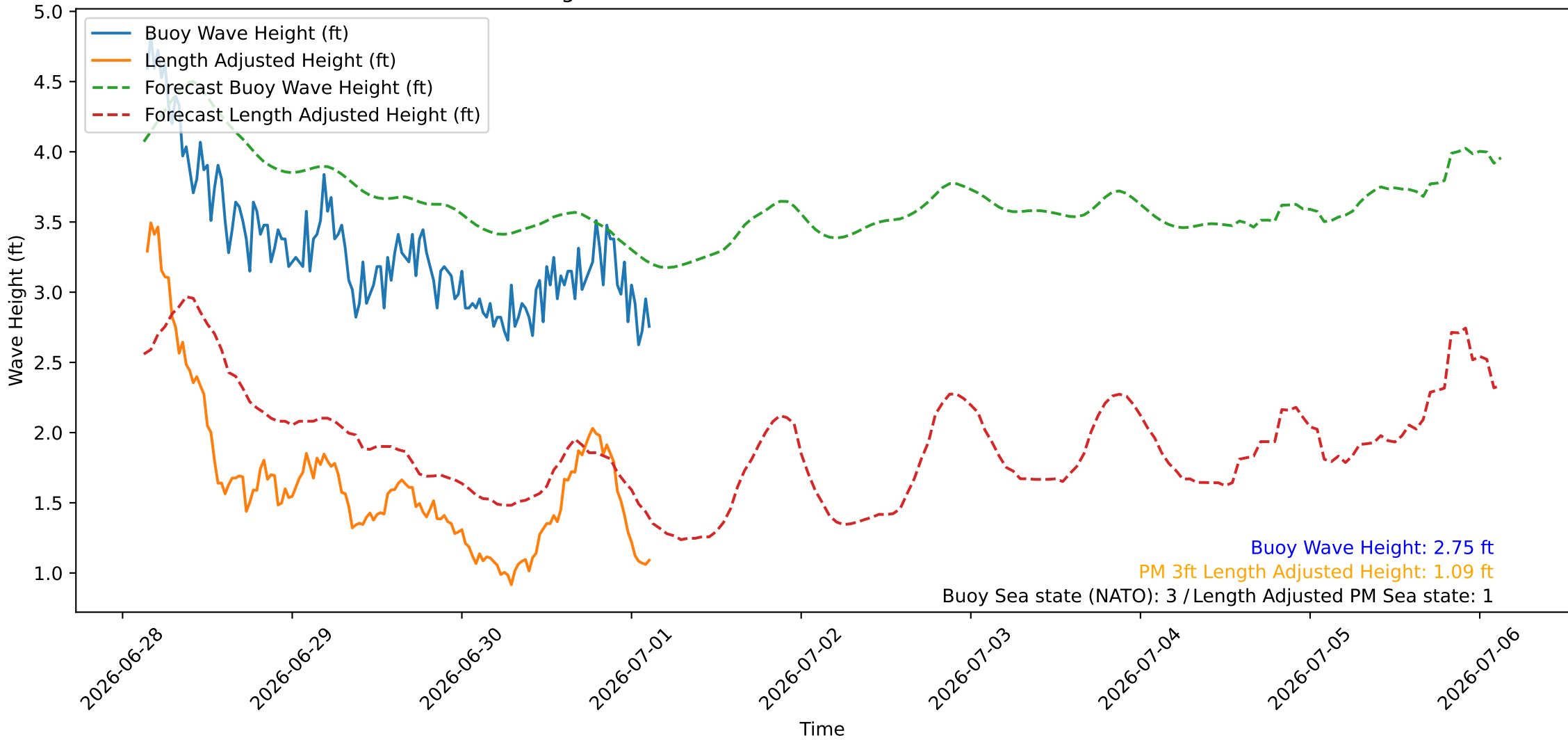
Wave Heights over Time for Green Beach at 2026-07-01 03:21:09
