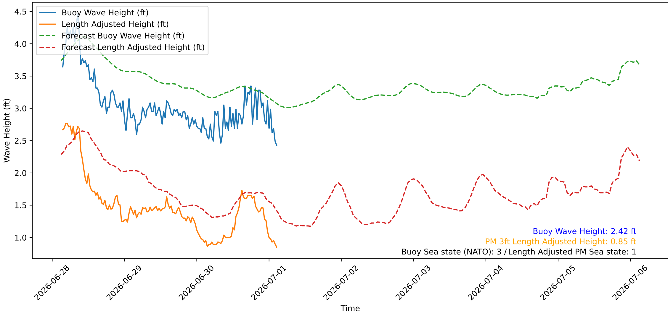
Wave Heights over Time for Red Beach at 2026-07-01 03:20:46
