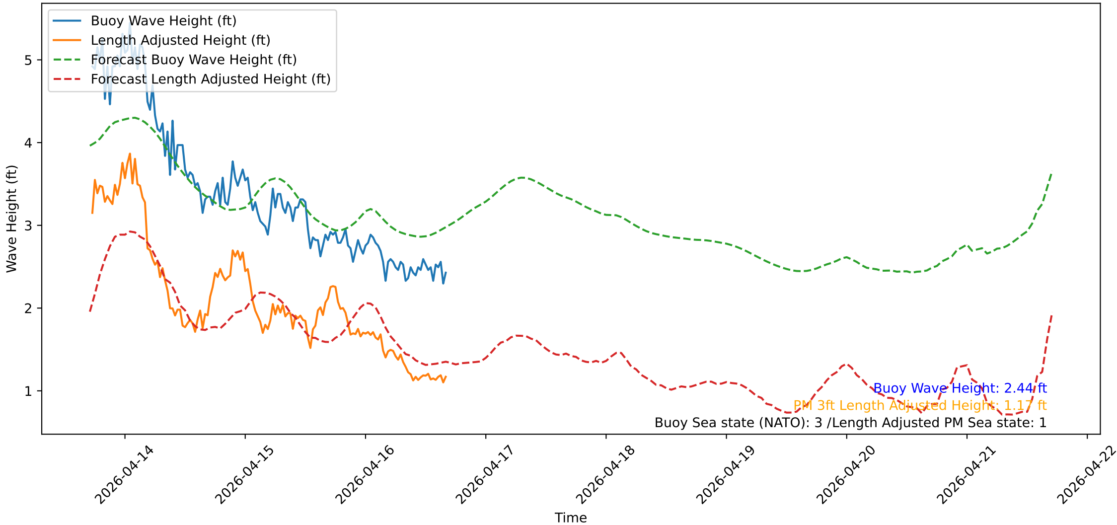
Wave Heights over Time for Oceanside Harbor at 2026-04-16 17:20:32
