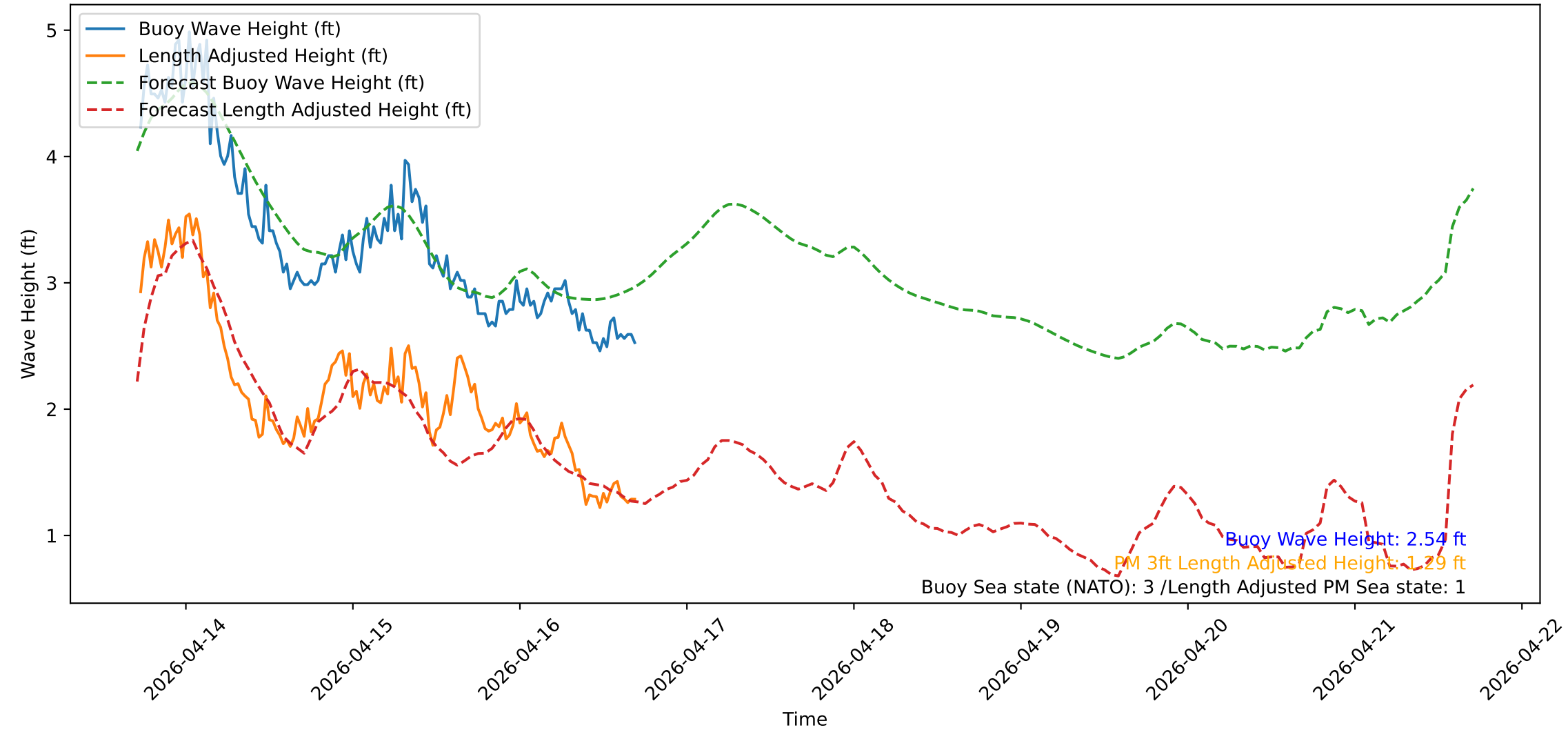
Wave Heights over Time for Green Beach at 2026-04-16 17:21:16
