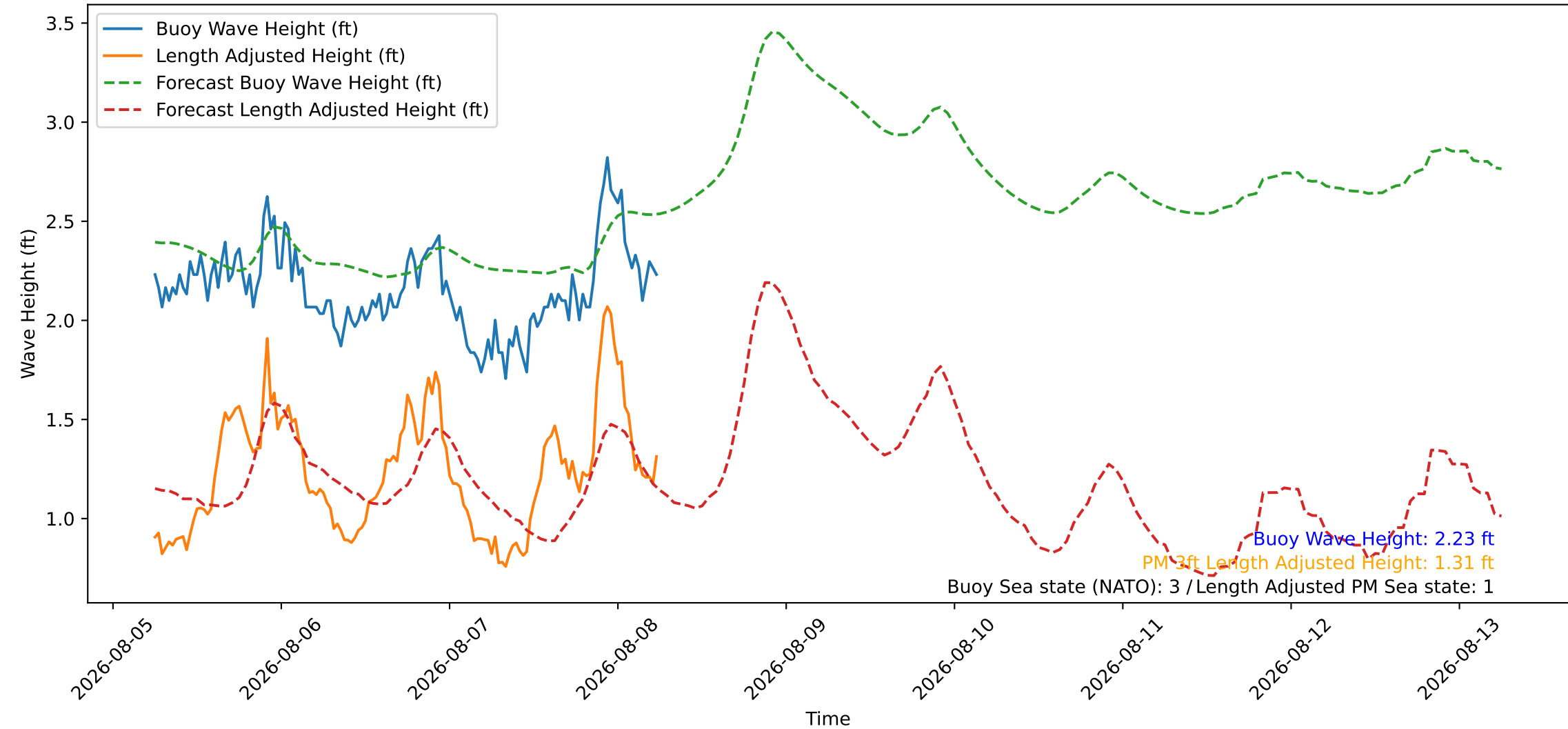
Wave Heights over Time for Green Beach at 2026-08-08 06:11:09
