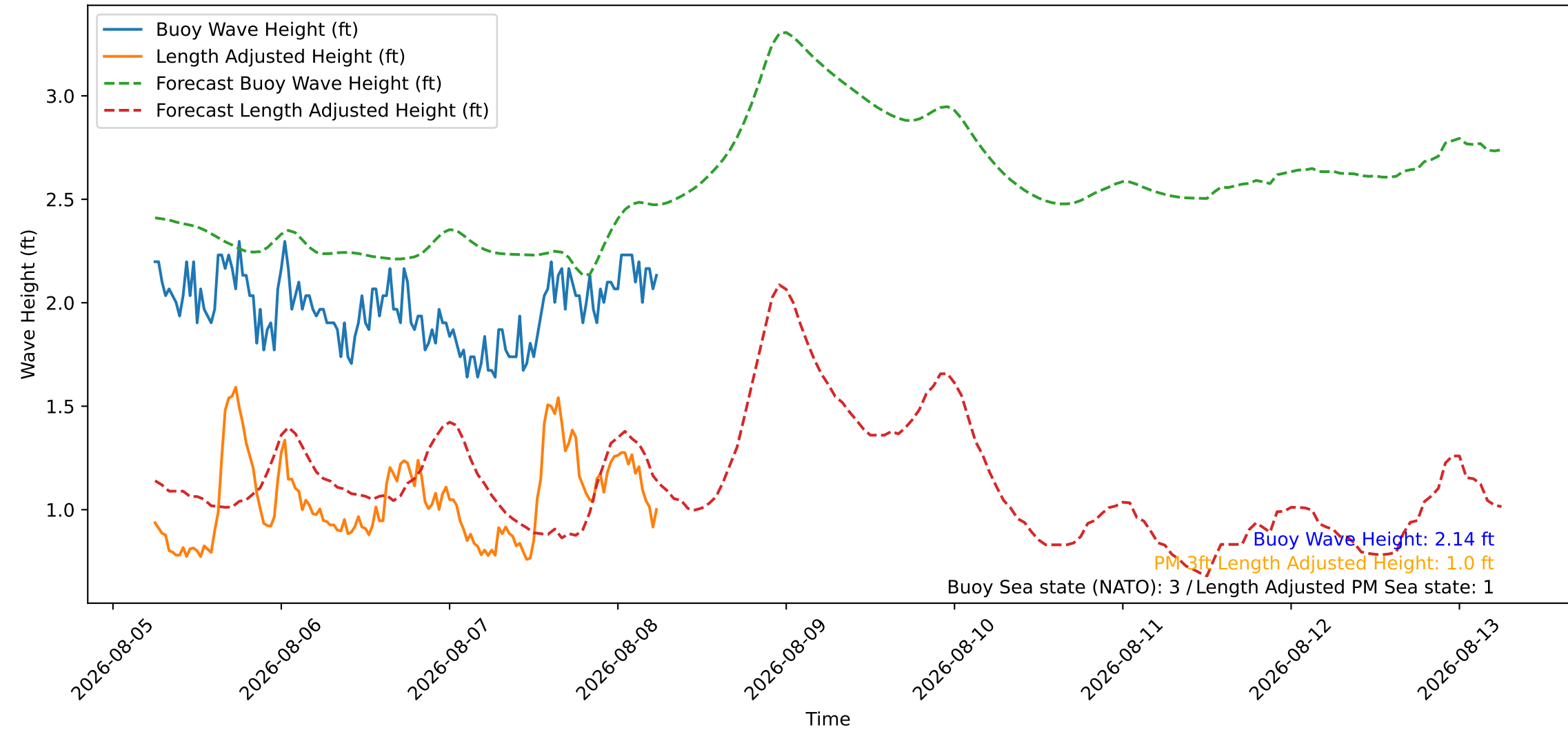
Wave Heights over Time for Oceanside Harbor at 2026-08-08 06:10:27
