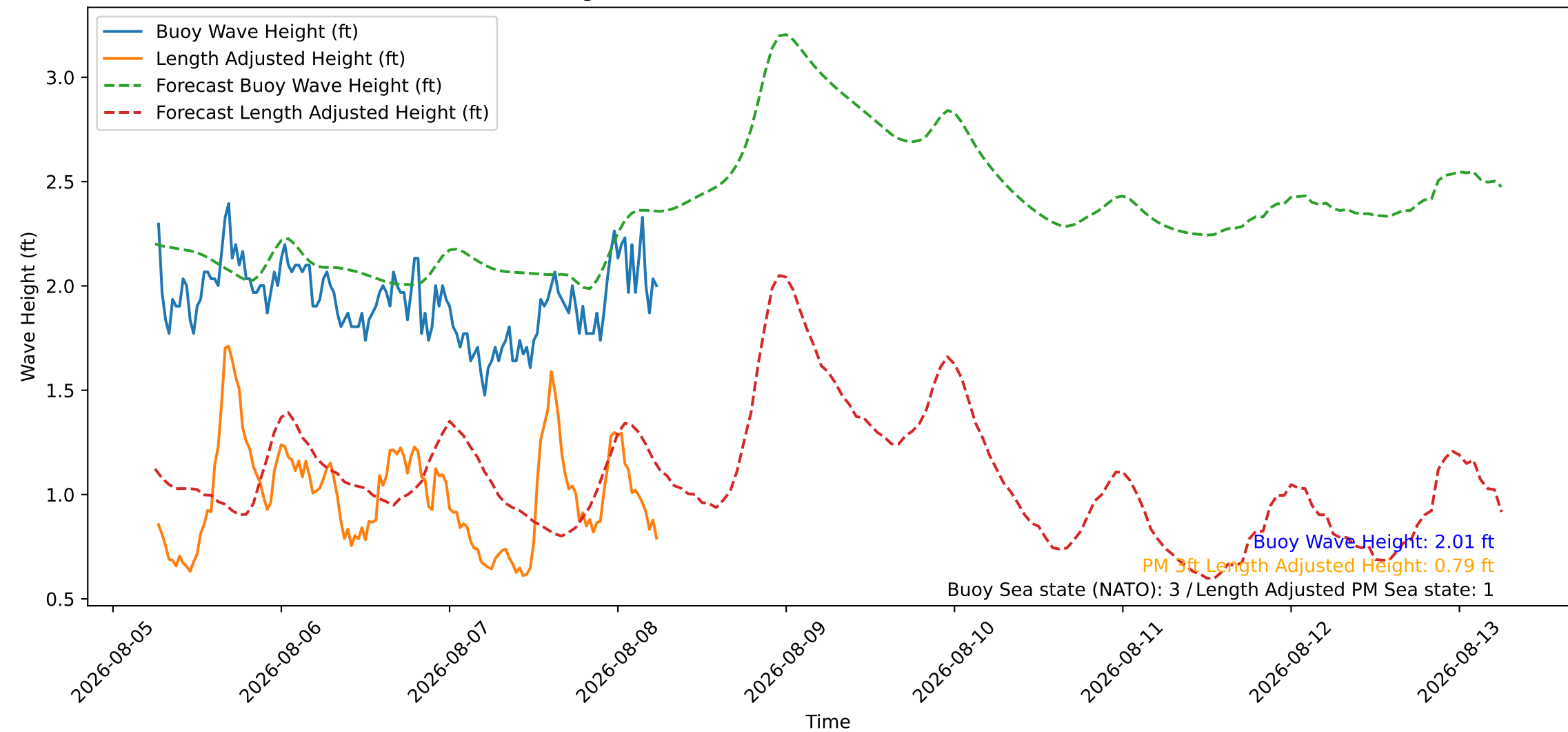
Wave Heights over Time for Red Beach at 2026-08-08 06:10:46
