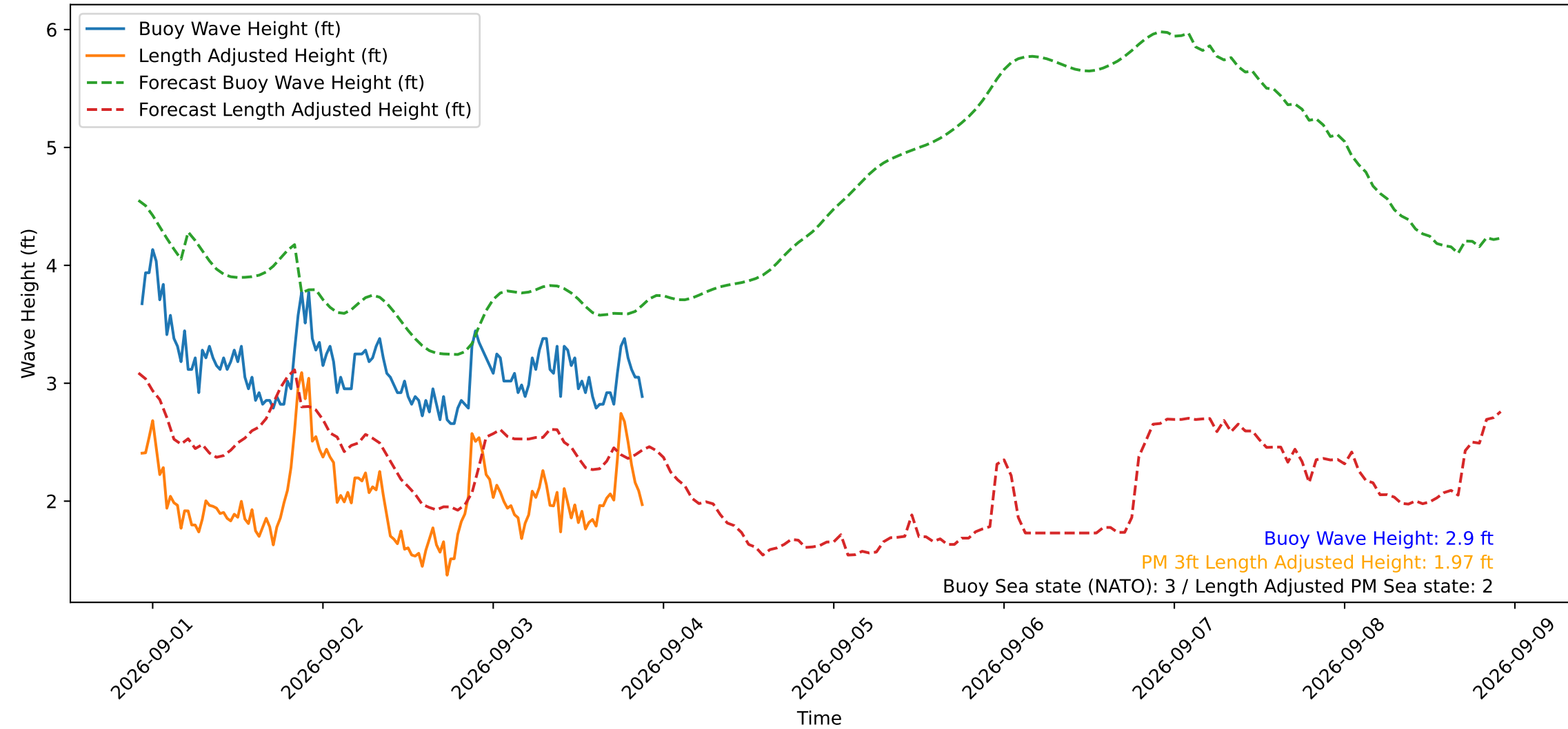
Wave Heights over Time for Green Beach at 2026-09-03 22:01:13
