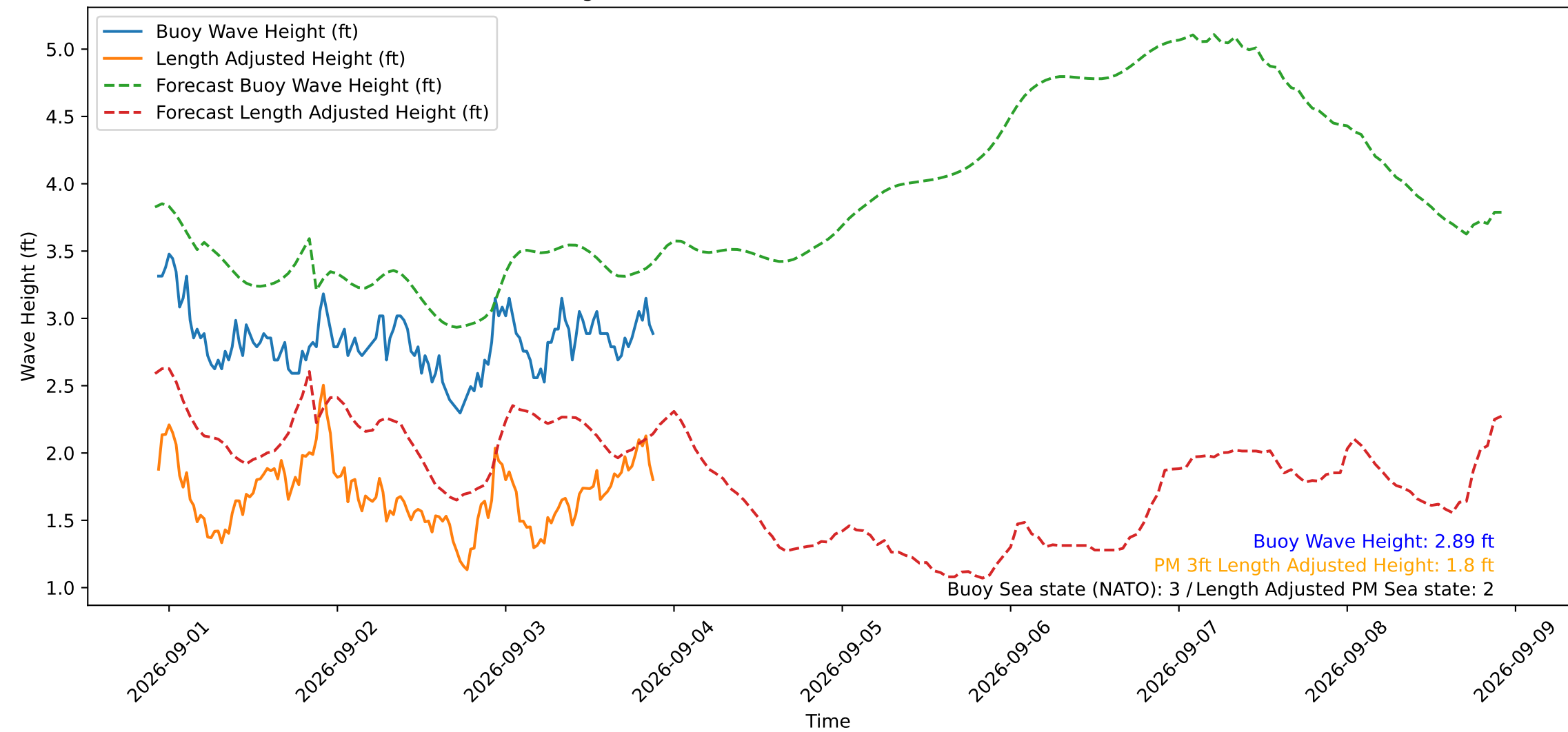
Wave Heights over Time for Red Beach at 2026-09-03 22:00:50
