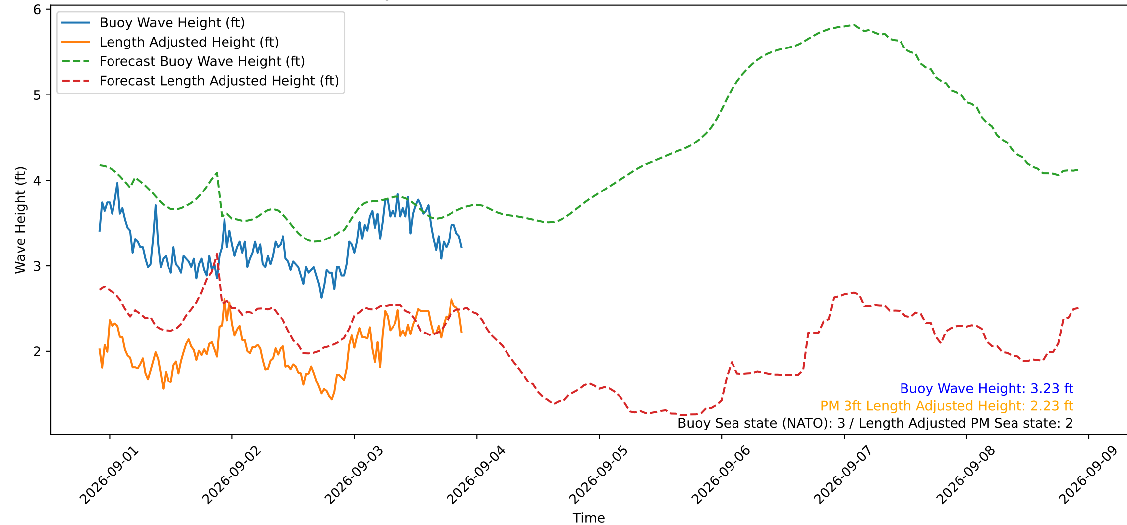
Wave Heights over Time for Oceanside Harbor at 2026-09-03 22:00:30
