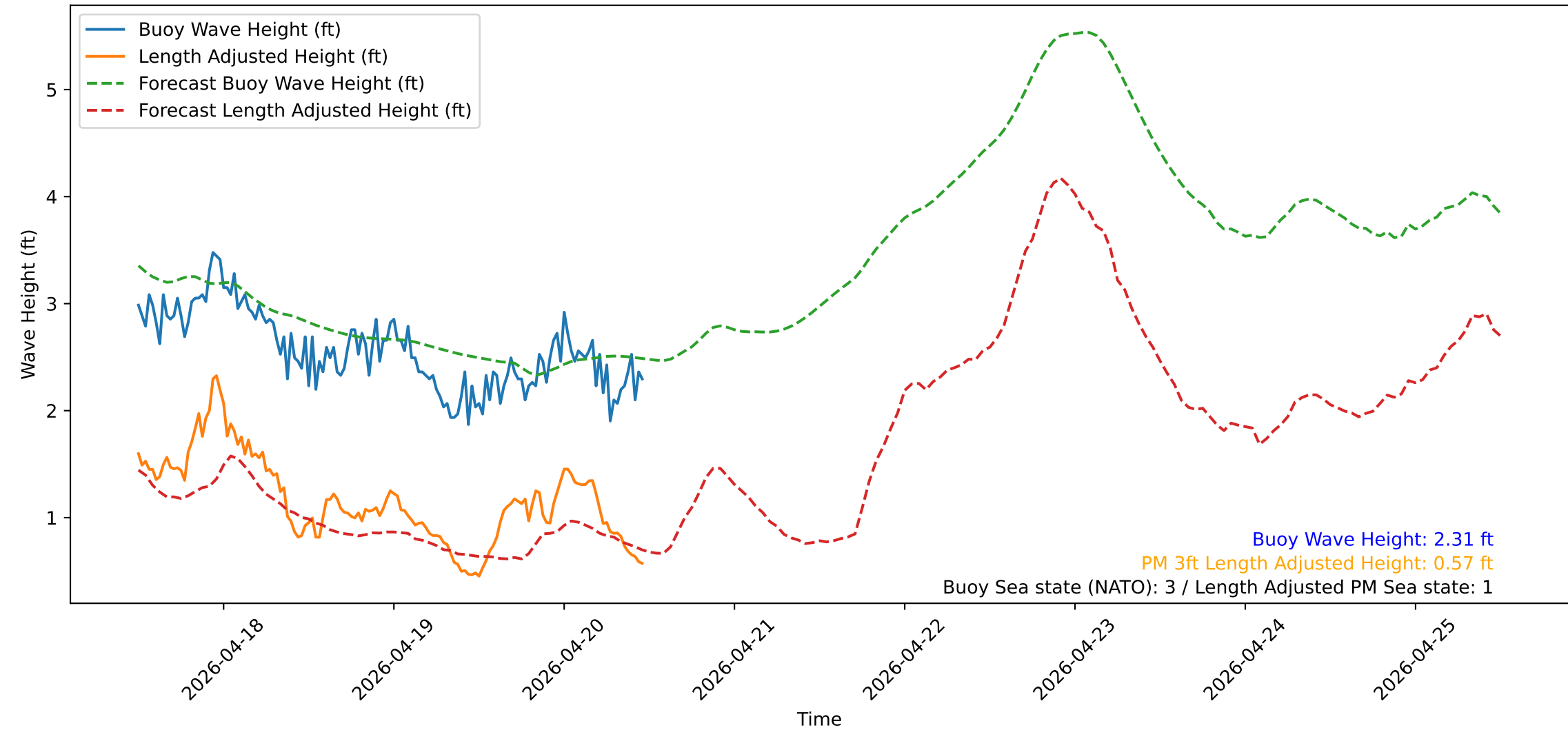
Wave Heights over Time for Green Beach at 2026-04-20 11:51:14
