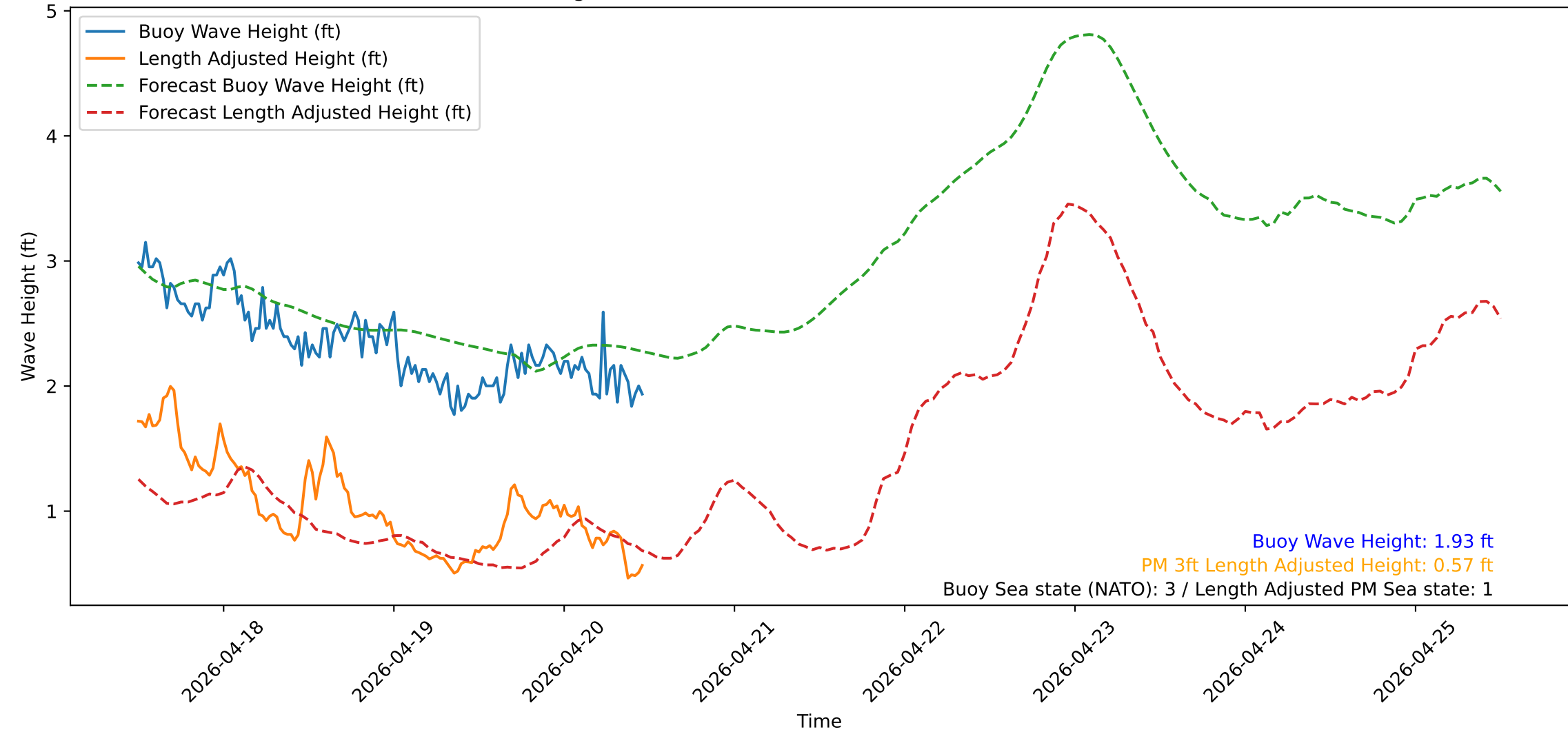
Wave Heights over Time for Red Beach at 2026-04-20 11:50:51
