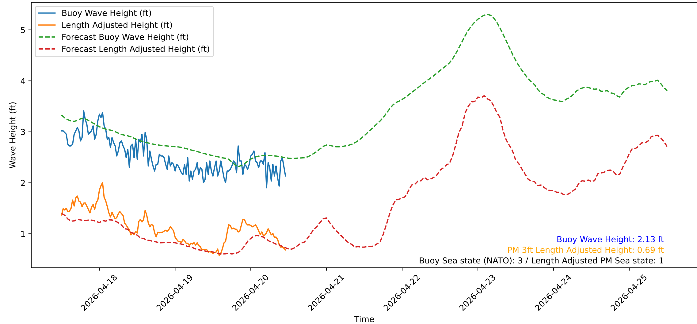
Wave Heights over Time for Oceanside Harbor at 2026-04-20 11:50:31
