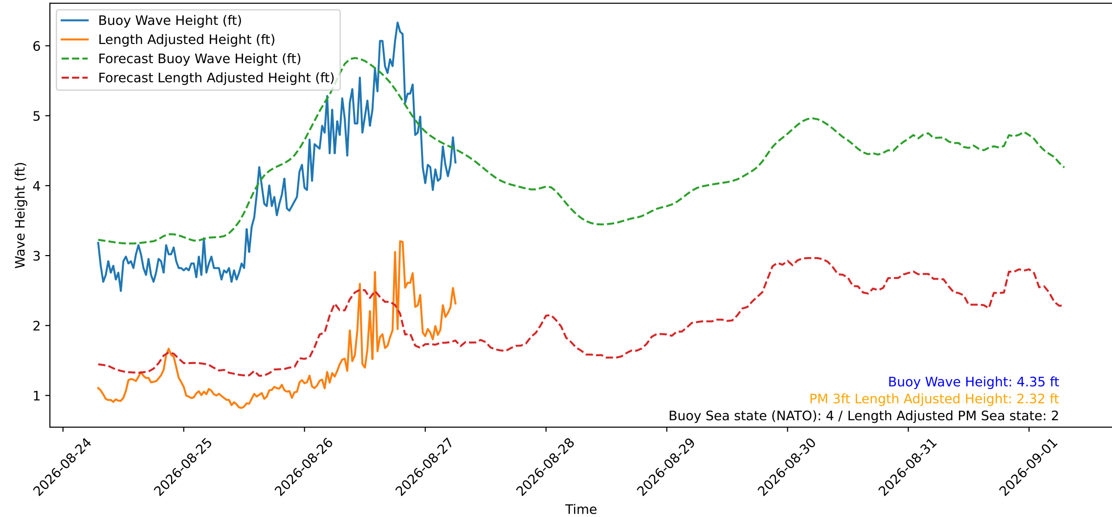
Wave Heights over Time for Green Beach at 2026-08-27 06:41:12
