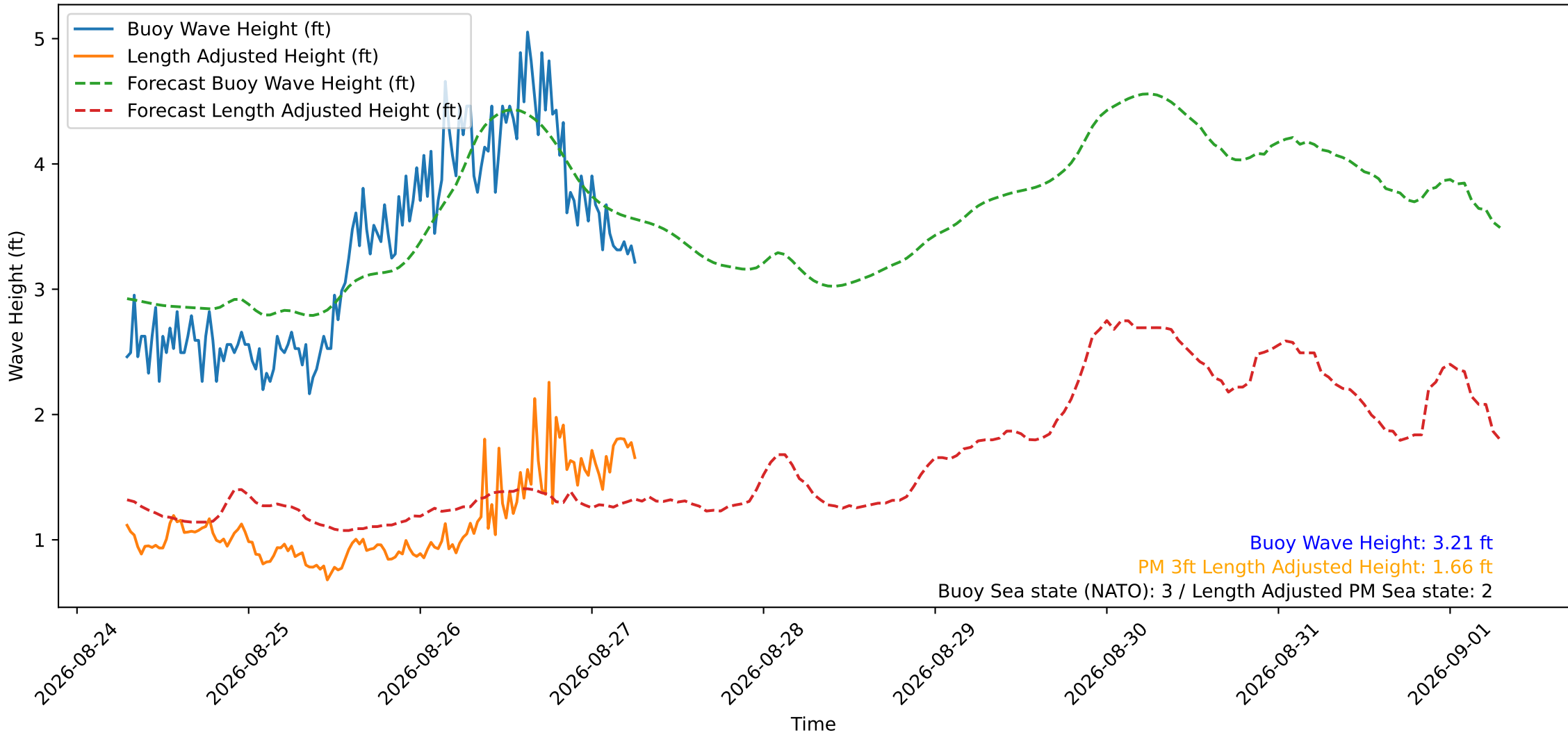
Wave Heights over Time for Red Beach at 2026-08-27 06:40:49
