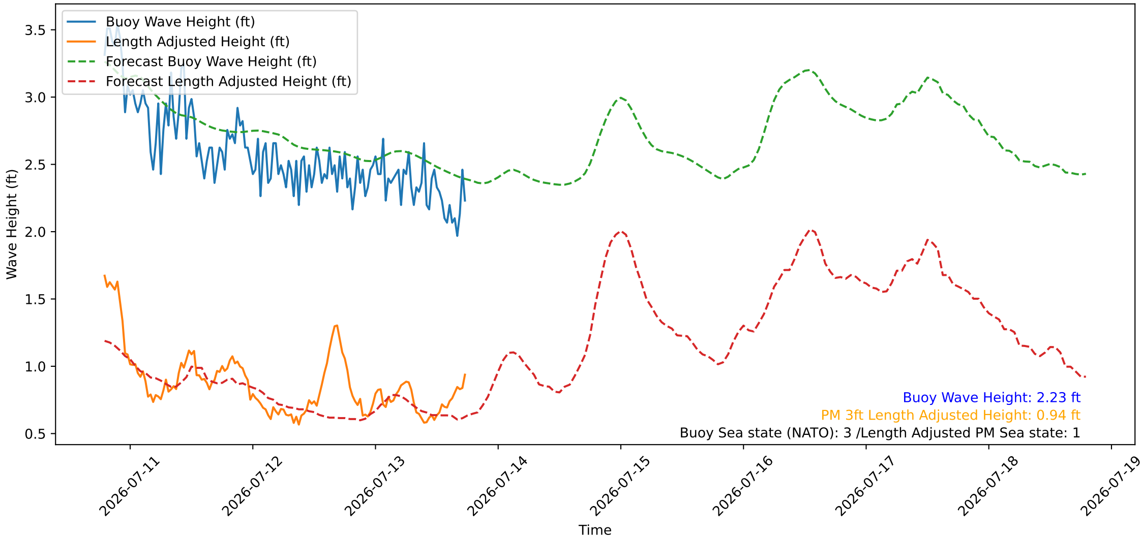
Wave Heights over Time for Red Beach at 2026-07-13 18:30:47
