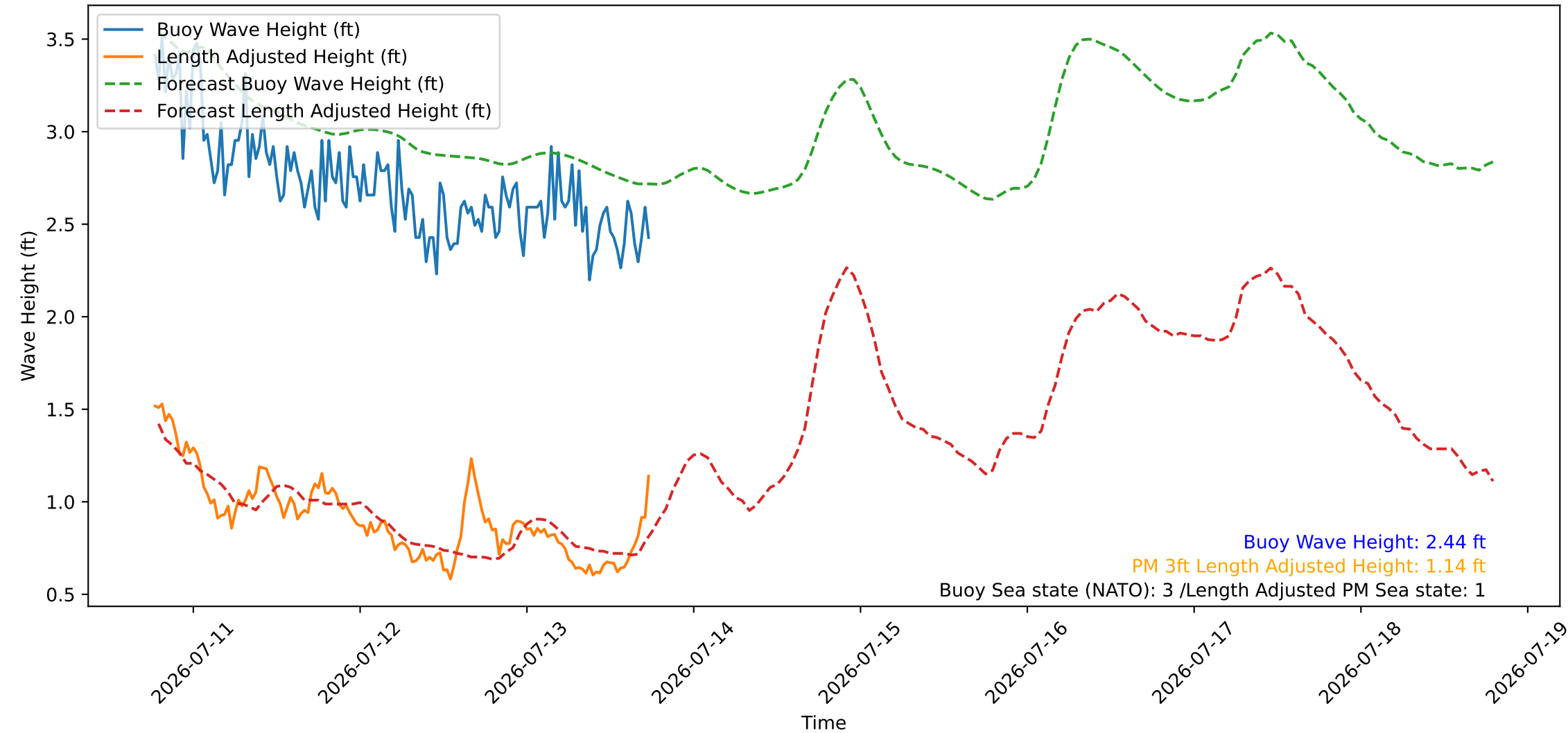
Wave Heights over Time for Green Beach at 2026-07-13 18:31:09
