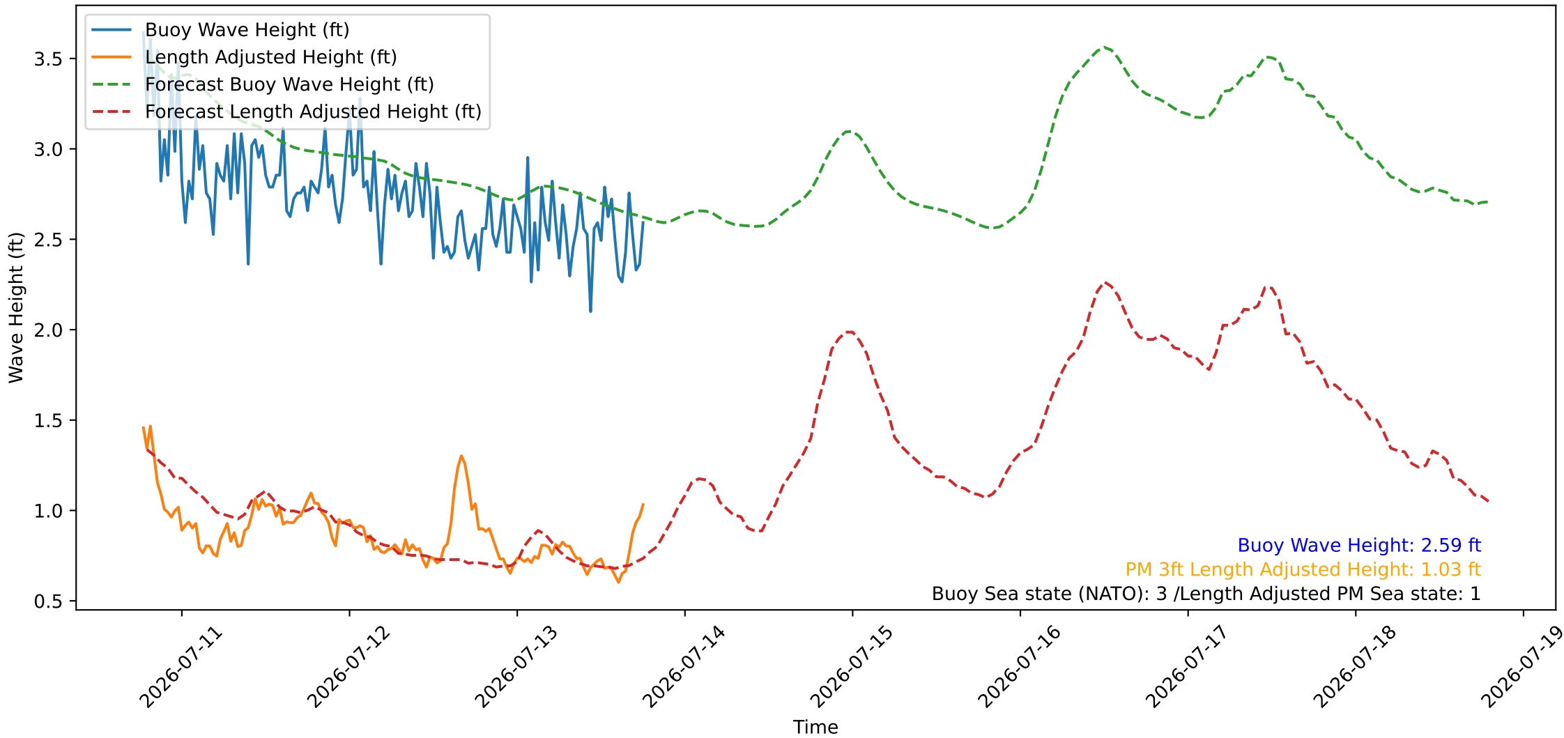
Wave Heights over Time for Oceanside Harbor at 2026-07-13 18:30:27
