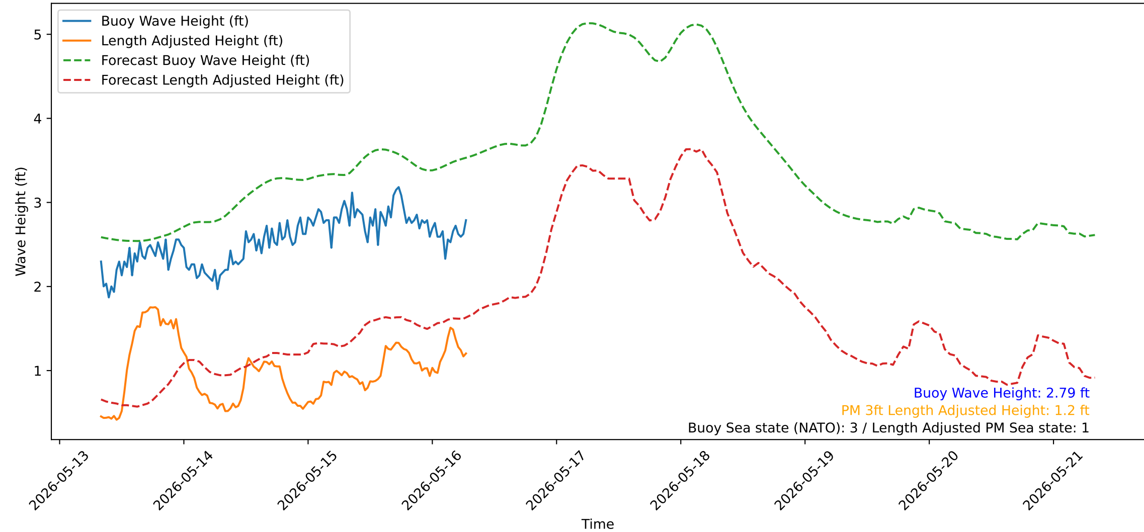
Wave Heights over Time for Red Beach at 2026-05-16 07:40:50
