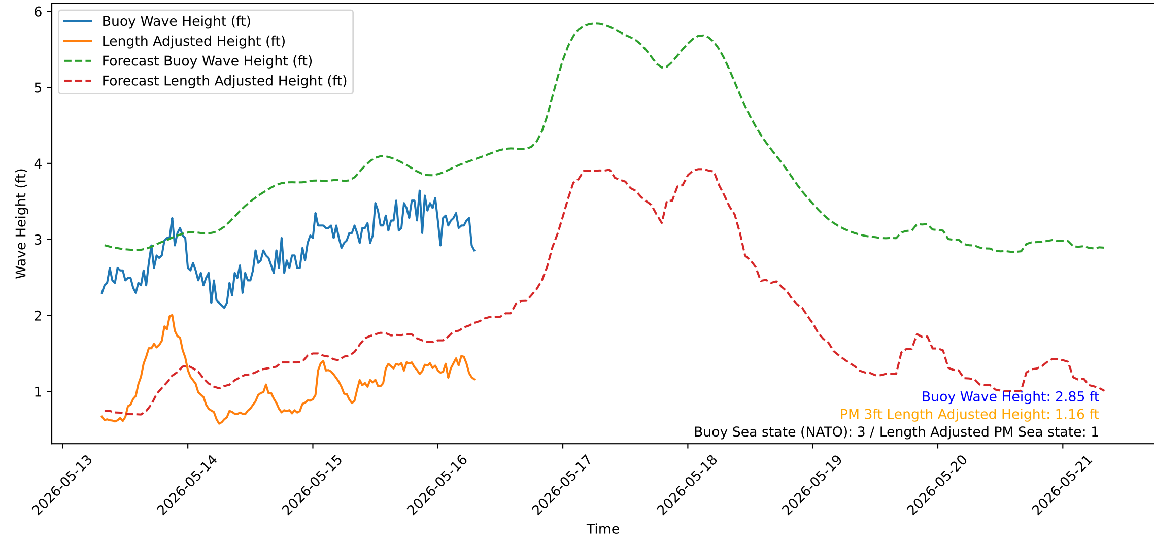
Wave Heights over Time for Green Beach at 2026-05-16 07:41:13
