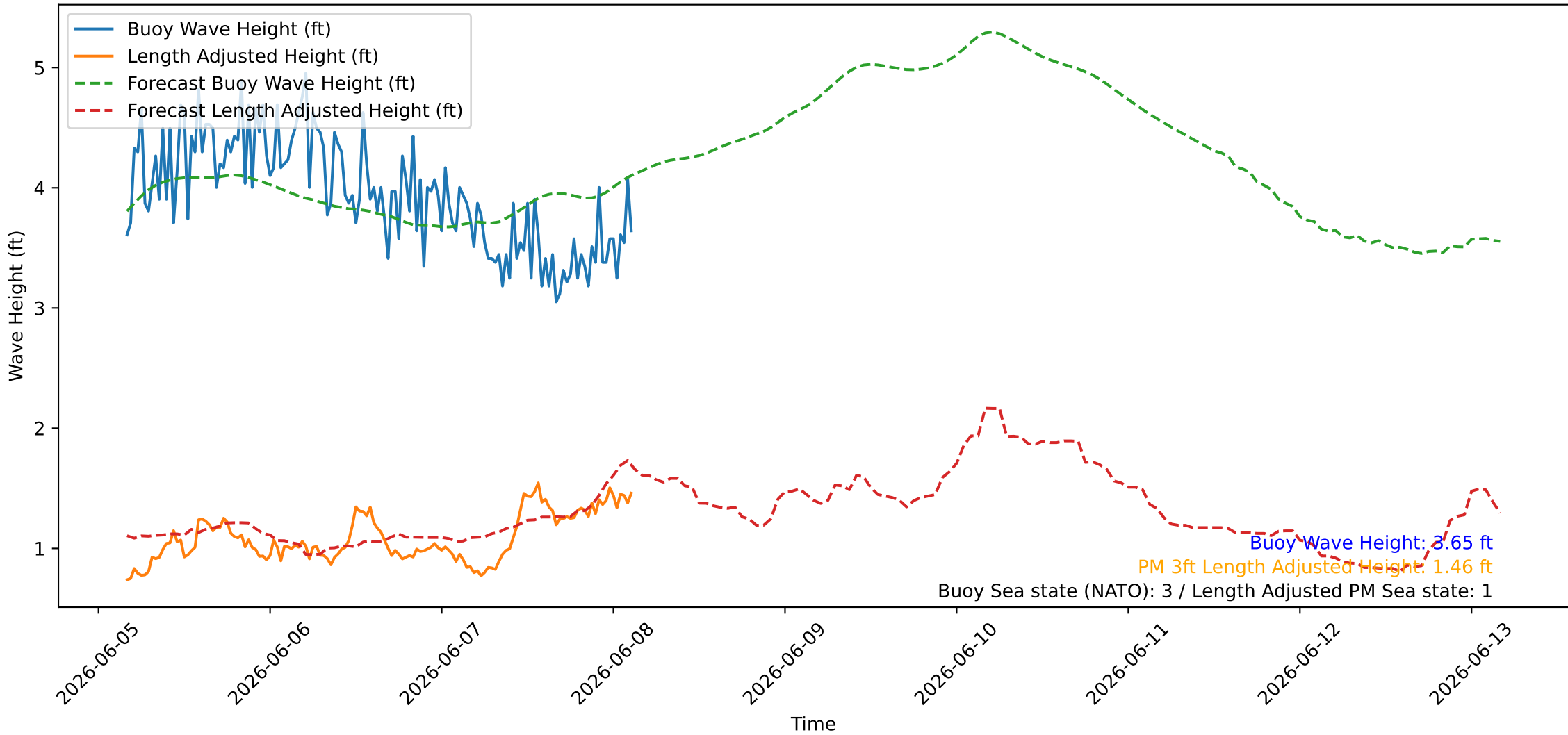
Wave Heights over Time for Red Beach at 2026-06-08 03:30:45
