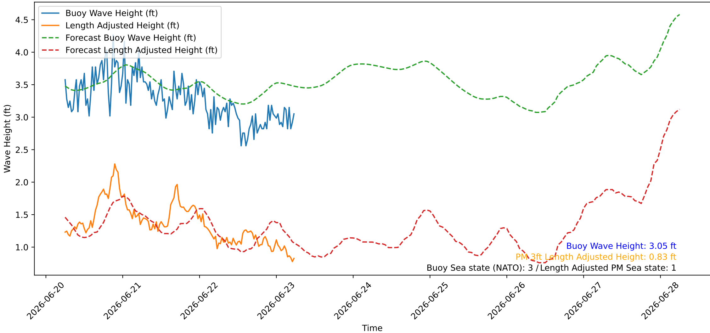
Wave Heights over Time for Oceanside Harbor at 2026-06-23 06:10:26
