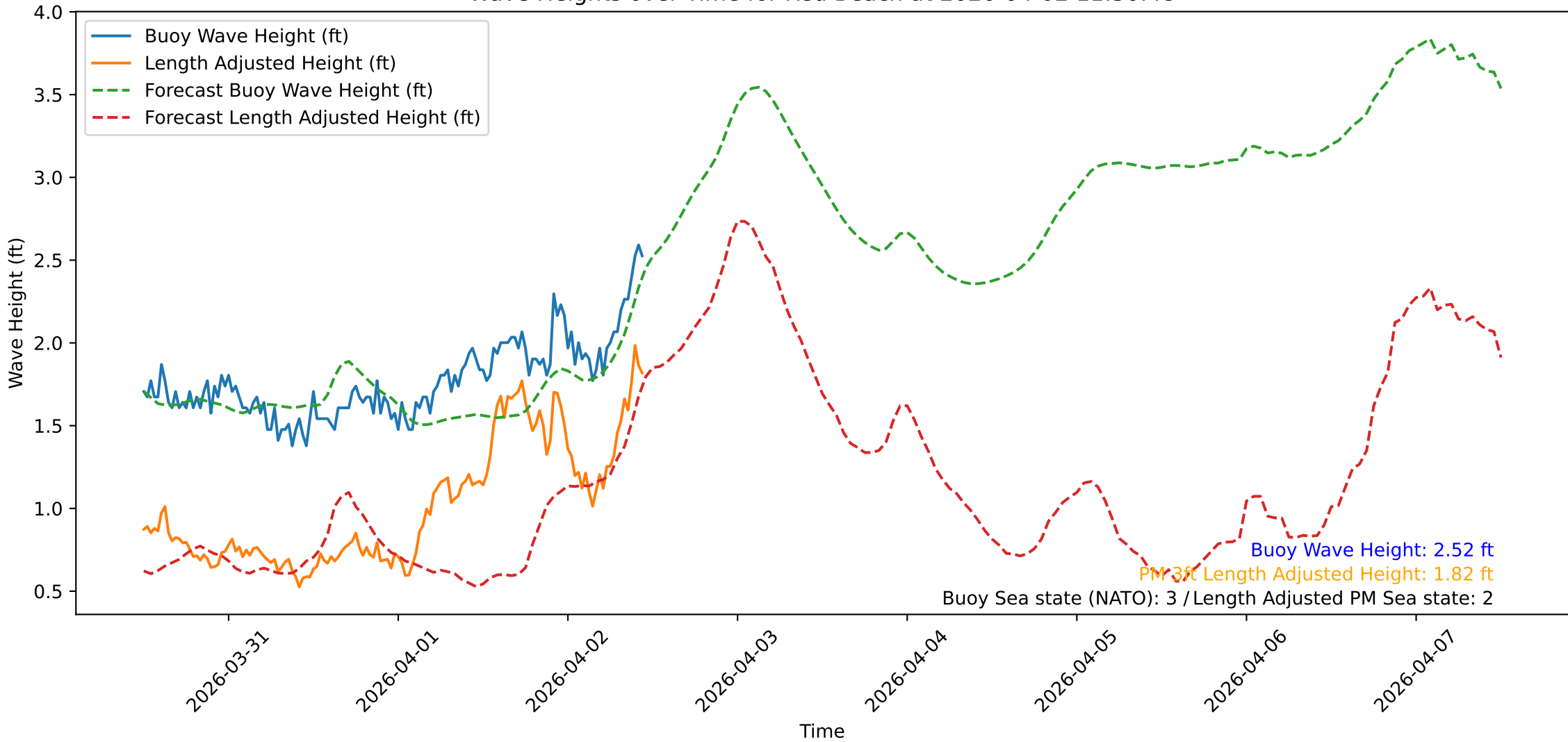
Wave Heights over Time for Red Beach at 2026-04-02 11:30:48
