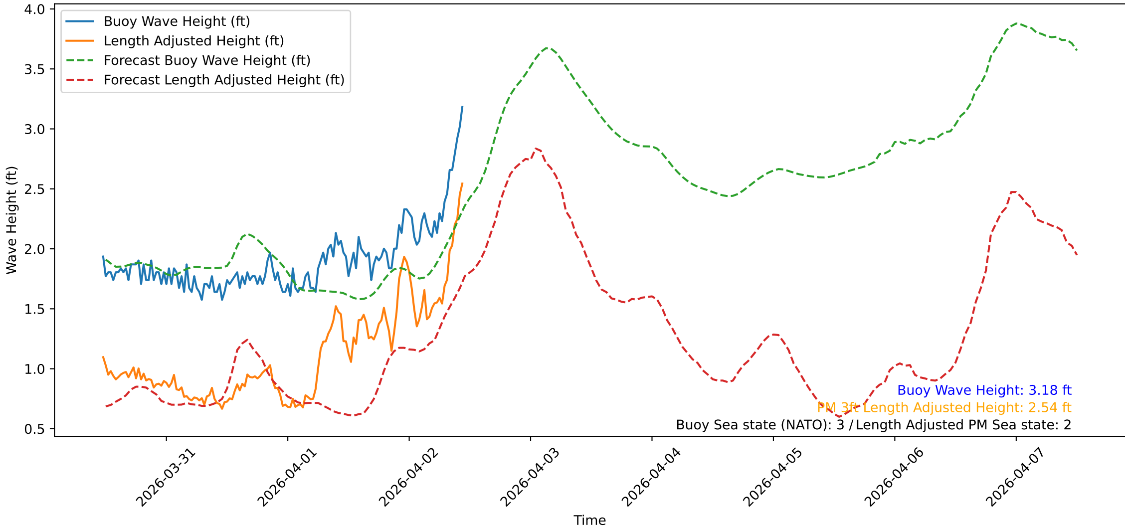
Wave Heights over Time for Oceanside Harbor at 2026-04-02 11:30:32
