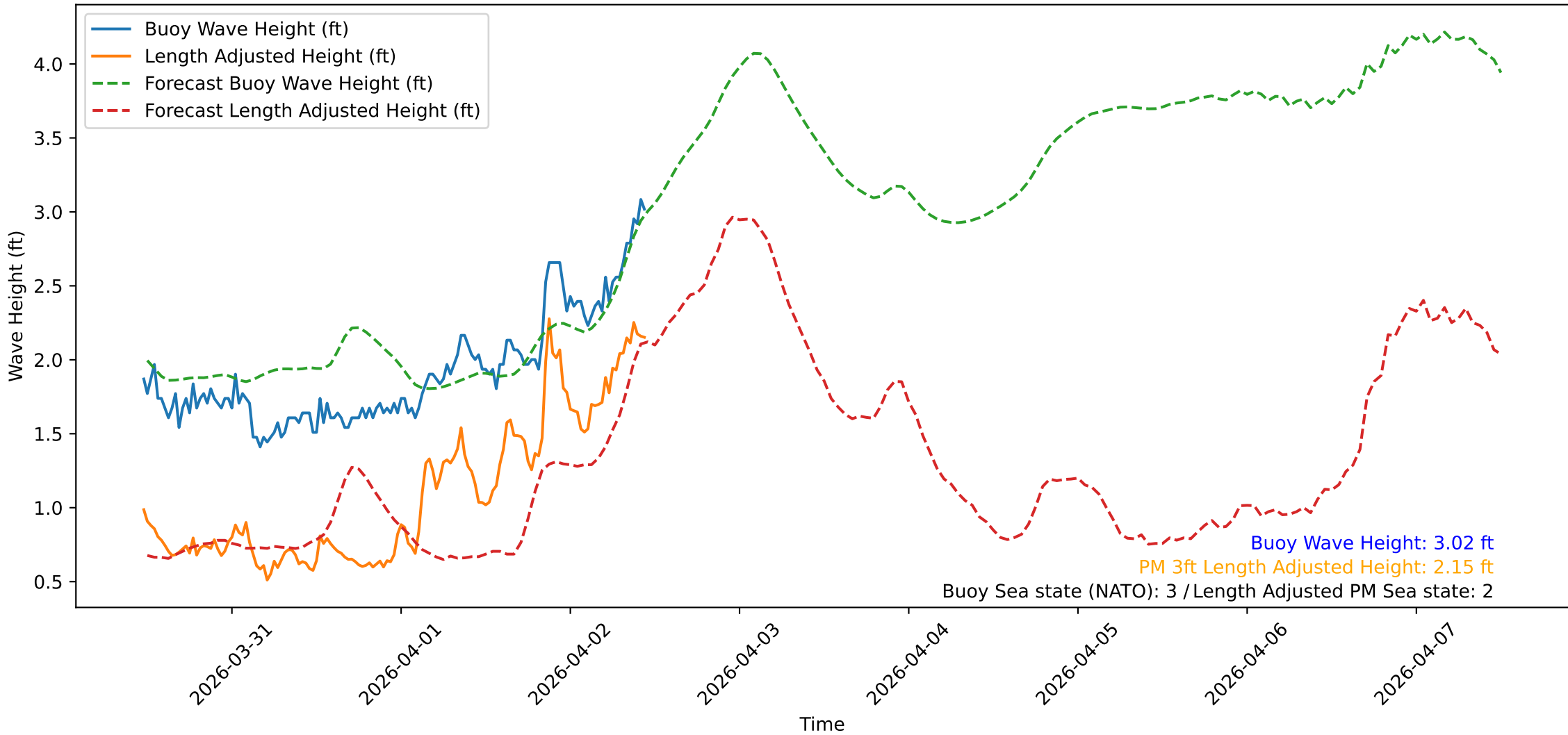
Wave Heights over Time for Green Beach at 2026-04-02 11:31:11
