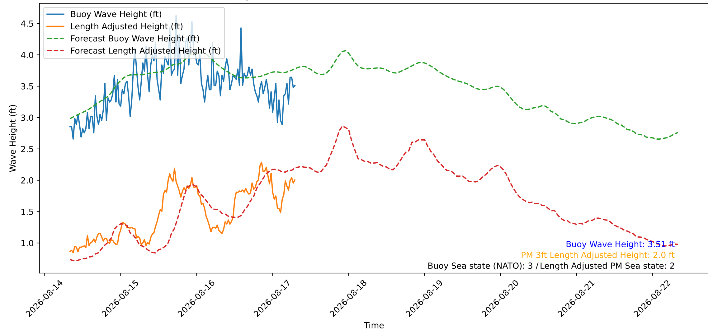
Wave Heights over Time for Oceanside Harbor at 2026-08-17 07:50:26
