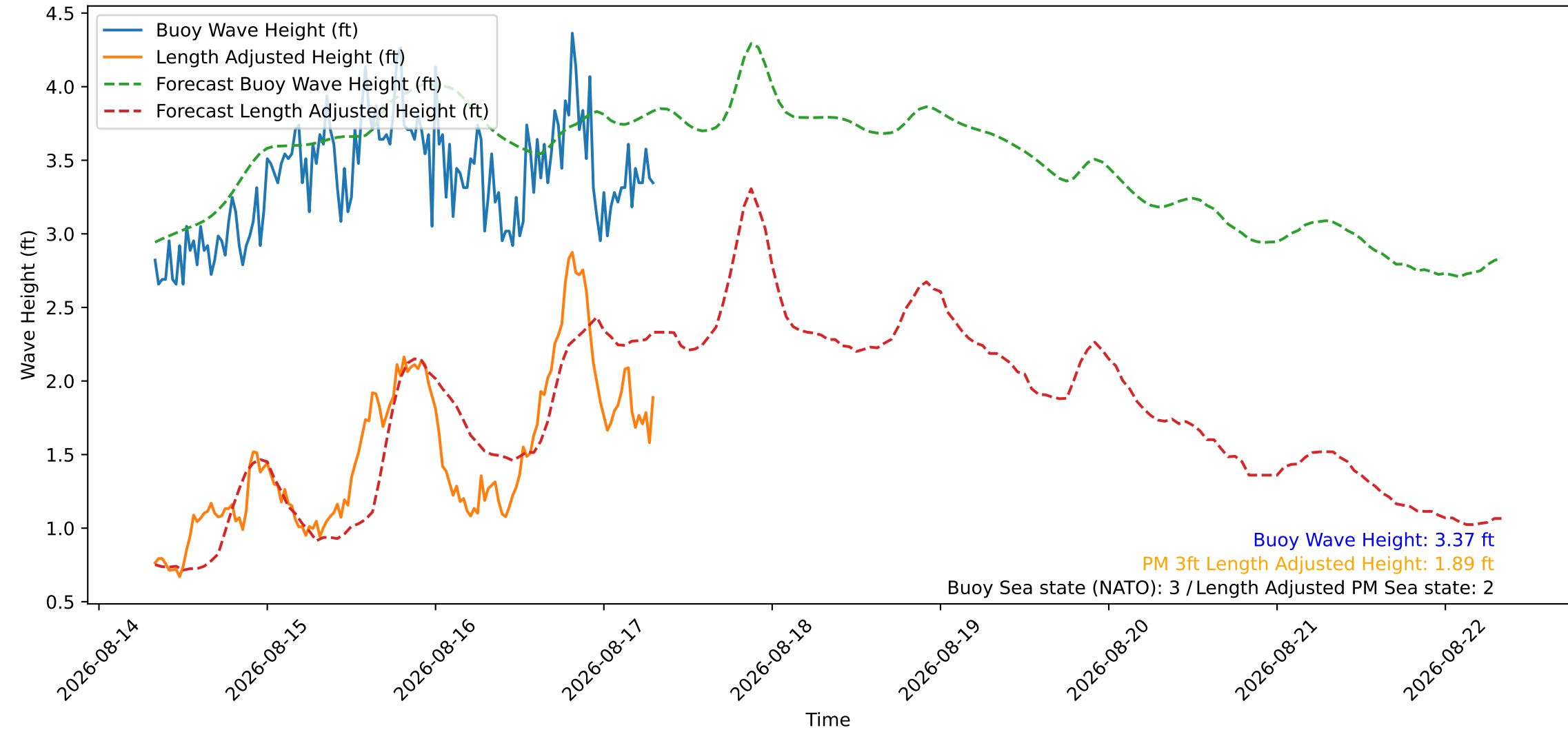
Wave Heights over Time for Green Beach at 2026-08-17 07:51:11
