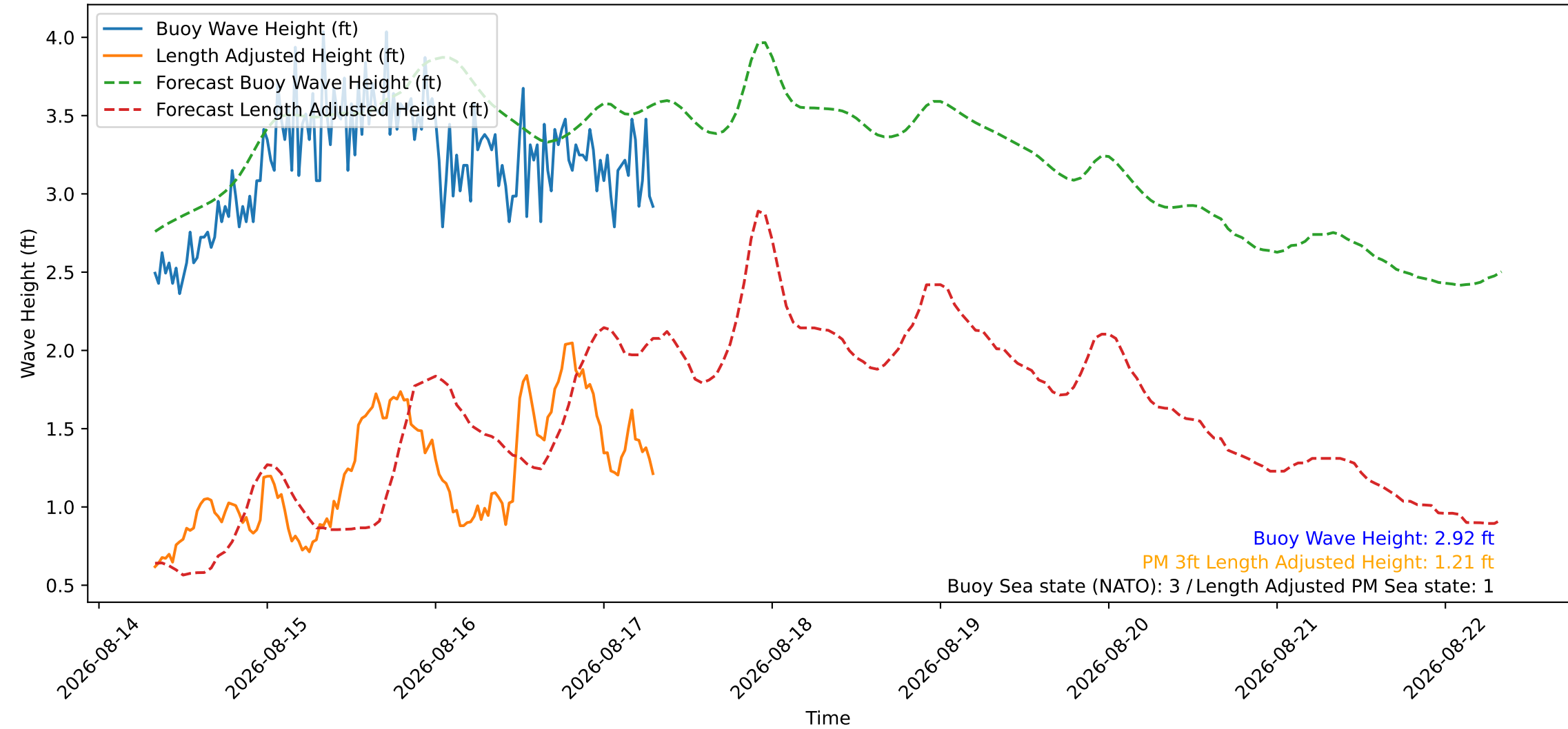
Wave Heights over Time for Red Beach at 2026-08-17 07:50:47
