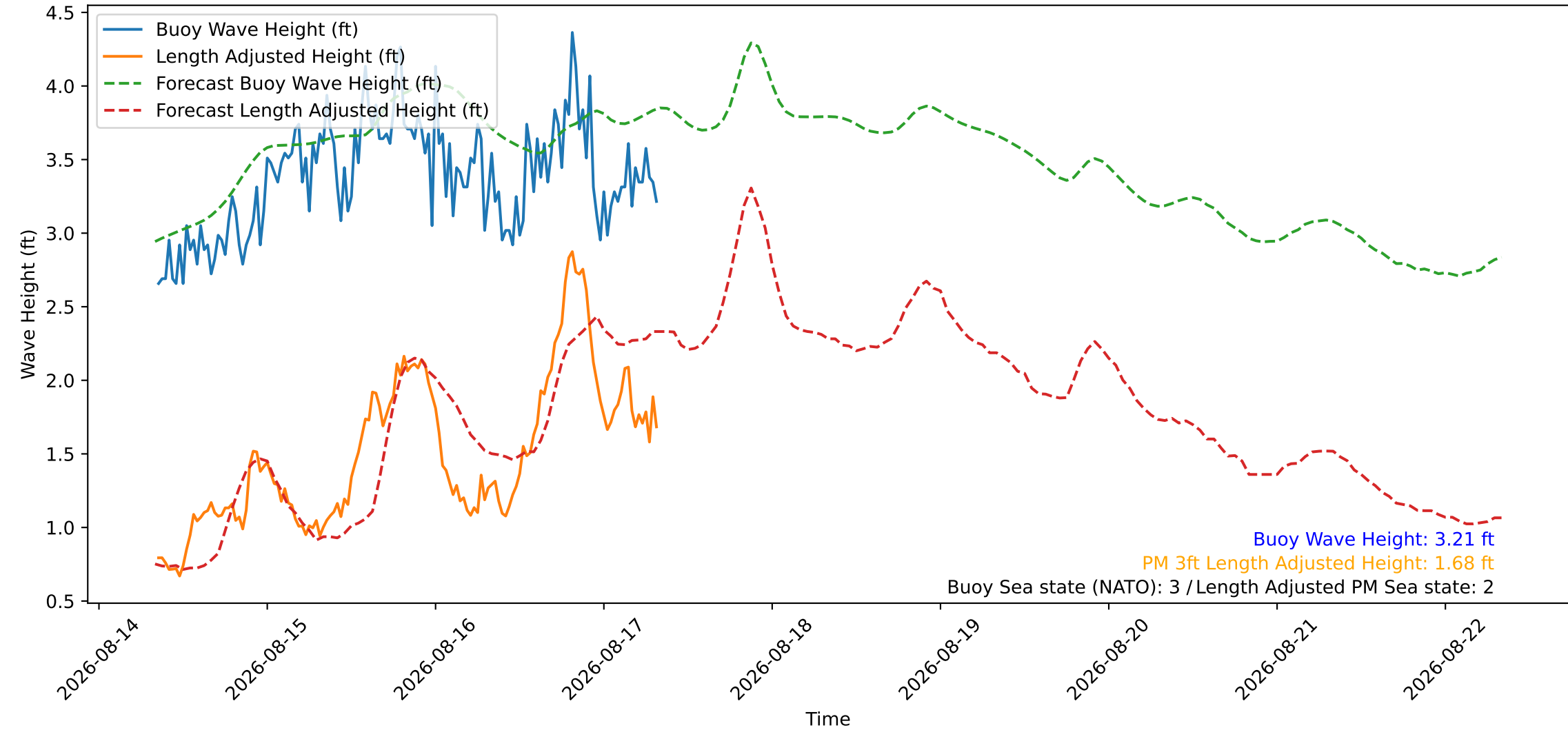
Wave Heights over Time for Green Beach at 2026-08-17 08:11:09
