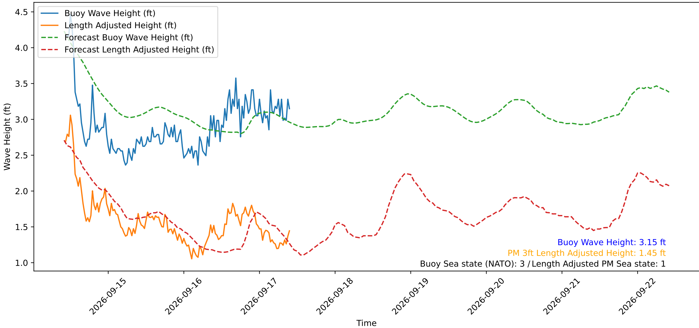
Wave Heights over Time for Oceanside Harbor at 2026-09-17 10:20:29
