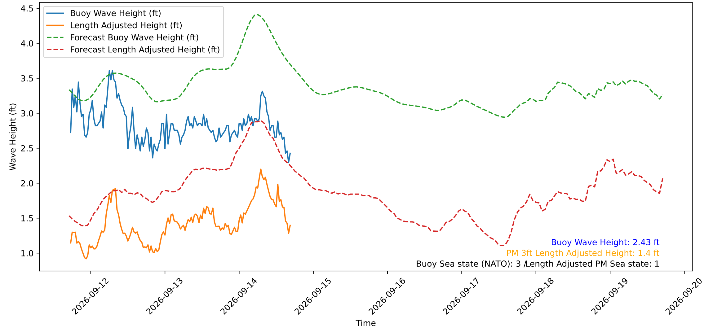
Wave Heights over Time for Green Beach at 2026-09-14 17:21:14
