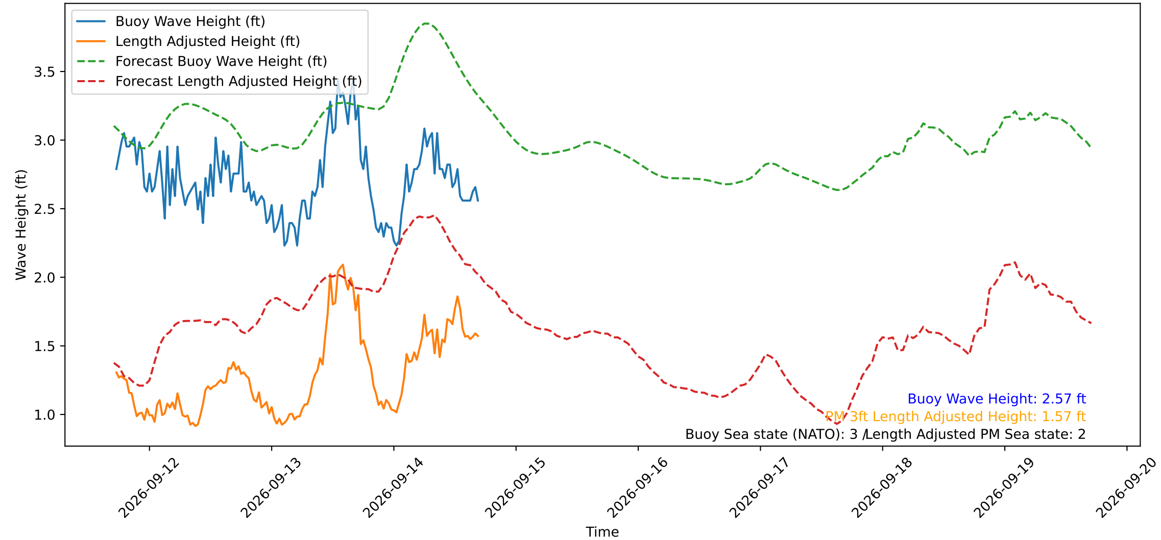
Wave Heights over Time for Red Beach at 2026-09-14 17:20:50
