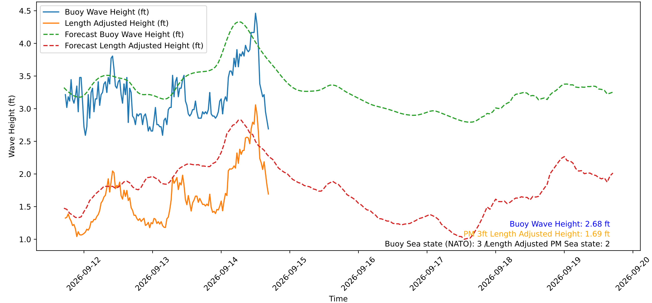
Wave Heights over Time for Oceanside Harbor at 2026-09-14 17:20:29
