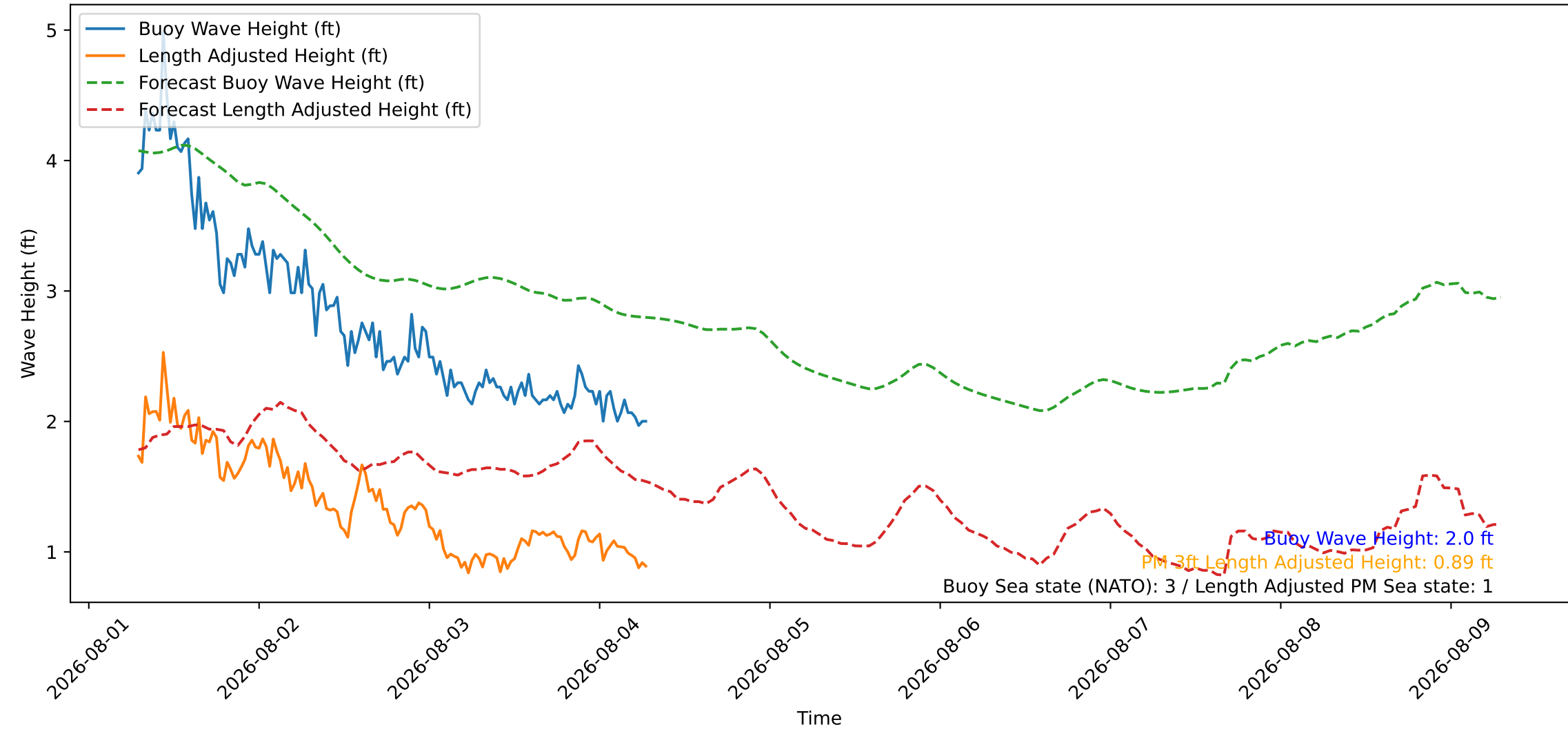
Wave Heights over Time for Green Beach at 2026-08-04 07:11:08
