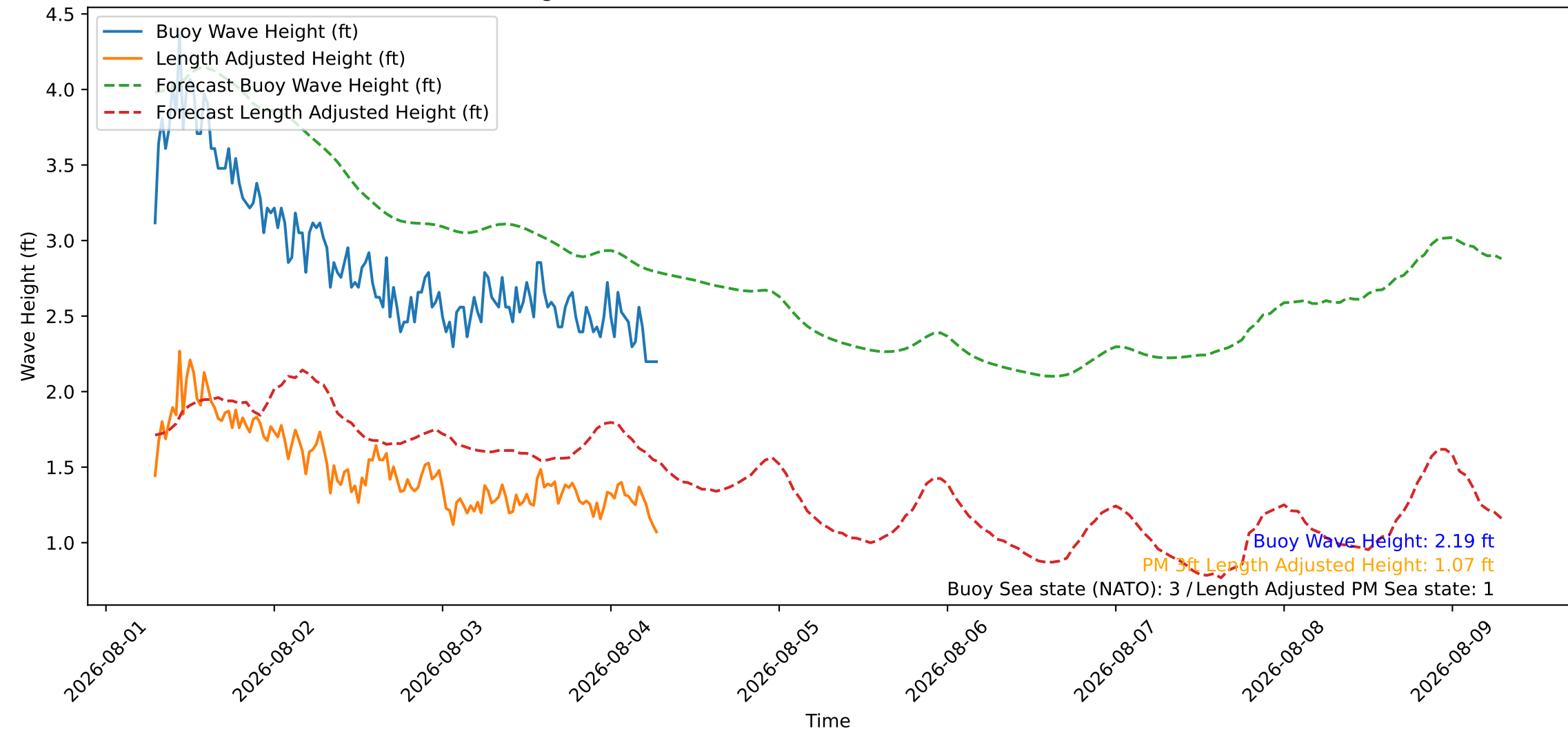
Wave Heights over Time for Oceanside Harbor at 2026-08-04 07:10:26
