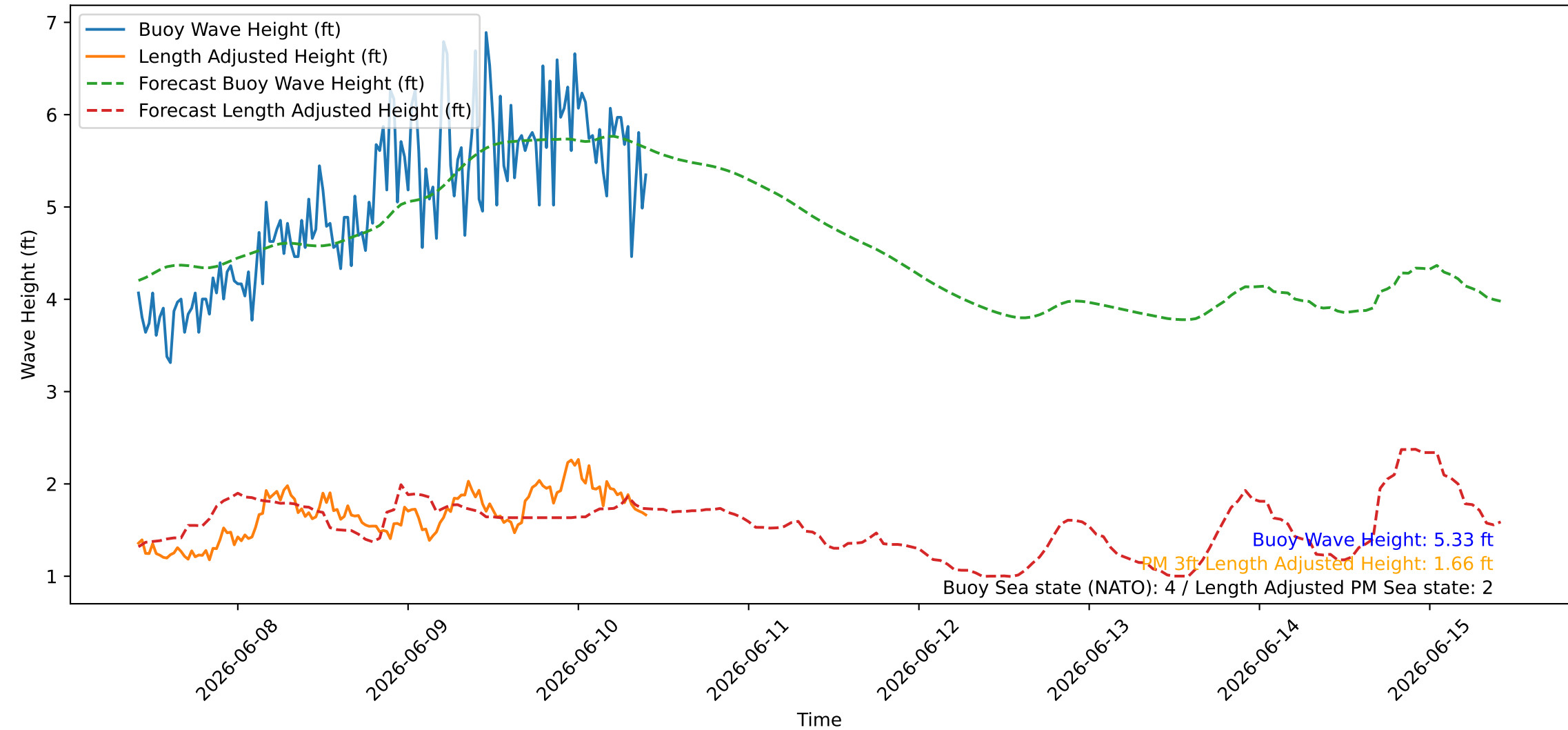
Wave Heights over Time for Green Beach at 2026-06-10 10:11:09
