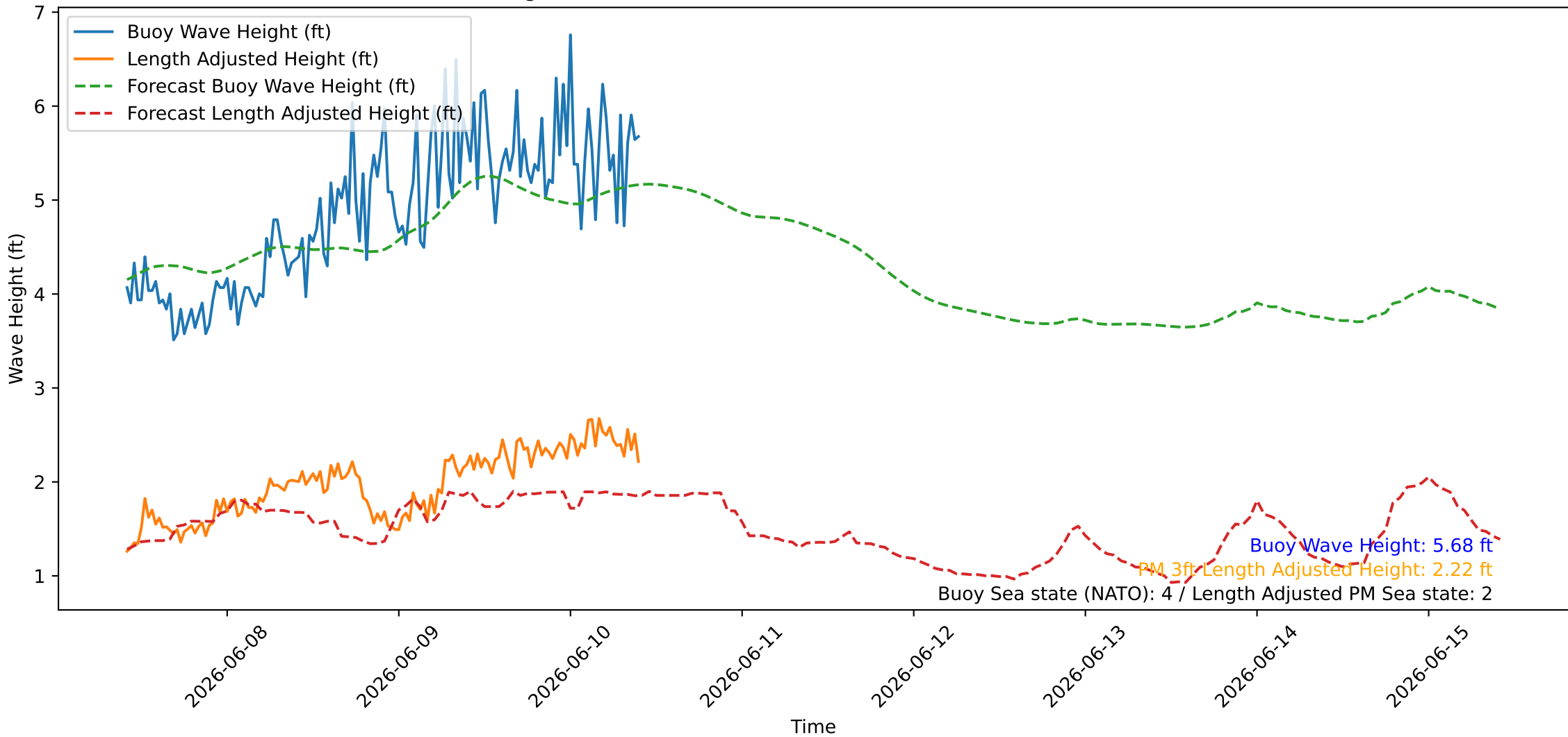
Wave Heights over Time for Oceanside Harbor at 2026-06-10 10:10:26
