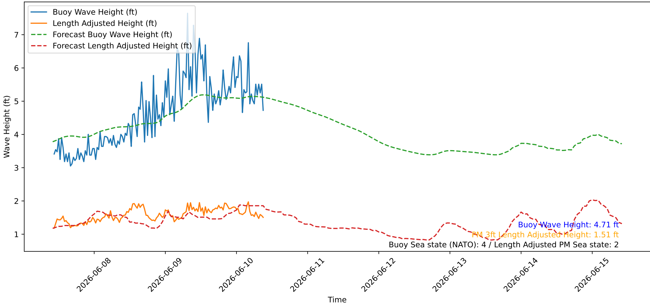
Wave Heights over Time for Red Beach at 2026-06-10 10:10:46
