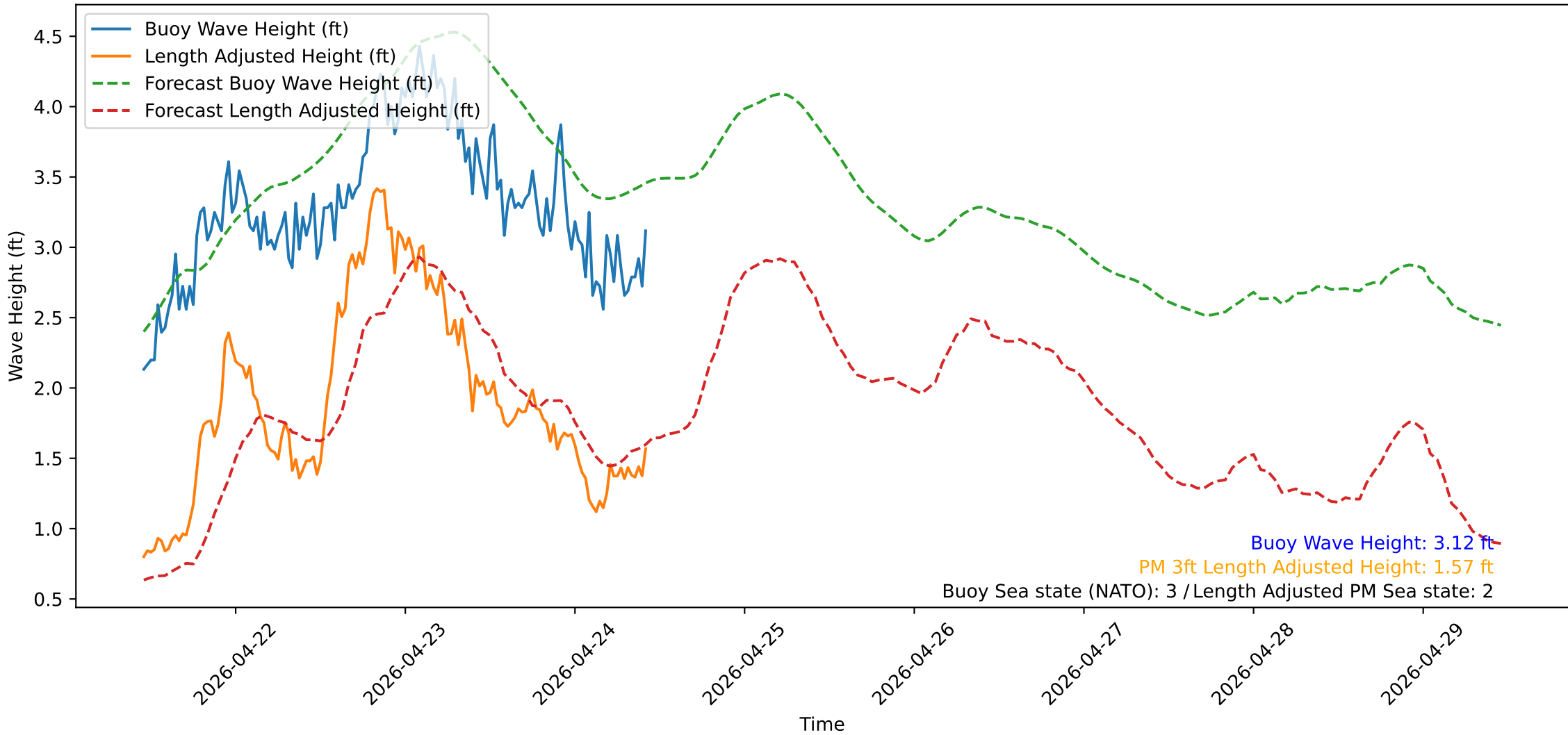
Wave Heights over Time for Oceanside Harbor at 2026-04-24 11:00:30
