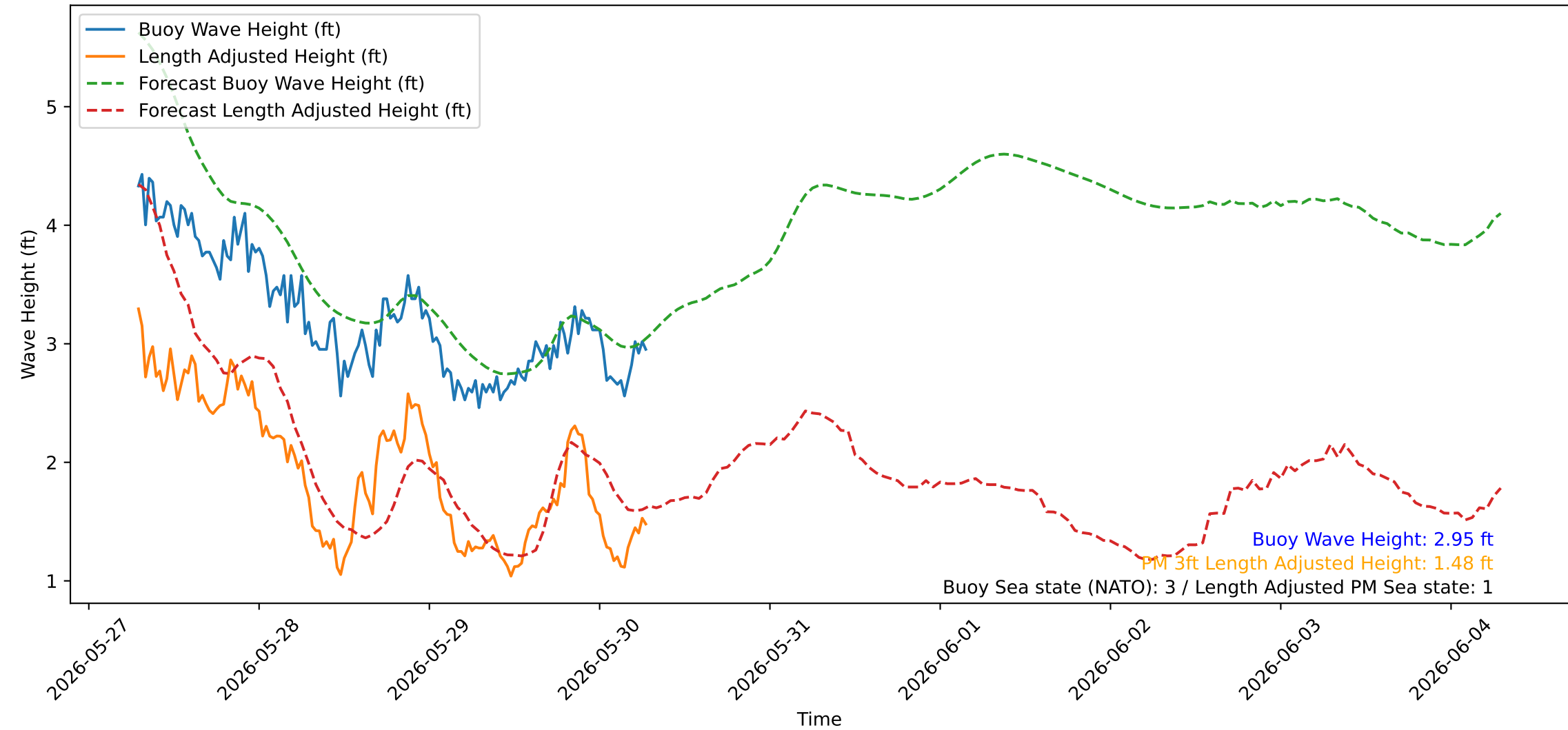
Wave Heights over Time for Green Beach at 2026-05-30 07:11:05
