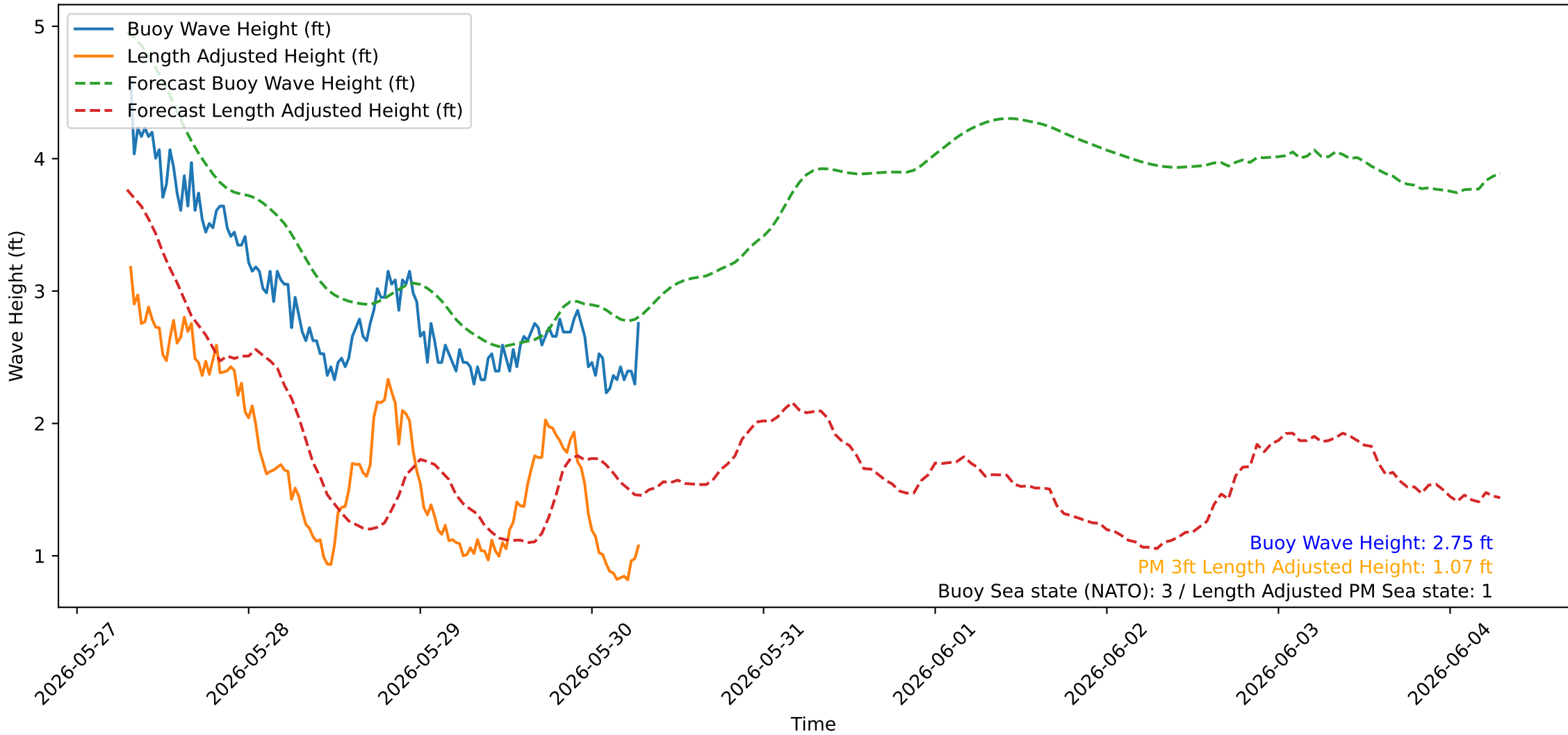
Wave Heights over Time for Red Beach at 2026-05-30 07:10:43
