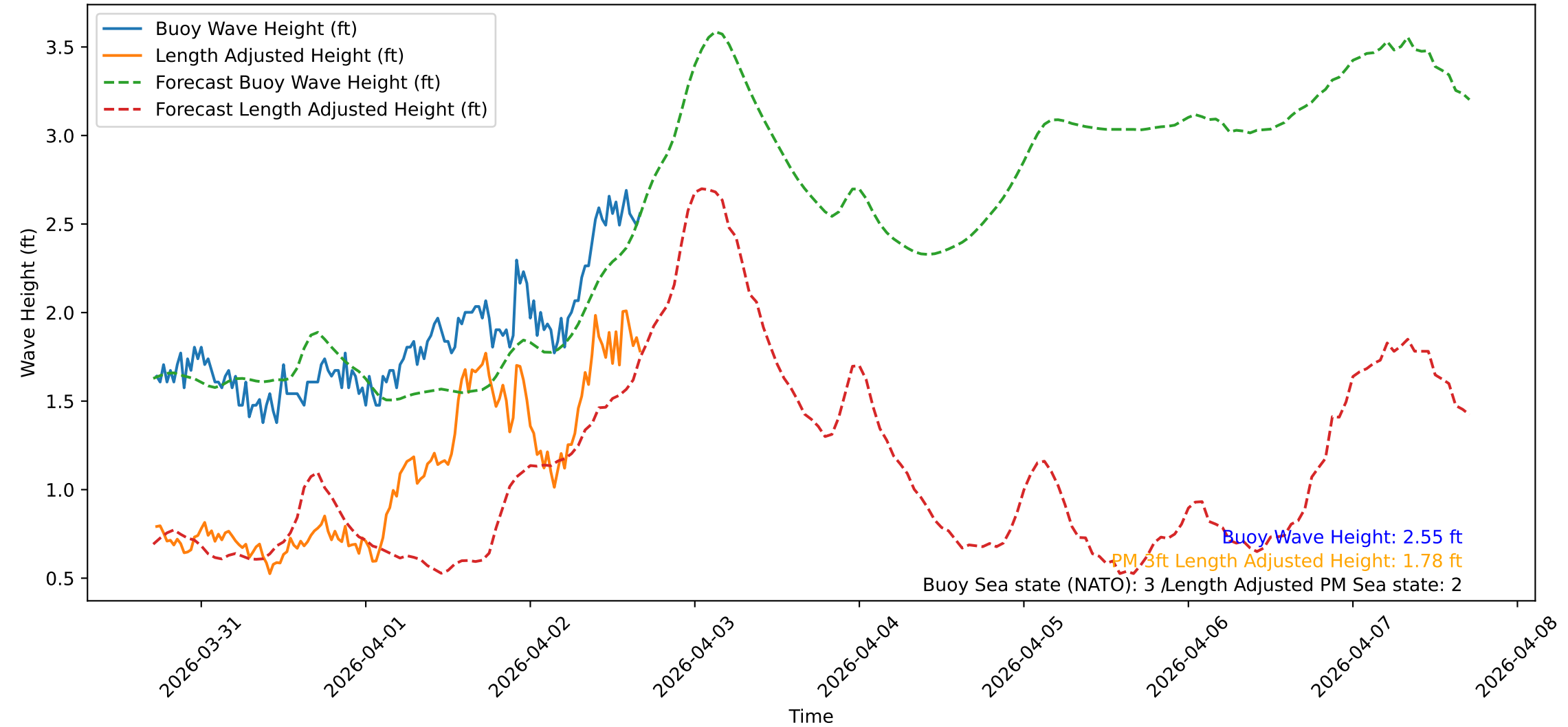
Wave Heights over Time for Red Beach at 2026-04-02 17:00:47
