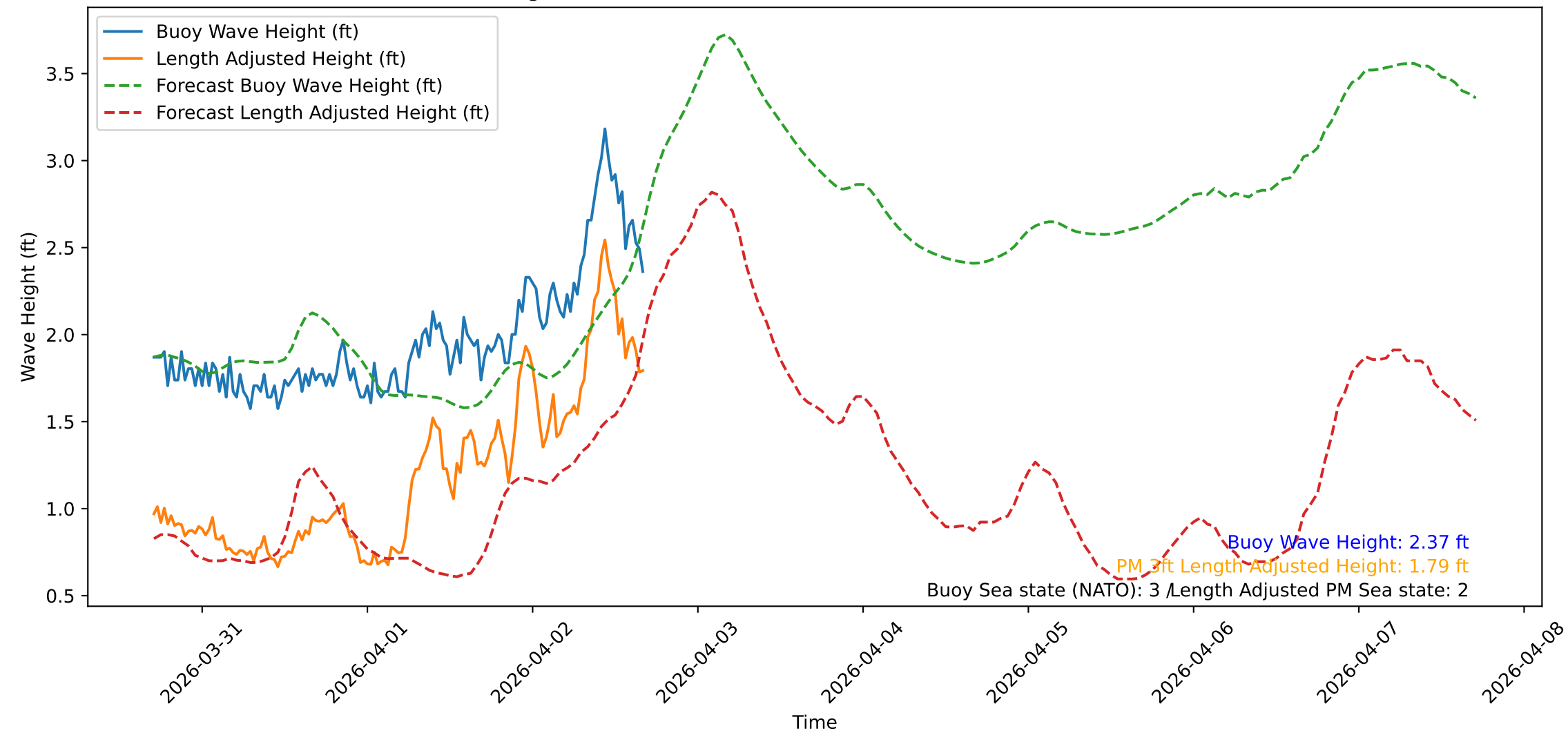
Wave Heights over Time for Oceanside Harbor at 2026-04-02 17:00:31
