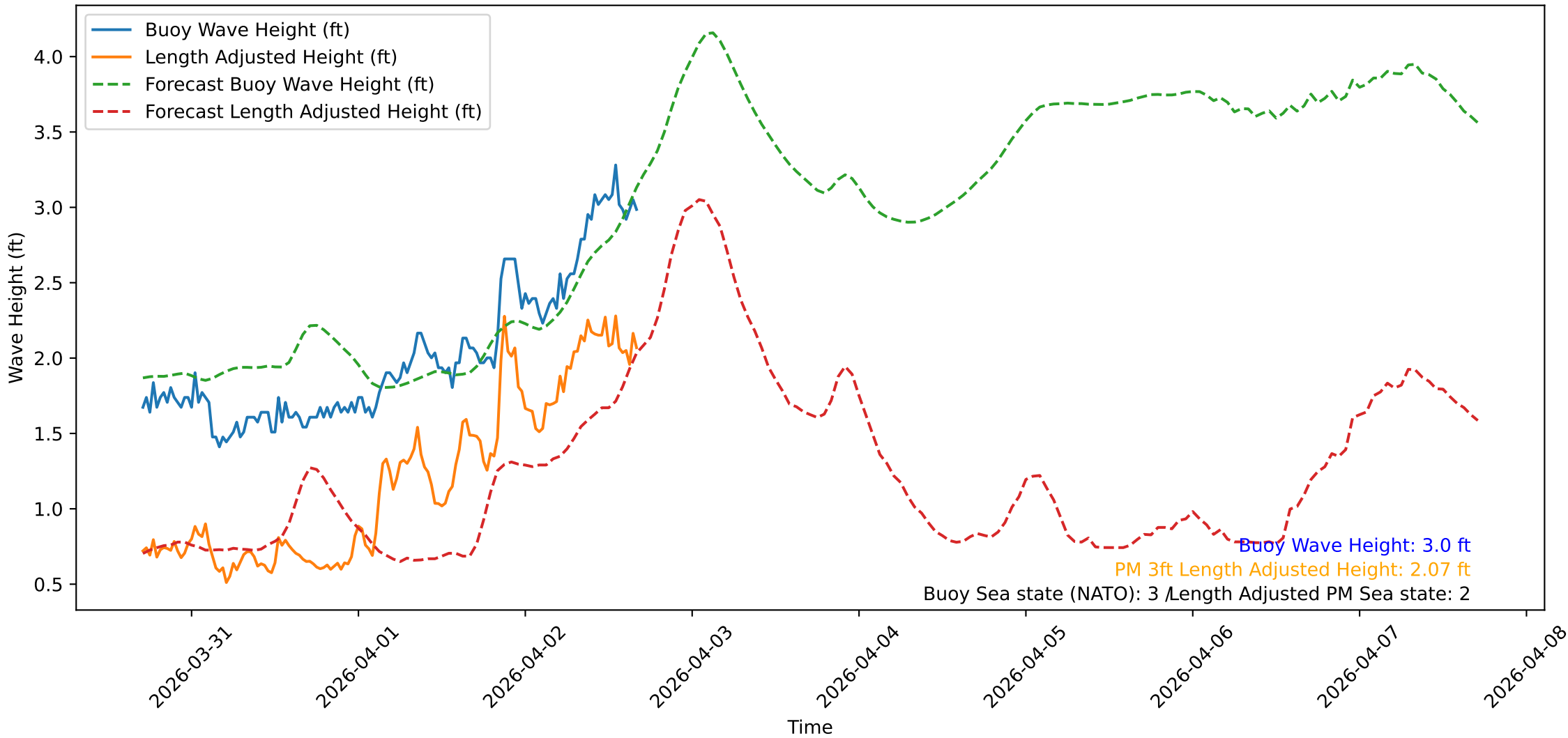
Wave Heights over Time for Green Beach at 2026-04-02 17:01:09
