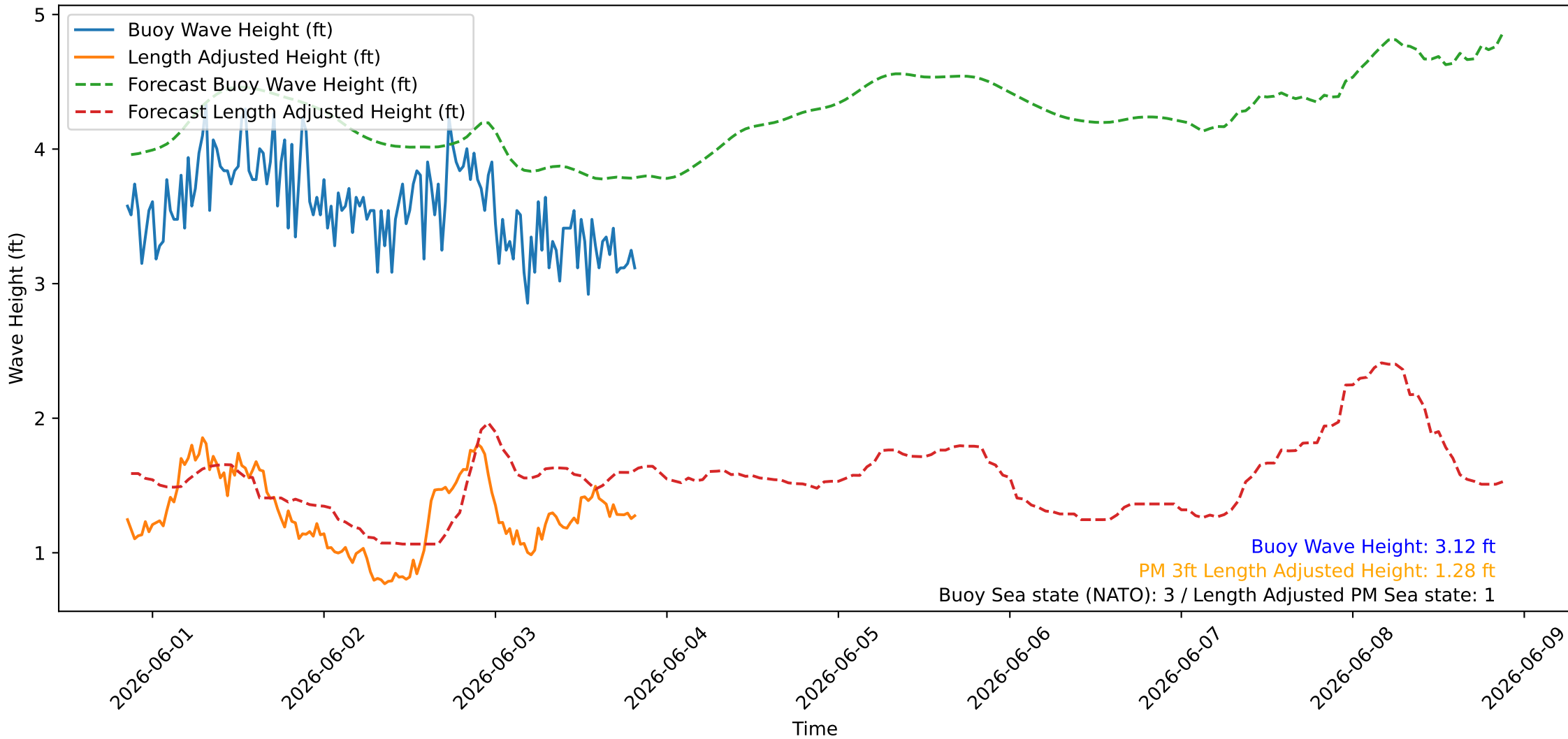
Wave Heights over Time for Green Beach at 2026-06-03 20:31:09
