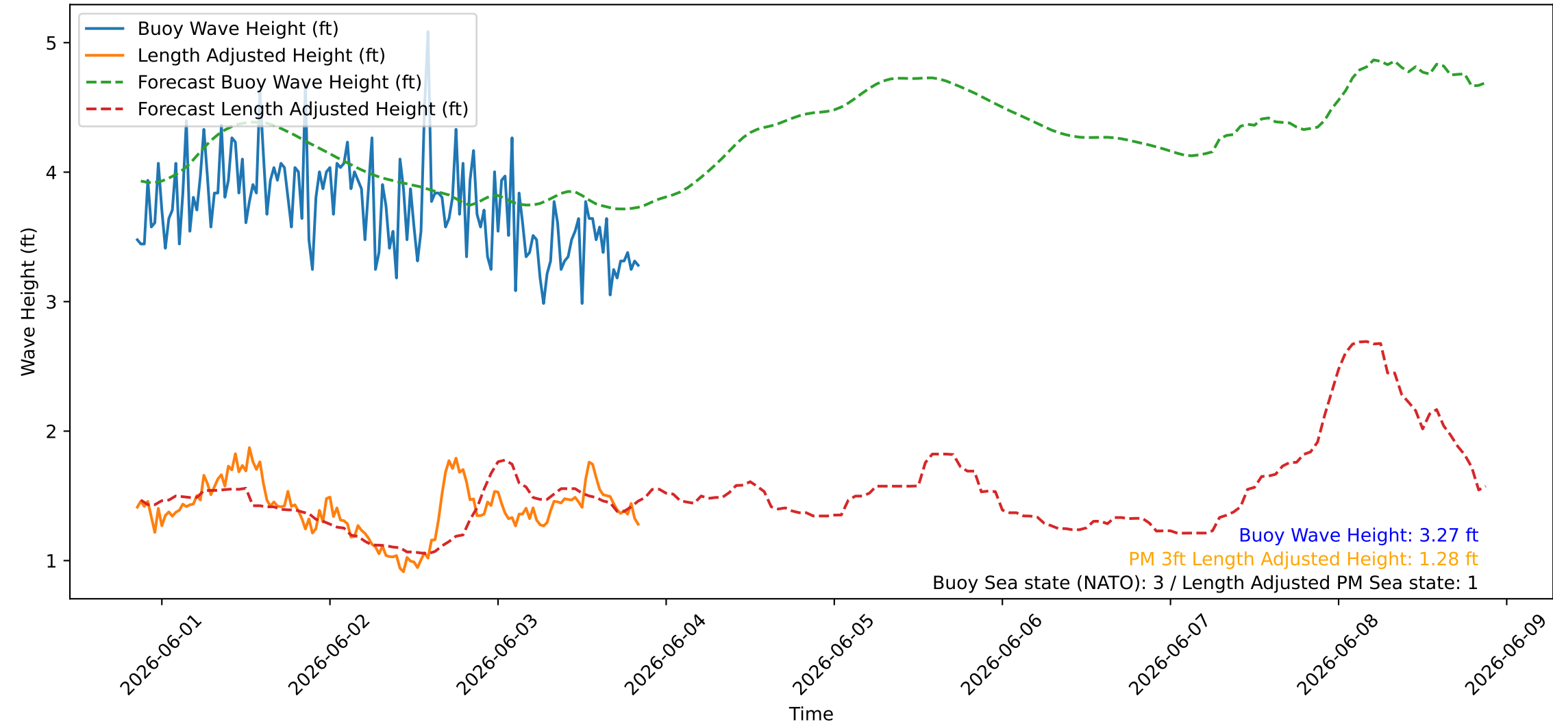
Wave Heights over Time for Oceanside Harbor at 2026-06-03 20:30:26
