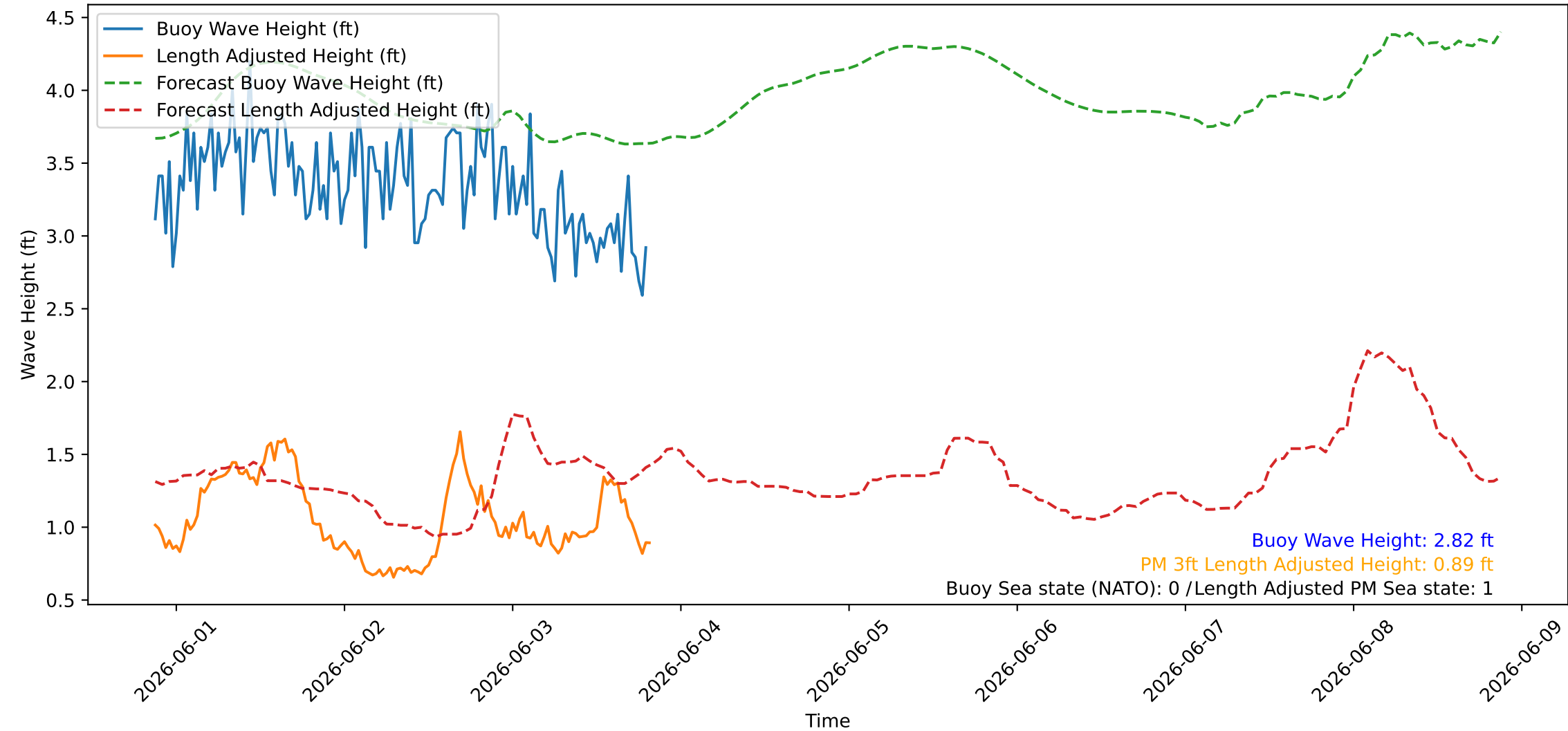
Wave Heights over Time for Red Beach at 2026-06-03 20:30:46
