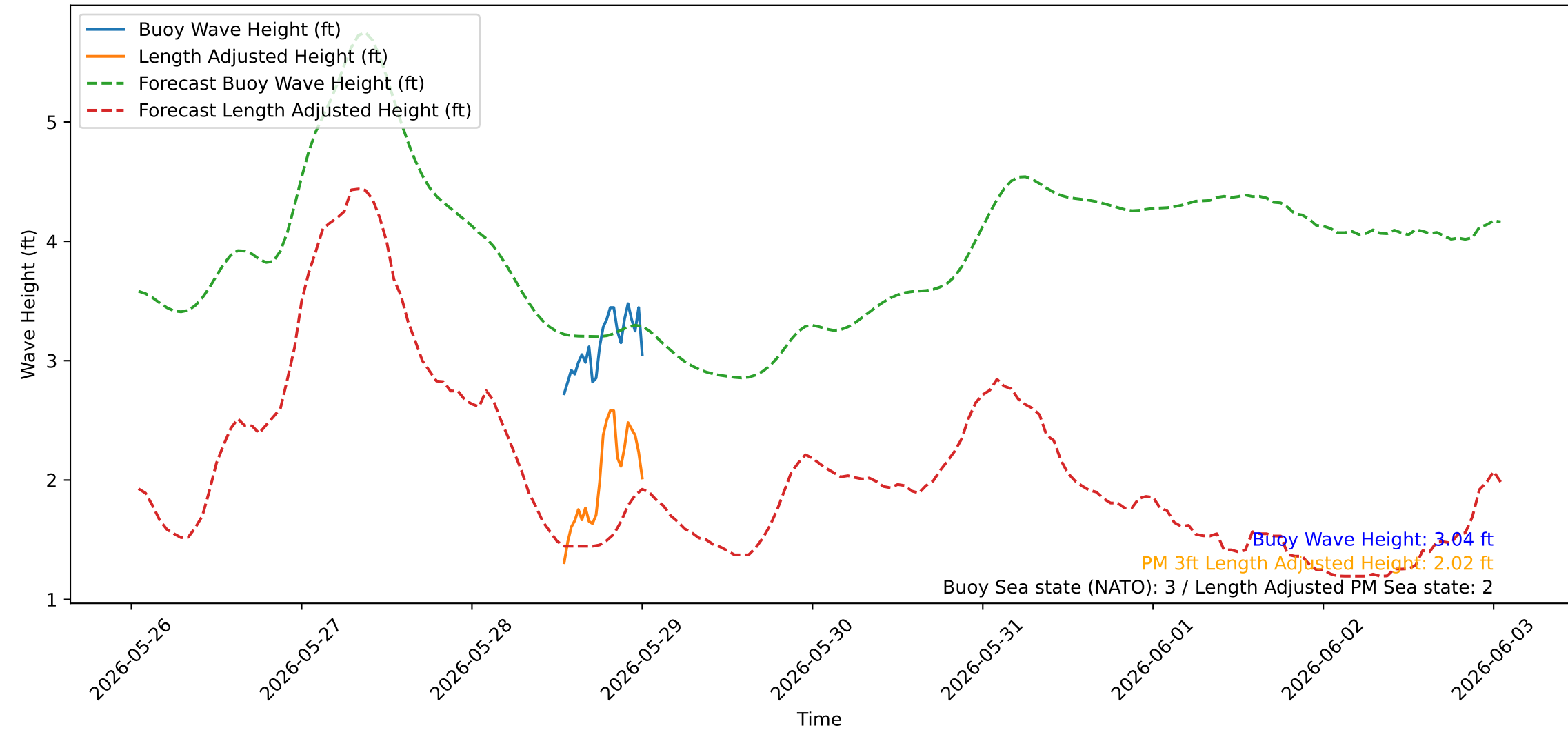
Wave Heights over Time for Oceanside Harbor at 2026-05-29 01:00:20
