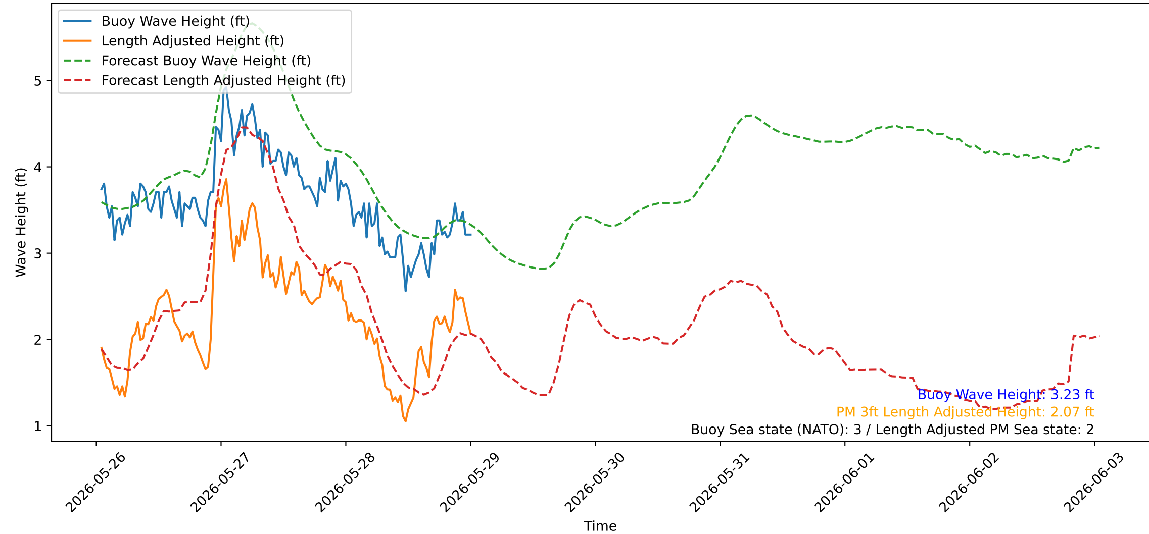
Wave Heights over Time for Green Beach at 2026-05-29 01:01:01
