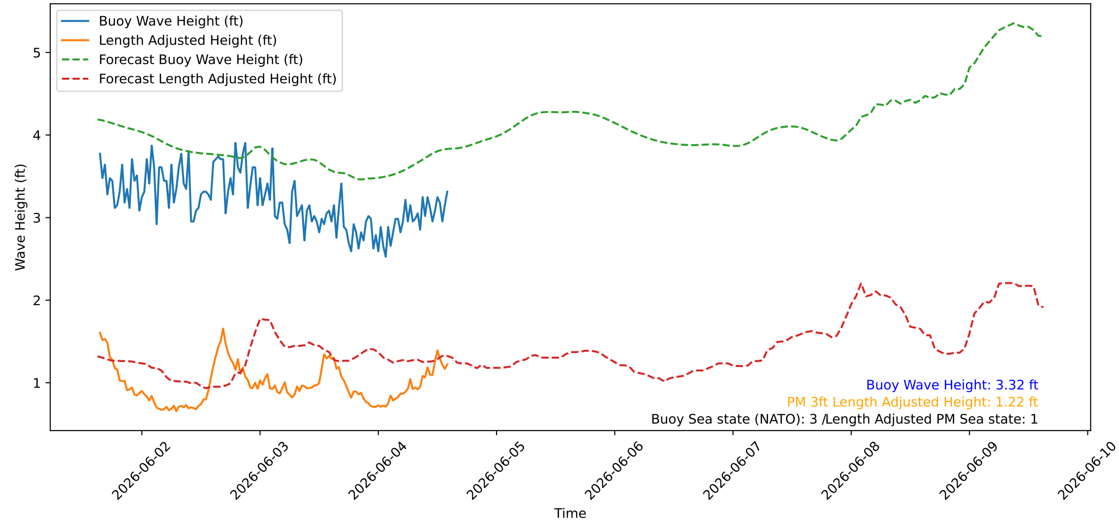
Wave Heights over Time for Red Beach at 2026-06-04 15:00:45
