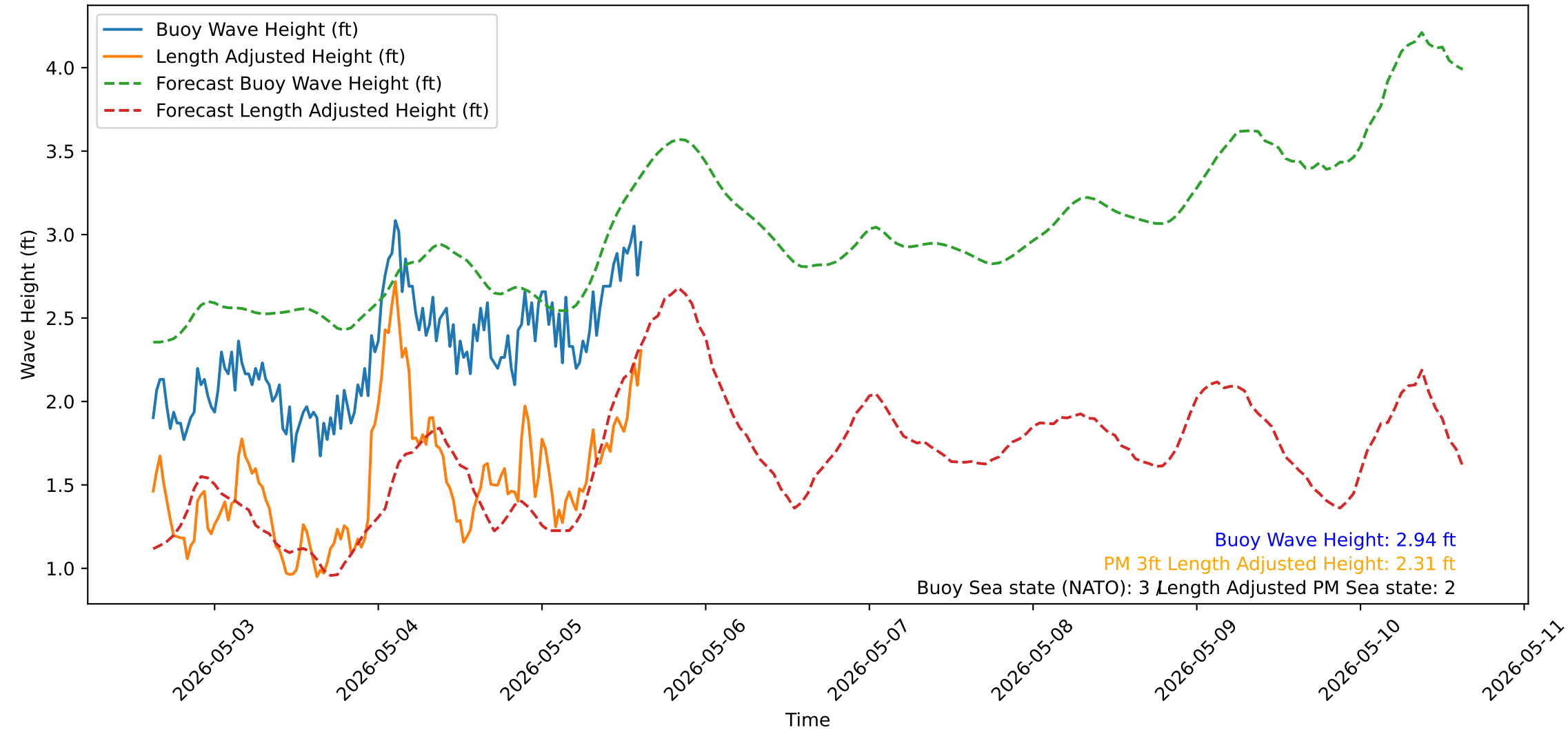
Wave Heights over Time for Oceanside Harbor at 2026-05-05 15:00:32
