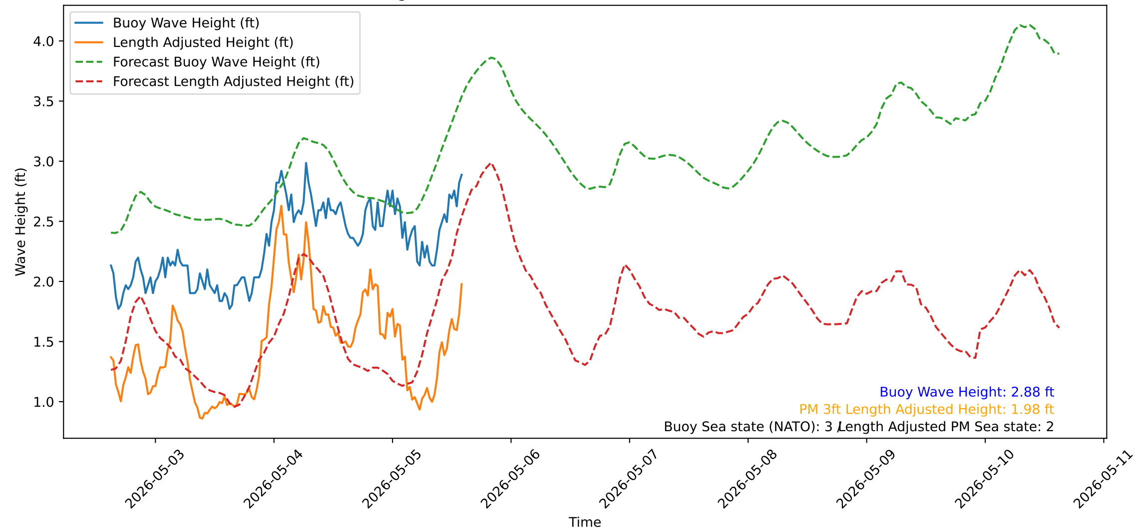
Wave Heights over Time for Green Beach at 2026-05-05 15:01:14
