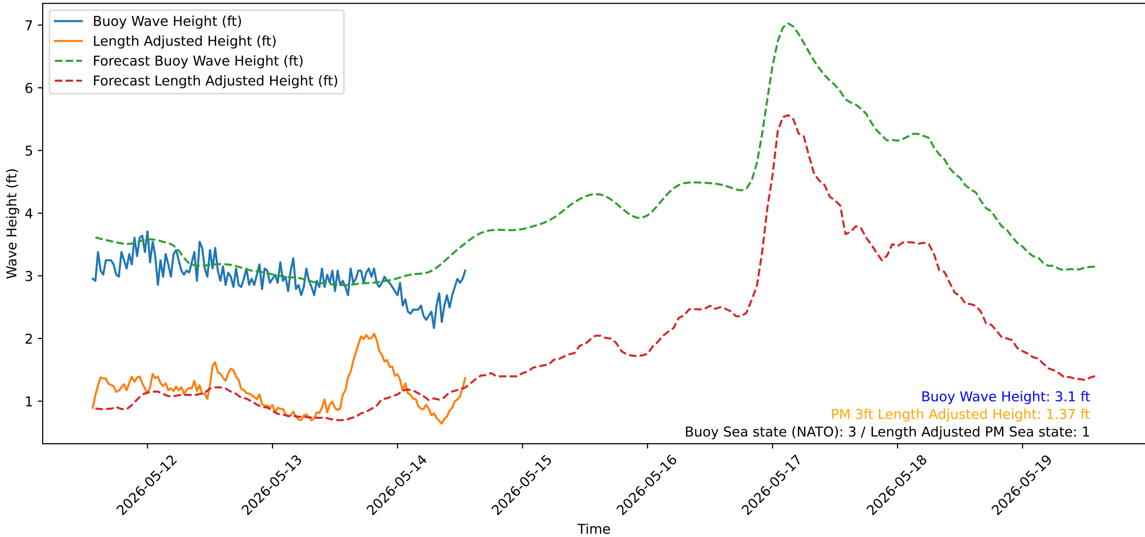
Wave Heights over Time for Oceanside Harbor at 2026-05-14 13:30:32
