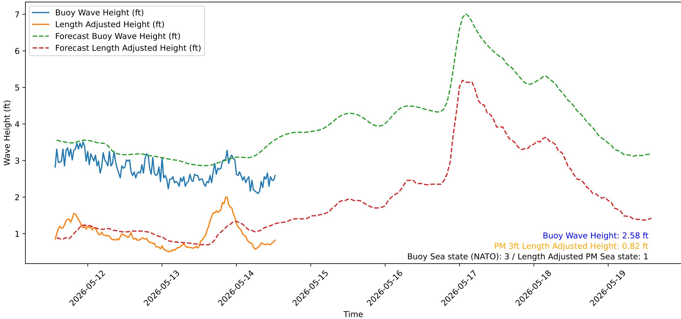
Wave Heights over Time for Green Beach at 2026-05-14 13:31:14
