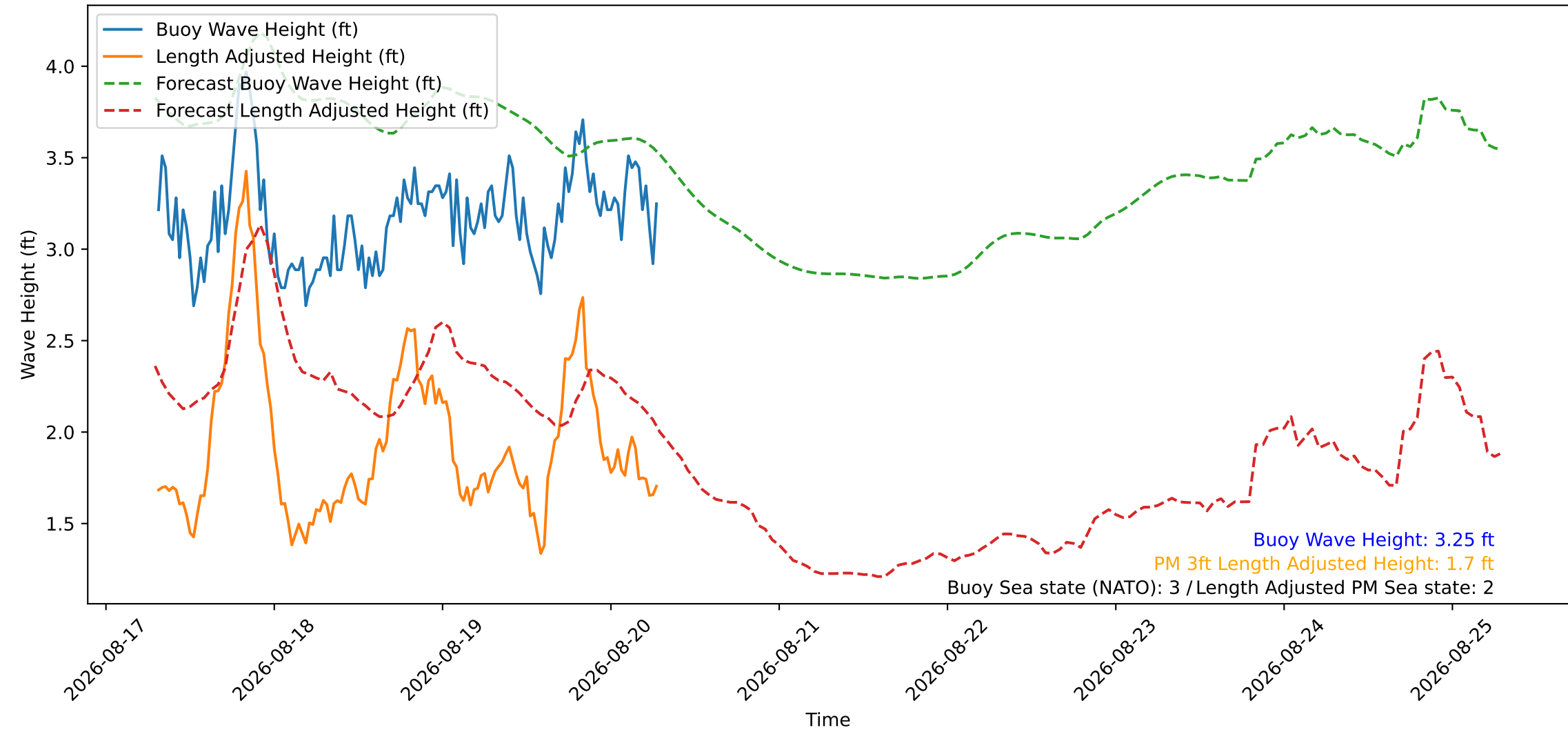
Wave Heights over Time for Green Beach at 2026-08-20 07:11:09
