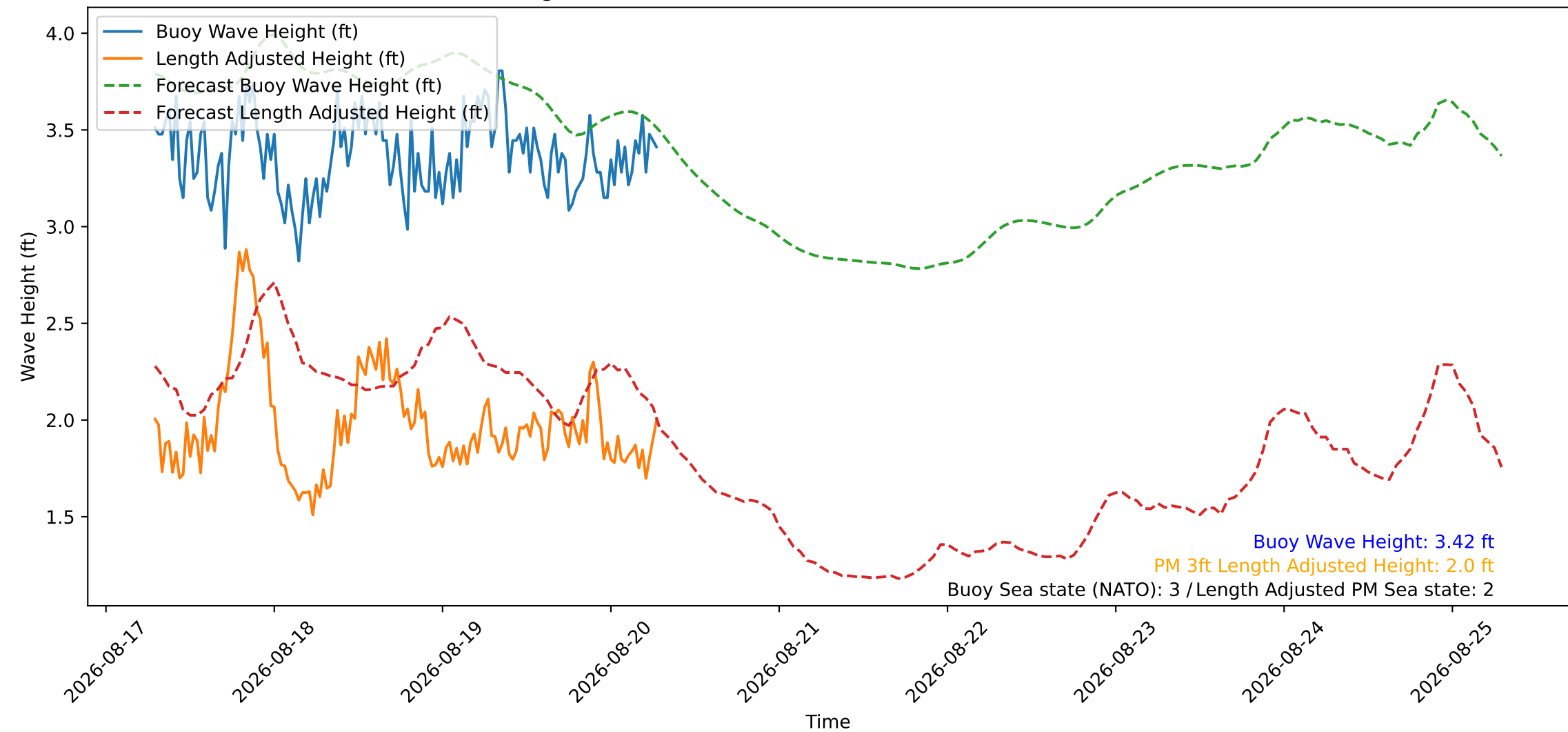
Wave Heights over Time for Oceanside Harbor at 2026-08-20 07:10:26
